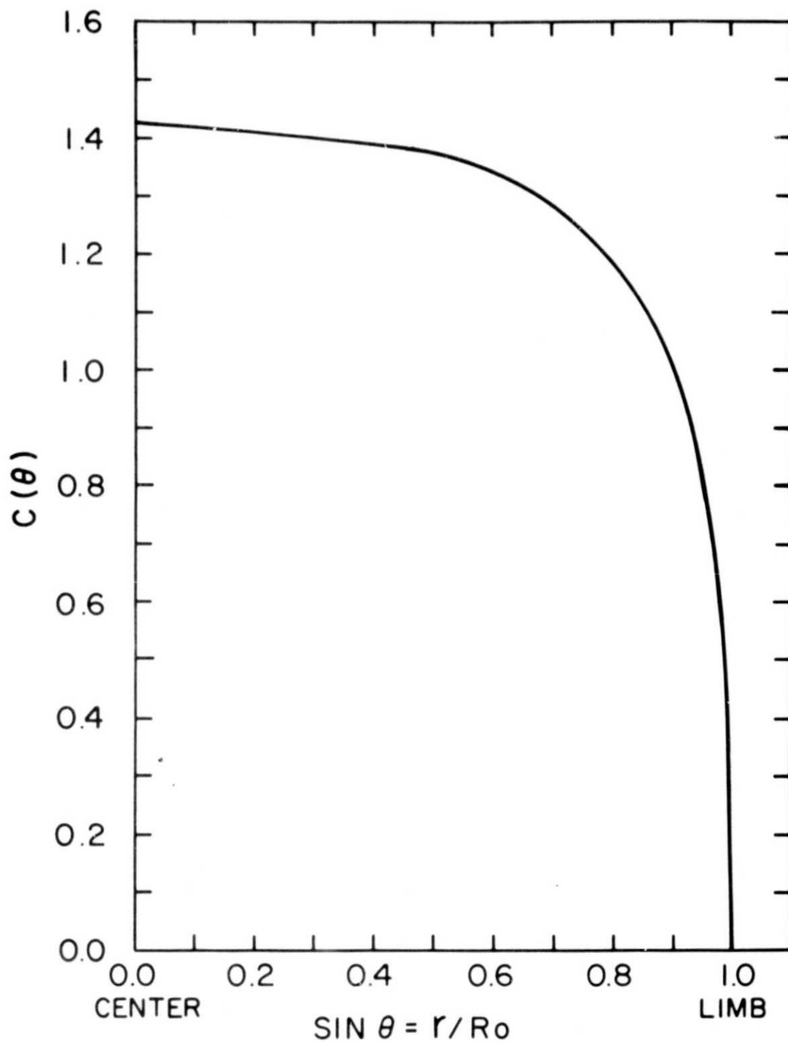
Figure 1. The function C(\theta) , describing the influence of the flare position on the albedo. R_0 is the radius of the sun and r is the distance of the flare source from the center of the solar disk.
