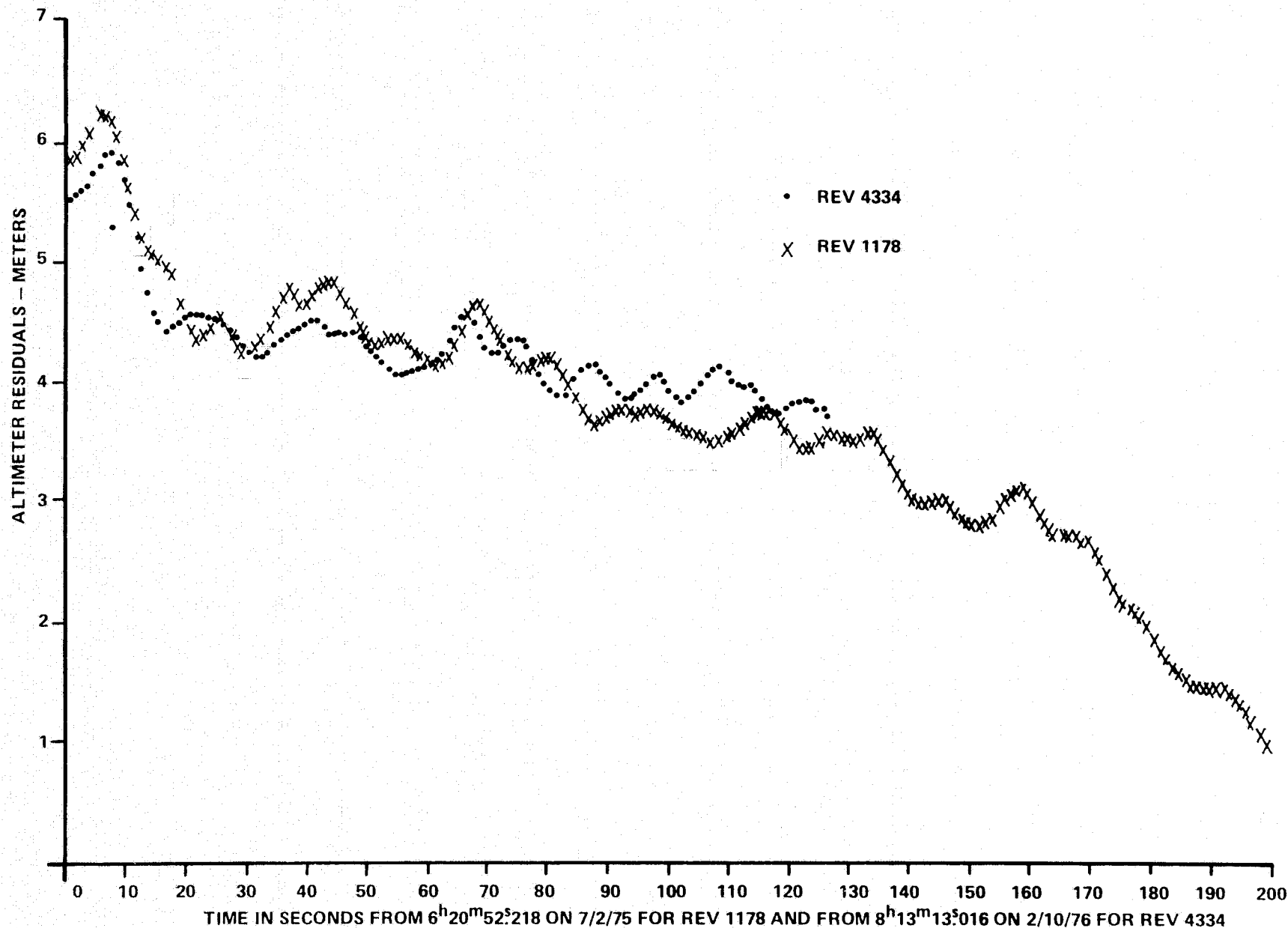
FIGURE 10. ALTIMETER RESIDUALS FOR OVERLAPPING TRACKS ON REVS 1178 AND 4334.
