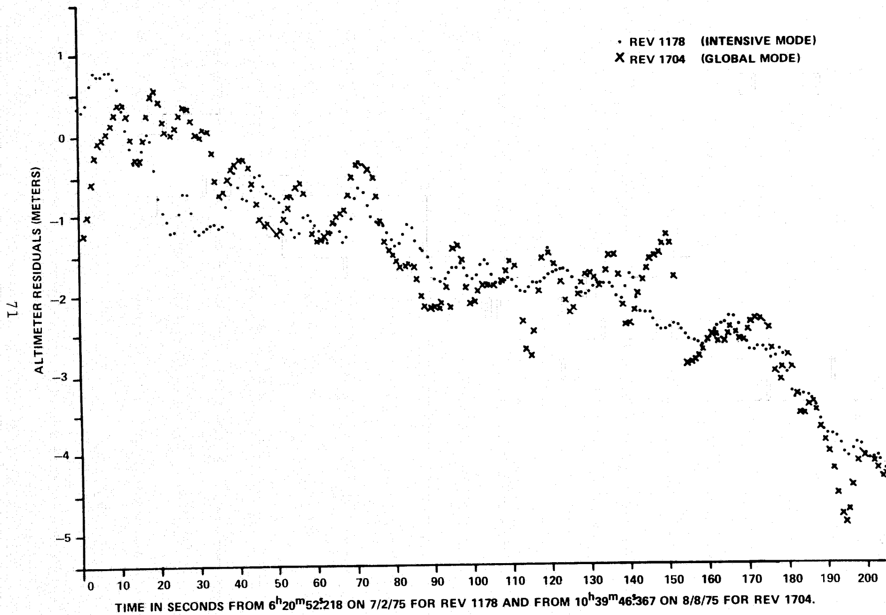
FIGURE 23. ALTIMETER RESIDUALS FOR OVERLAPPING TRACKS ON REVS 1178 AND 1704. REV 1704 HAS BEEN SHIFTED DOWN 1.75 m.
