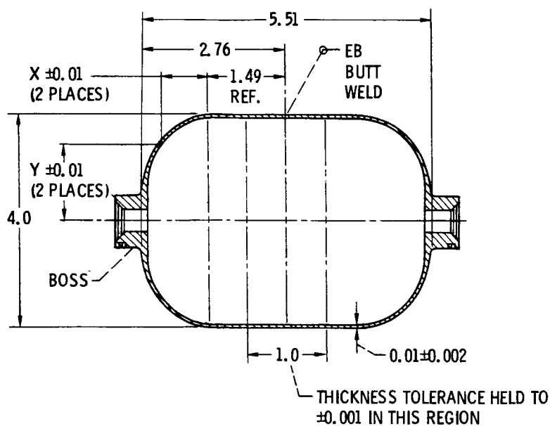
Figure 16. - Titanium (6Al-4V) liner designs.
