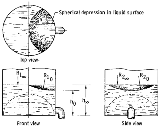
Figure 12. - Approximate surface curvature function ( (h_\infty/b) > 1 ).
