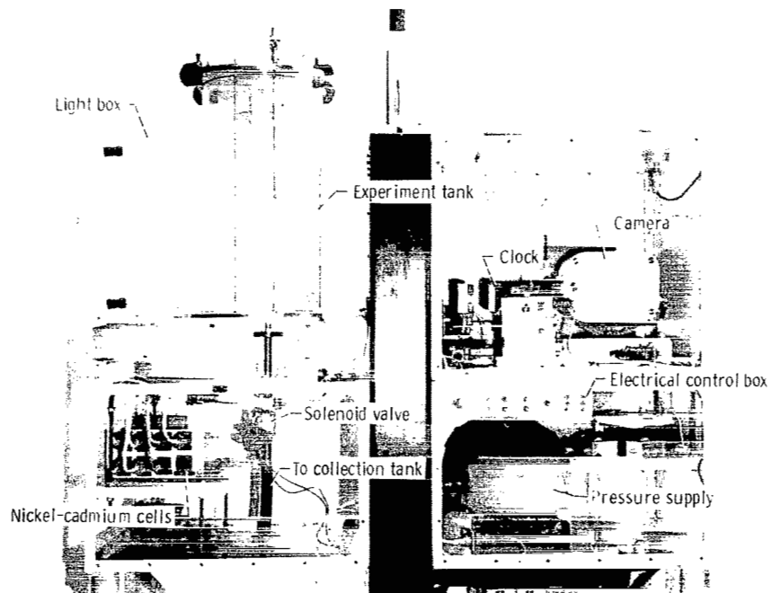
Figure 4. - Experiment package.
