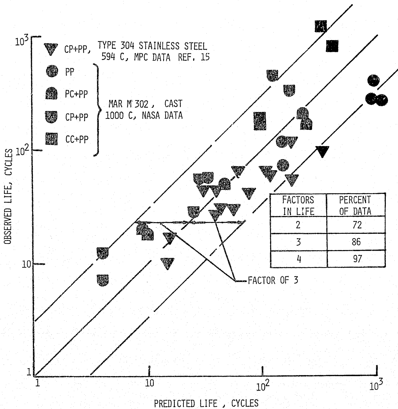
Fig. 2 - Comparison of Observed and Predicted Cyclic Lives for Two Alloys Based on the Ductility - Normalized Strainrange Partitioning Life Relations.
