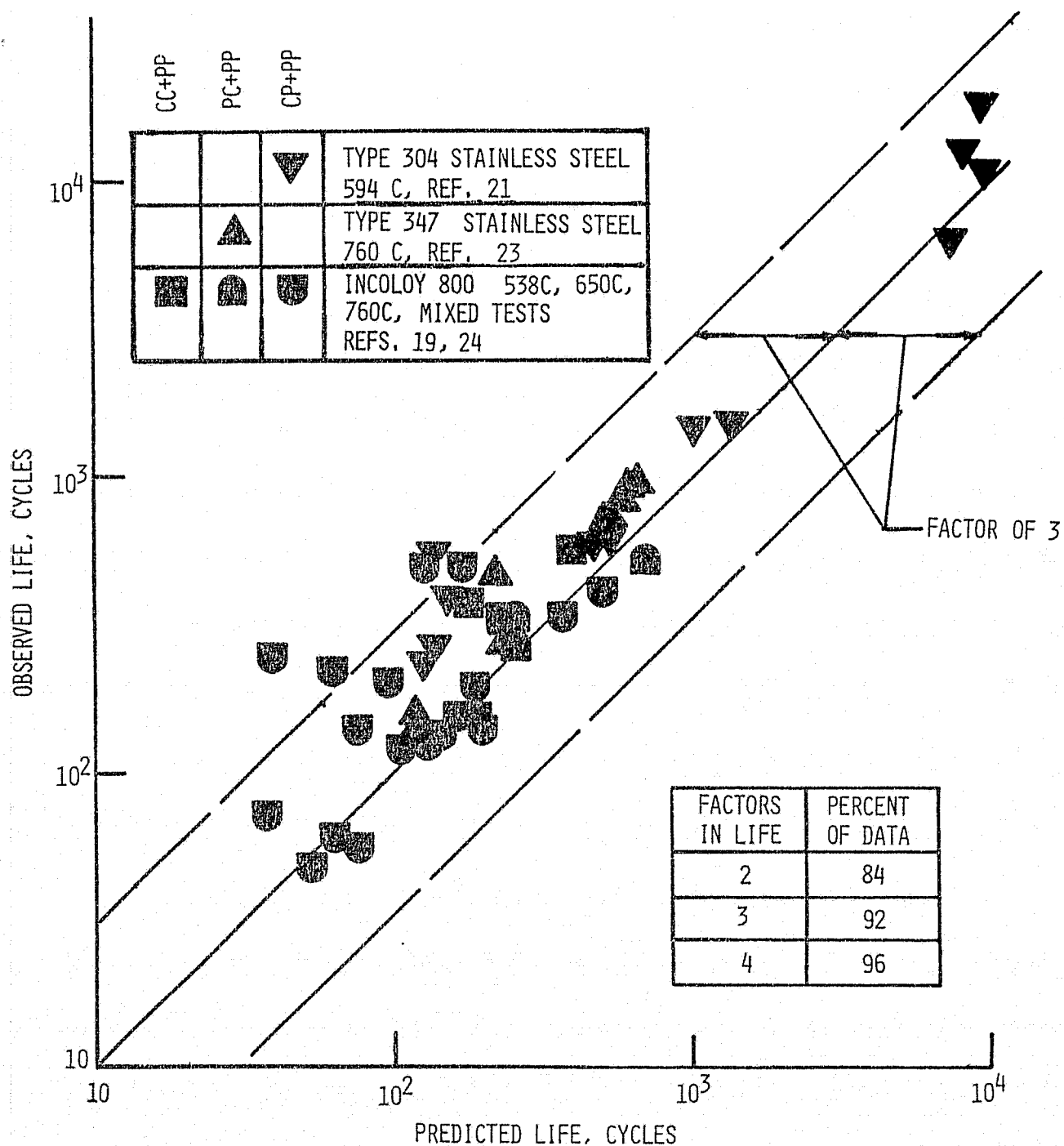
Fig. 4 - Comparison of Observed and Predicted Cyclic Lives for Three Alloys.
