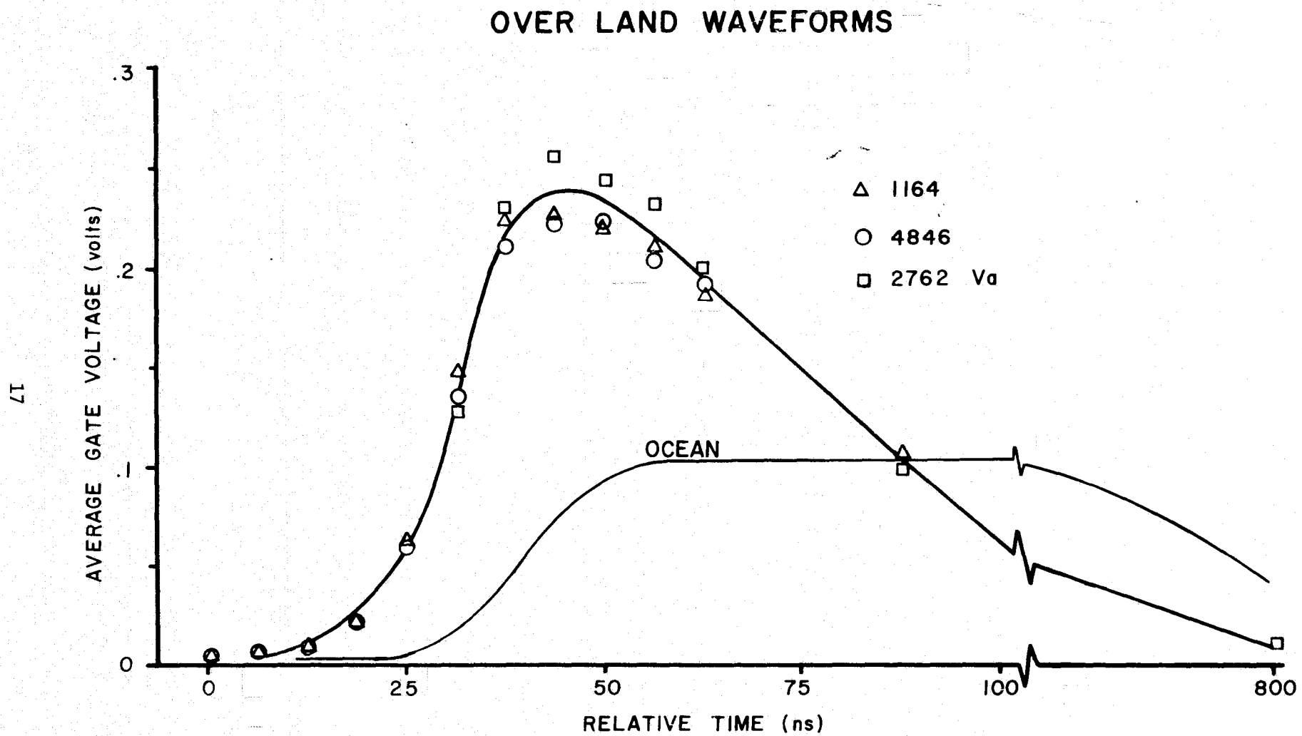
Figure 10. Typical over-land waveforms.
