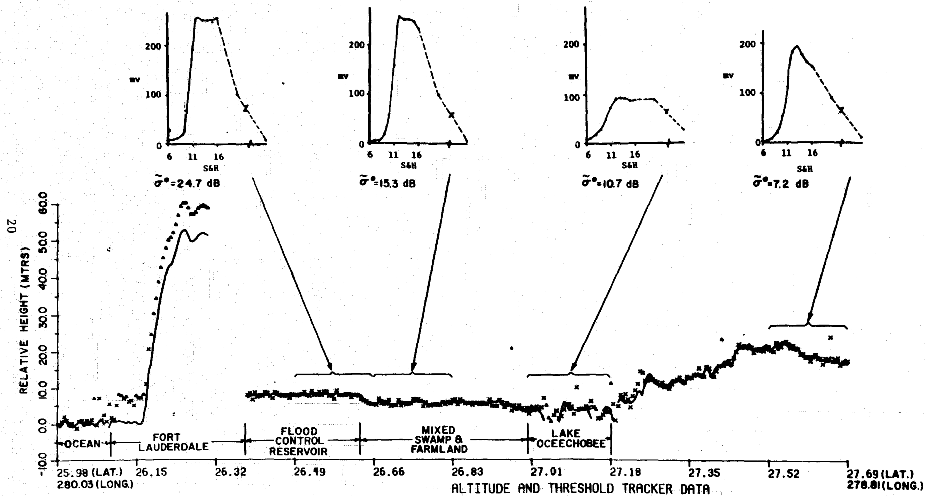
Figure 12. Altimeter and waveform data for a variety of topographic conditions, Orbit 4568.
