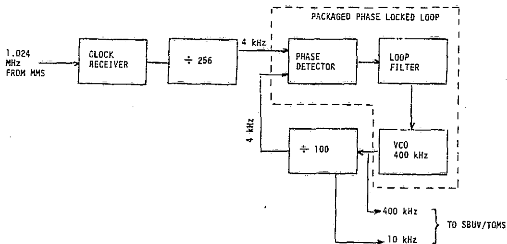
Figure C-2. Phase-Locked Clock
