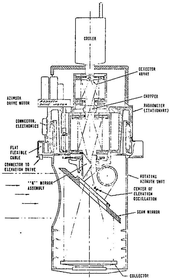
Figure 3. LACATE Instrument
