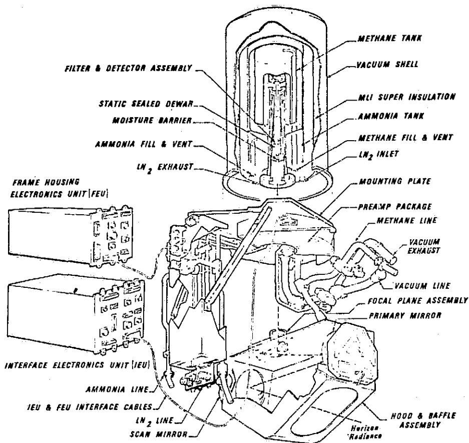
Figure 17. LIMS Sensor
