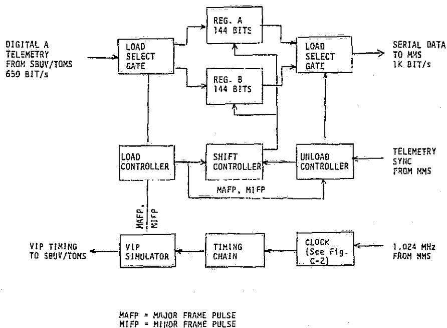
Figure C-3. Block Diagram, Digital Telemetry Translation Logic
