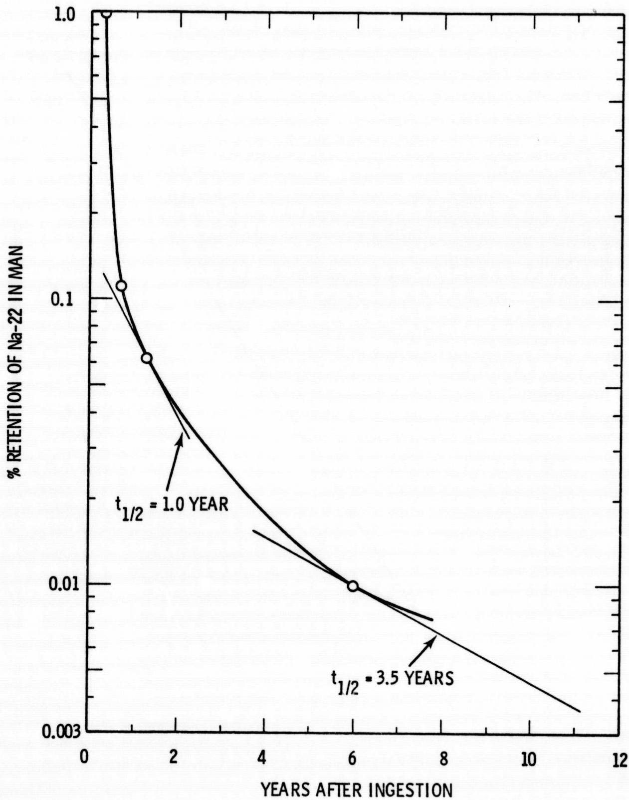
FIGURE 6. Retention of Na-22 in Adult Human Starting 100 Days After Administration of 50 \mu Ci (Data Corrected For Radioactive Decay).
