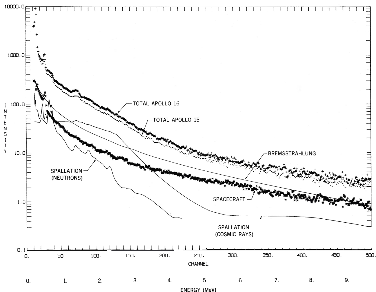
FIG. 1.—The total energy-loss spectra observed at full (7.6 m) boom extension on Apollo 15 and Apollo 16 are compared with the calculated levels of various backgrounds discussed in the text. The latter are shown for the Apollo 16 measurement. The only component to change significantly is the electron bremsstrahlung, which, at the time of Apollo 15 , was approximately half the value shown.
