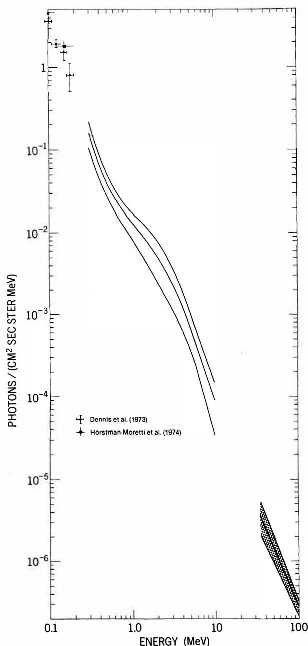
FIG. 4.—The unfolded photon spectrum from the Apollo data is shown by the line within the \pm 1 \sigma error band. Comparison is made with the recent high- and low-energy data. Hatched area, the SAS-2 measurement (Fichtel et al. 1975).
