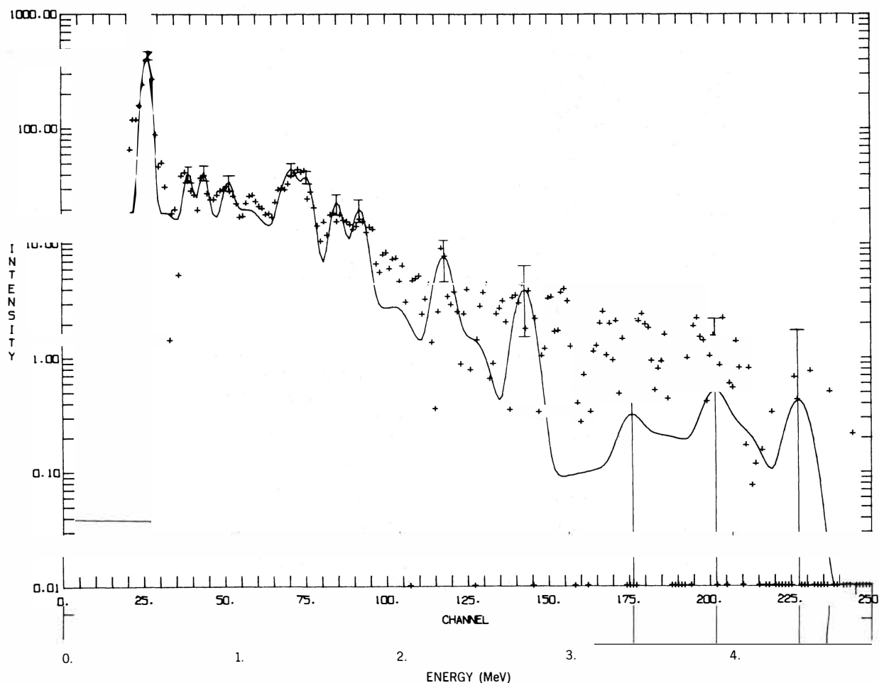
FIG. 2.—The energy-loss spectrum (plus sign) of the discrete line background for the Apollo 16 measurement is compared with the fitted line spectrum (solid line) obtained by the iterative unfolding procedure.
