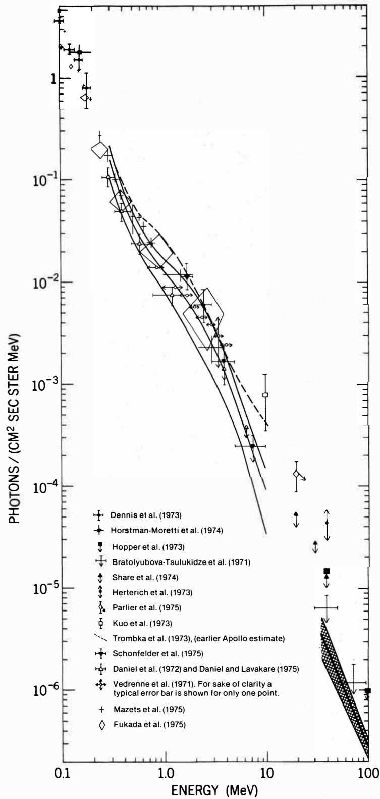
FIG. 5.—The diffuse cosmic gamma radiation observed by several experiments. Some convergence of the data has occurred as awareness of spurious background has increased.
