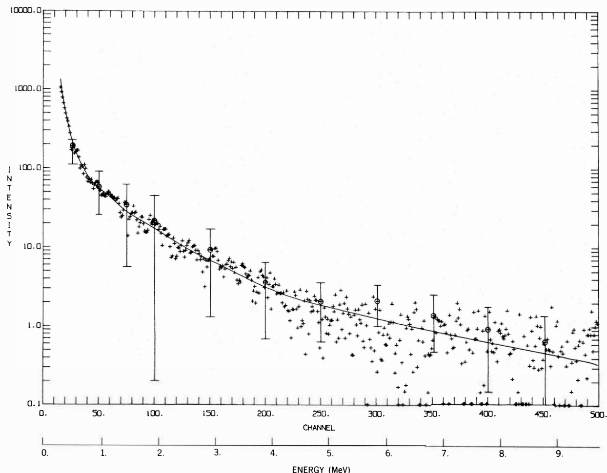
FIG. 3.—The energy-loss spectrum (points) of the cosmic \gamma -ray component obtained after the subtraction of all backgrounds is compared with the energy-loss equivalent (solid line) of the unfolded photon spectrum. Error bars are plotted every 25 or 50 channels and include the effect of statistics and the uncertainties in the subtraction of backgrounds.
