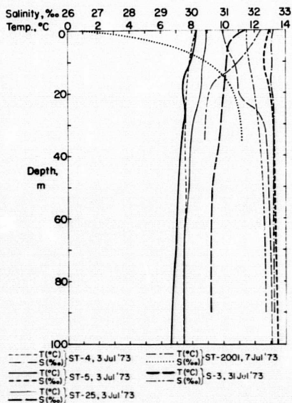
Figure 51. Temperature-salinity profiles, July 1973.
