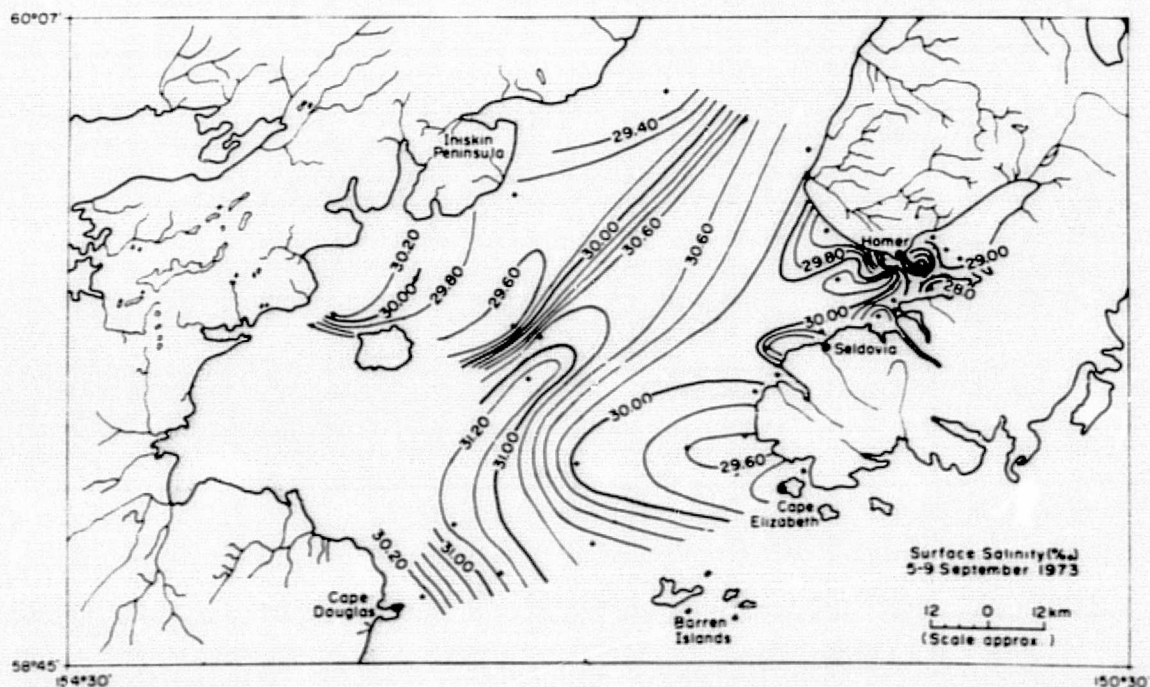
Figure 56. Surface salinity distribution, 5-9 September 1973.
