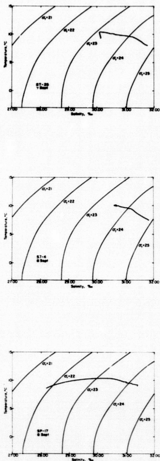
Figure 60. T-S diagrams, stations ST-25, -4 and SP-17.
