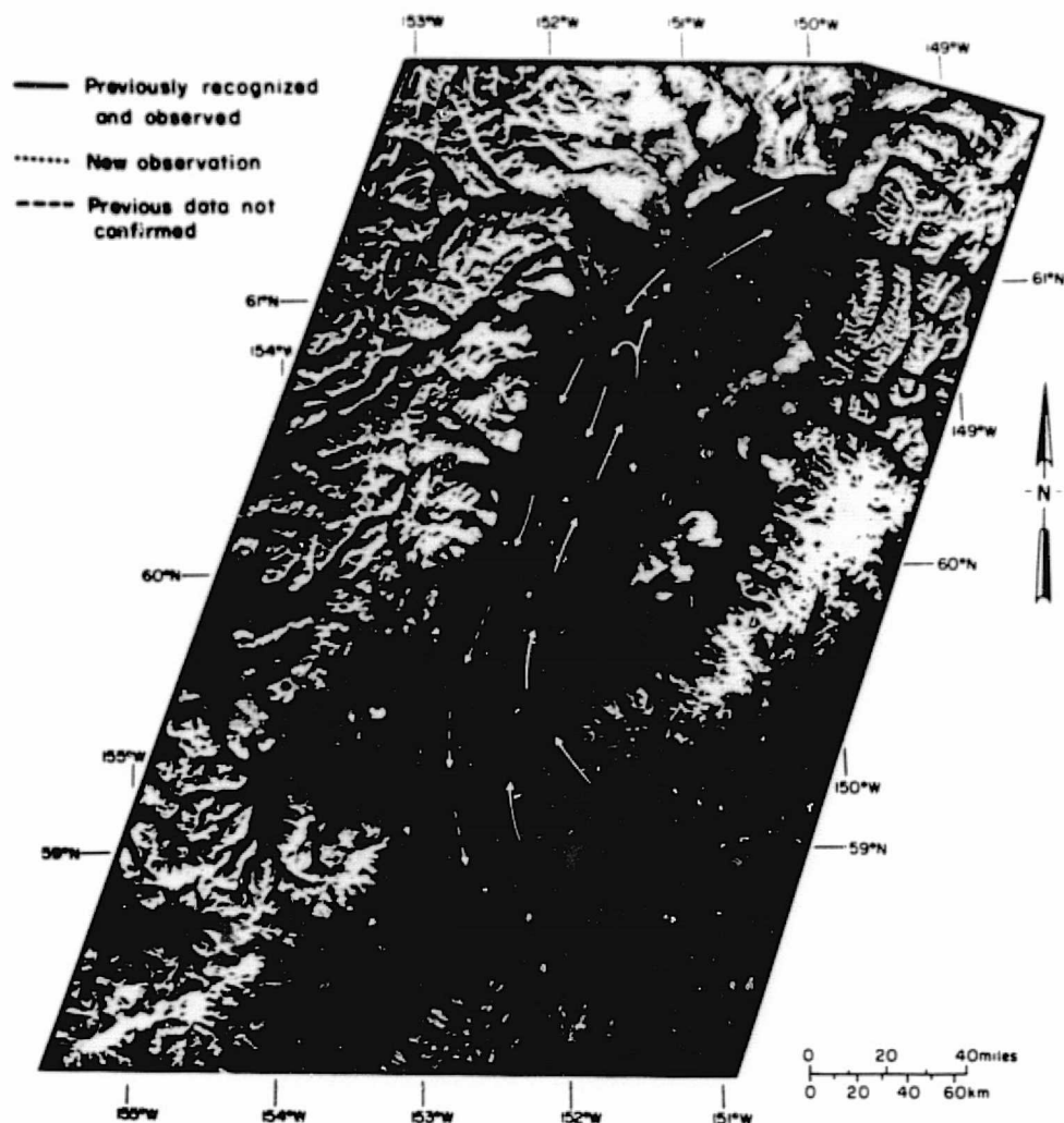
Figure 28. Generalized surface circulation patterns visible on MSS bands 4 and 5 imagery acquired in October and November 1972.
