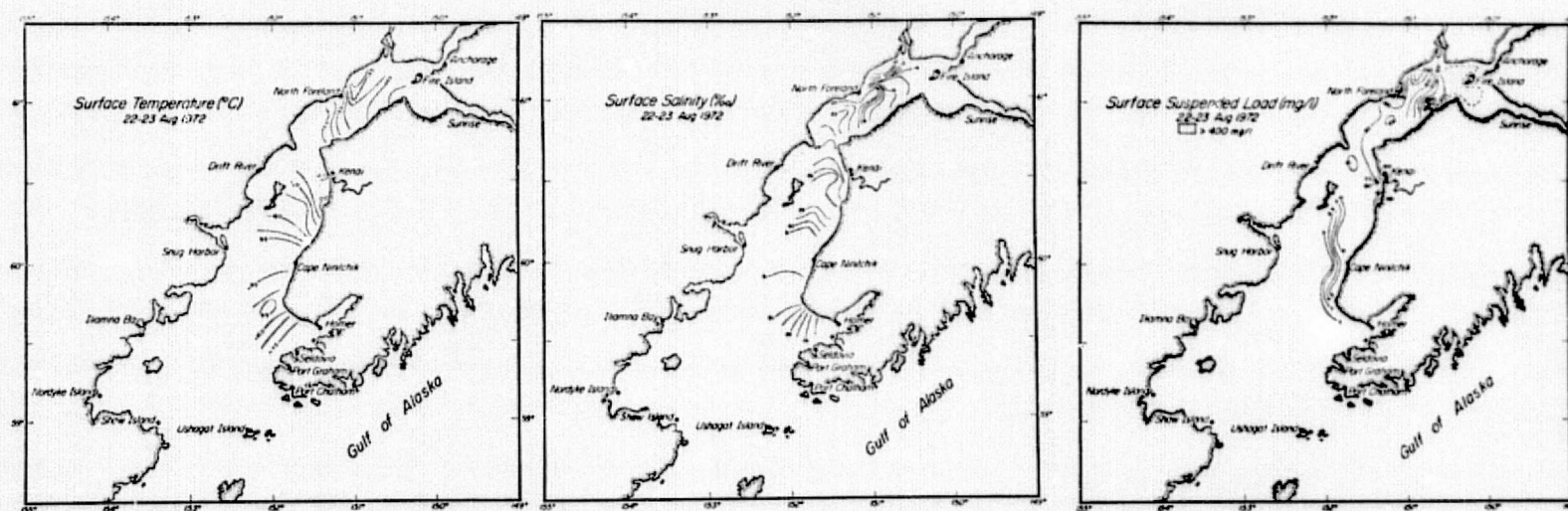
Figure 25. Surface temperature ( ^{\circ}\text{C} ), salinity (parts per thousand) and suspended sediment ( \text{mg/l} ) in August 1972 (adapted from unpublished data provided by F.F. Wright).
