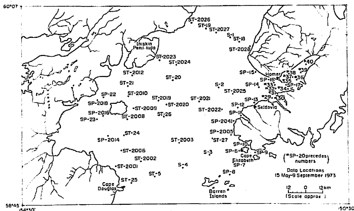
Figure 3. Data locations for NOAA survey from 15 May to 9 September 1973.
