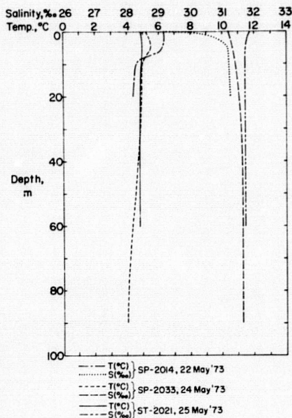
Figure 45. Temperature-salinity profiles, May 1973.
