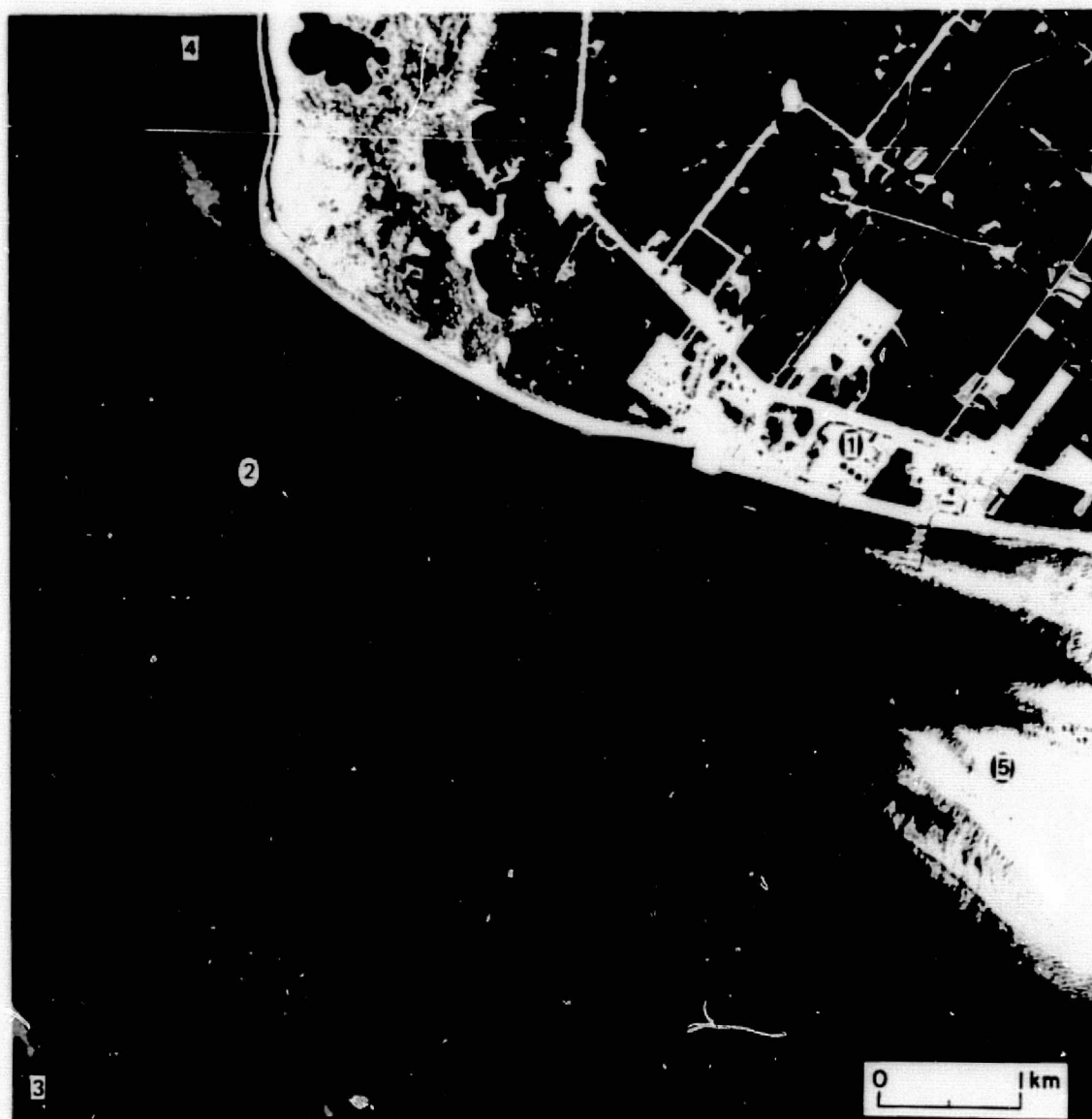
Figure 39. Nikiski wharf — East Foreland area during flood tide (outlined on Figure 37; NASA NP-3A photograph).
