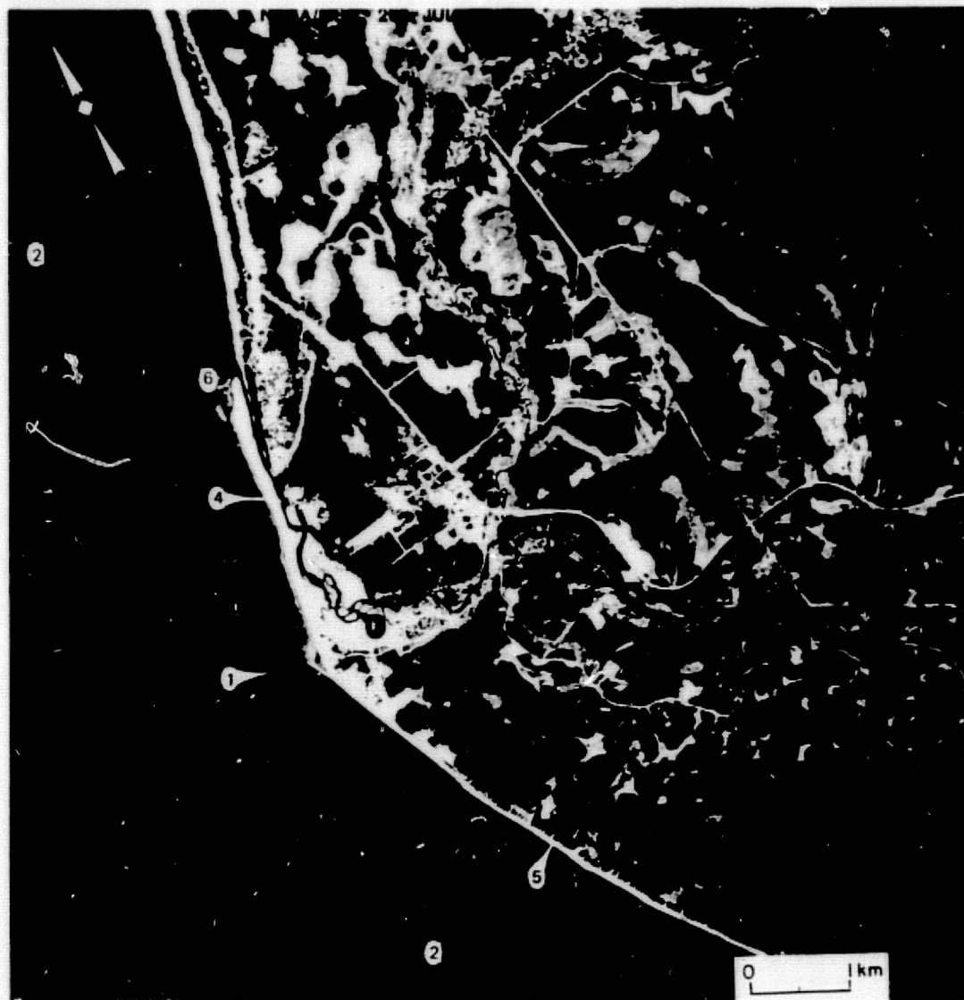
Figure 38. Anchor Point area during flood tide (outlined on Figure 37; NASA NP-3A photograph).
