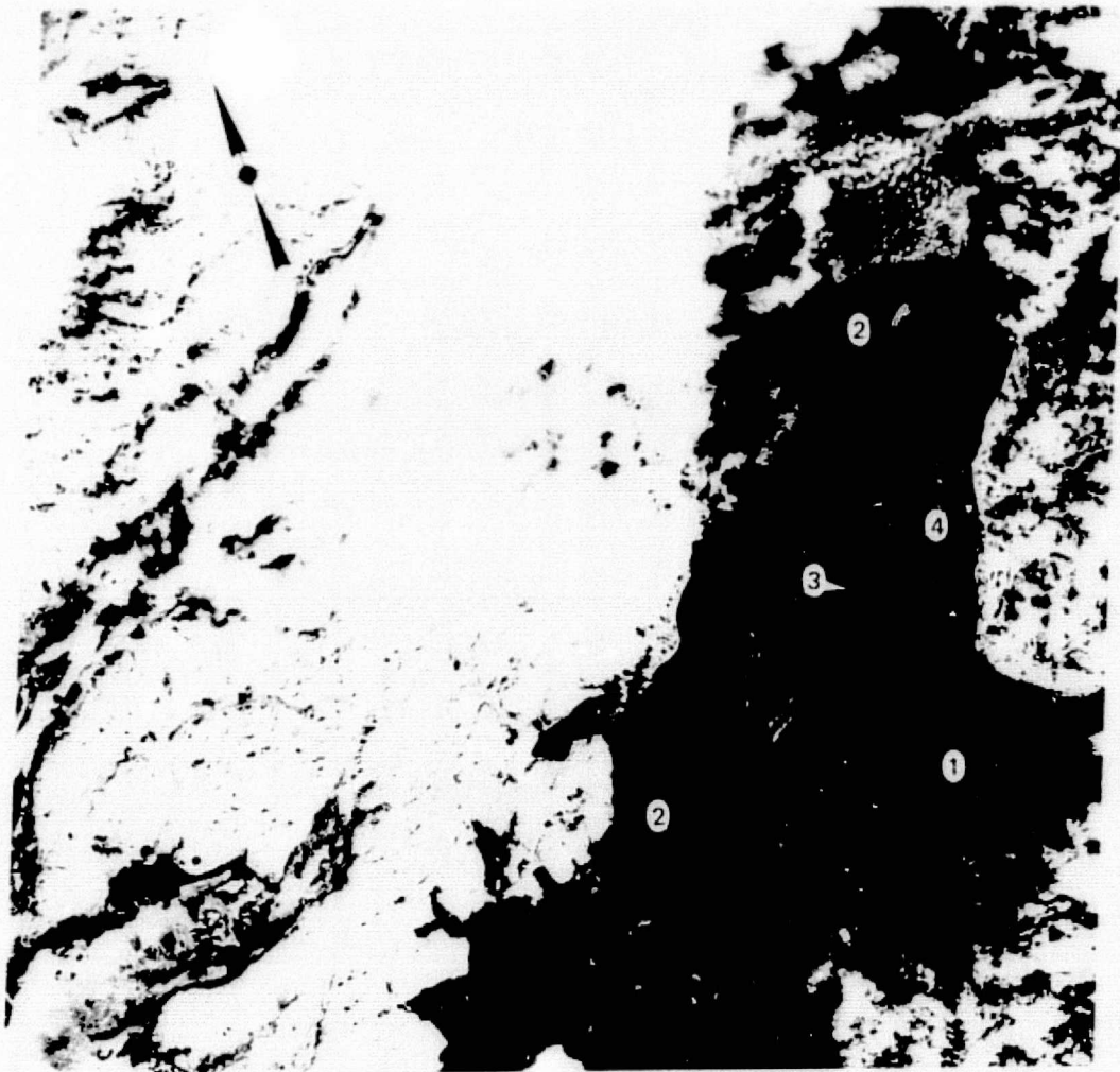
Figure 36. Surface water patterns in southern Cook Inlet. MSS band 5 image 1266-20581, acquired 15 April 1973.
