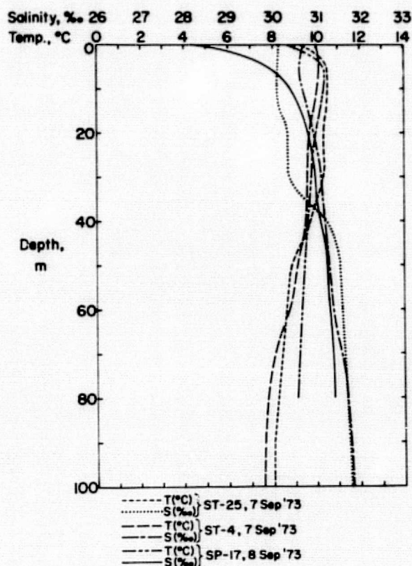
Figure 57. Temperature-salinity profiles, September 1973.
