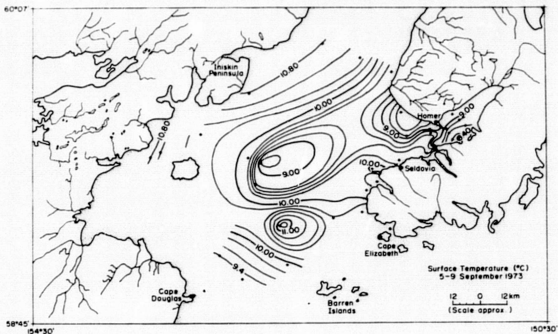
Figure 55. Surface temperature distribution, 5-9 September 1973.
