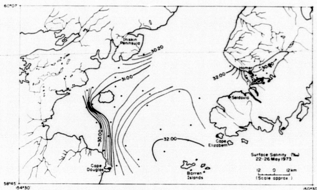
Figure 42. Surface salinity distribution, 22-26 May 1973.
