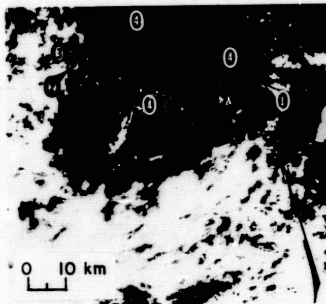
Figure 40. Surface water patterns near Kalgin Island. From MSS band 5 image 1410-20513, acquired 6 September 1973.
