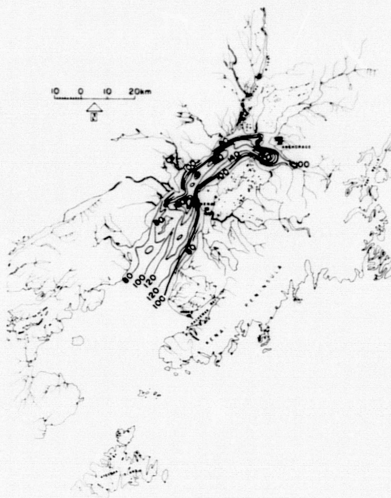
Figure 27. Predicted maximum tidal currents (cm/sec) (after Evans et al. 1972).
