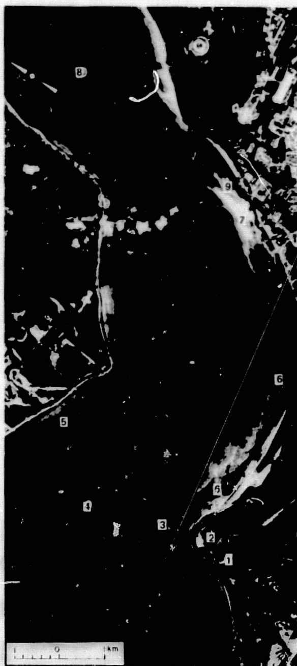
Figure 67. Anchorage area during early flood tide (outlined in Figure 66; NP-3A photograph).
