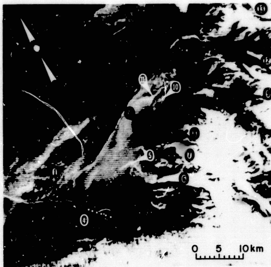
Figure 65. Kachemak Bay. 2x enlargement from LANDSAT MSS band 4 image 1066-20452, acquired 27 September 1972 (scale approximate).
