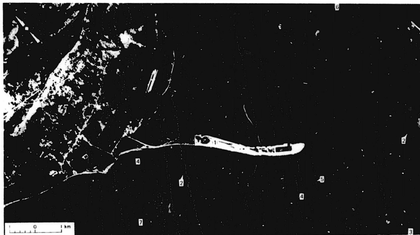
Figure 22. Homer Spit area during flood tide at Seldovia (NASA NP-3A photographs).
