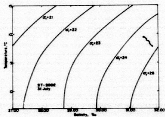
Figure 59. T-S diagrams, stations ST-25 and -2002.
