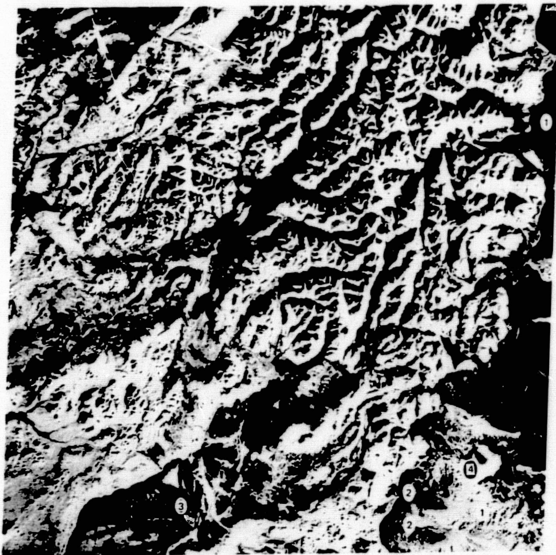
Figure 61. Distribution of inlet ice along the southwest shore. MSS band 5 image 1555-20591, acquired 29 January 1974.
