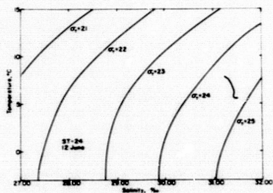
Figure 58. T-S diagrams, stations ST-2006, -2008, -24.
