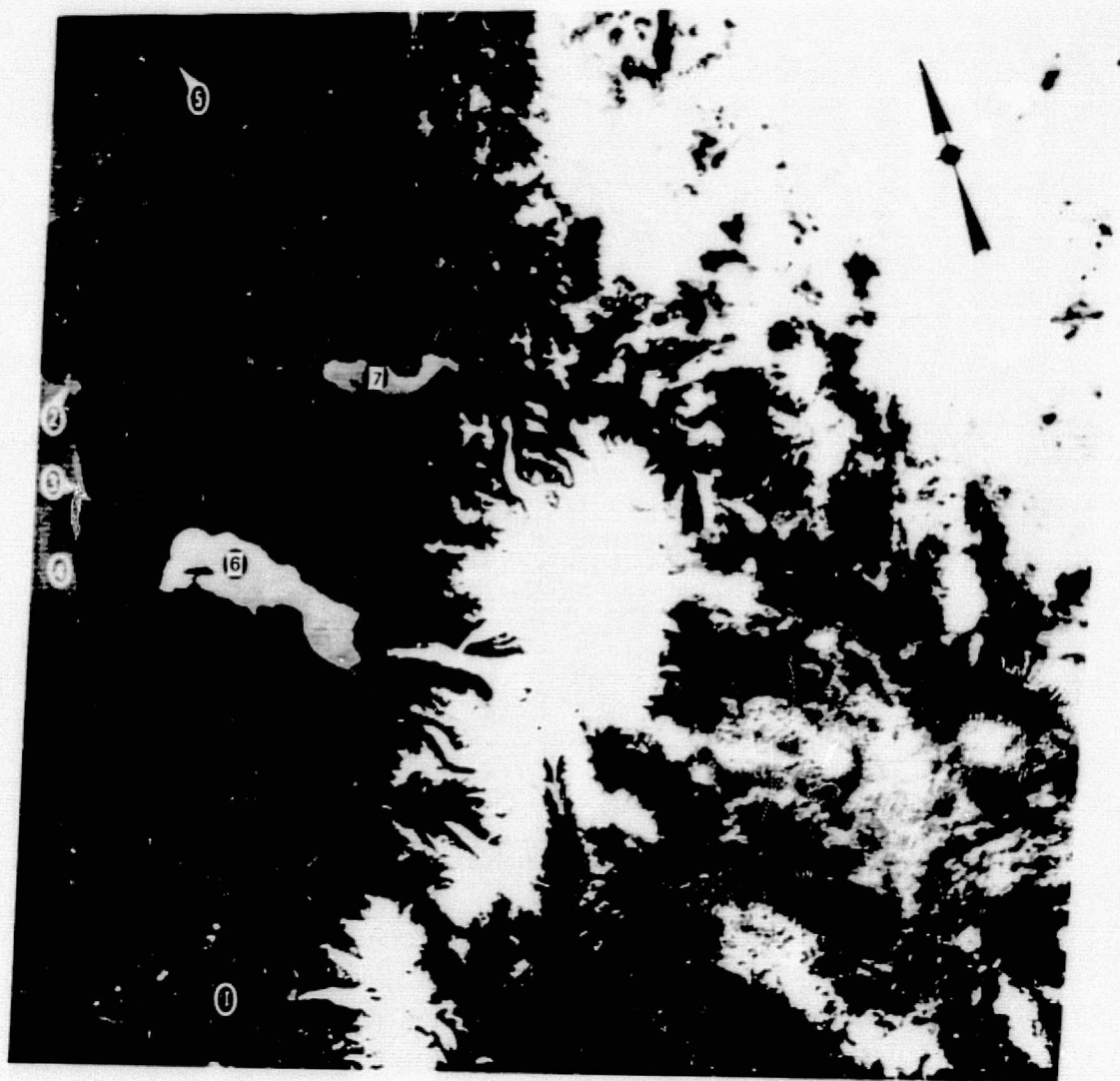
Figure 20. Southeastern Cook Inlet. MSS band 4 image 1426-20444, acquired 22 September 1973; early ebb at Anchorage, high water at Seldovia.
