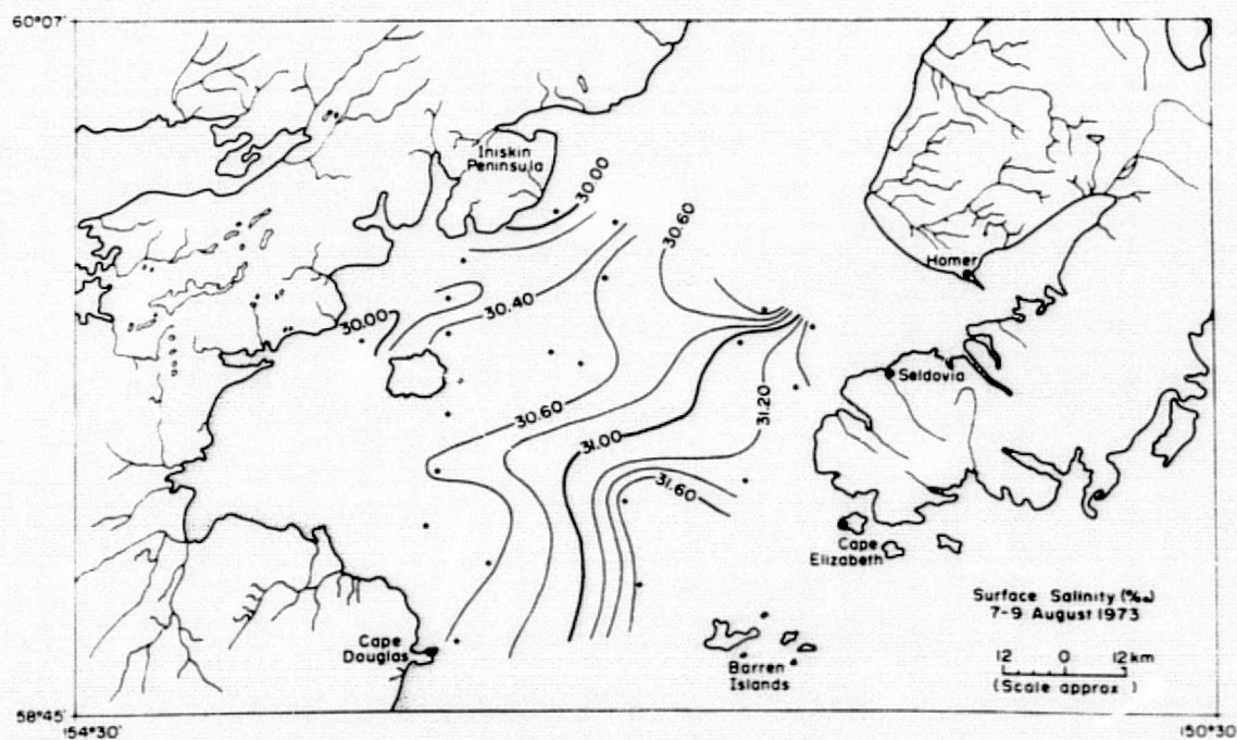
Figure 53. Surface salinity distribution, 7-9 August 1973.
