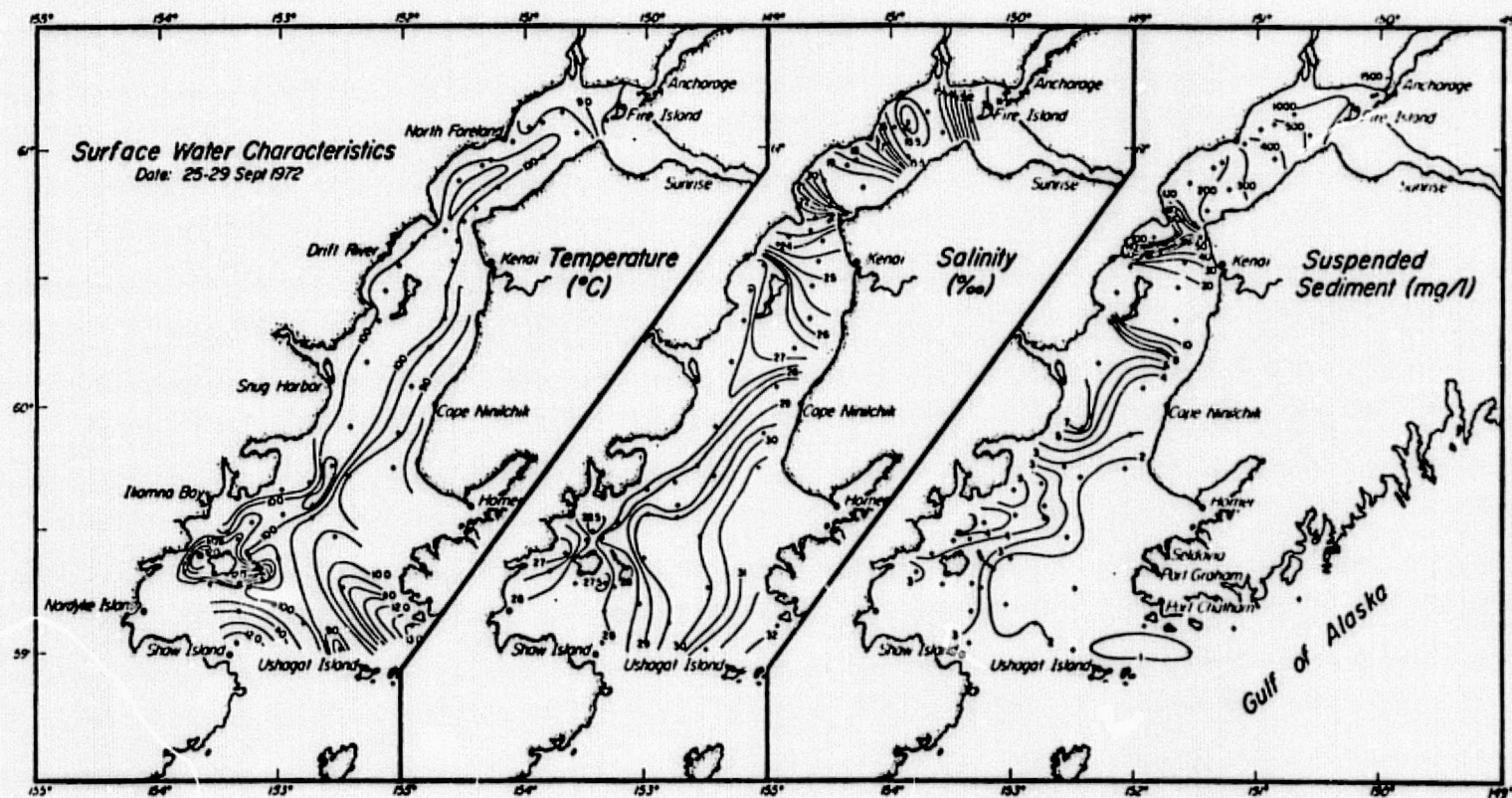
Figure 26. Surface temperature ( ^{\circ}\text{C} ), salinity (parts per thousand) and suspended sediment ( \text{mg/l} ) in September 1972 (adapted from Wright and Sharma 1973).
