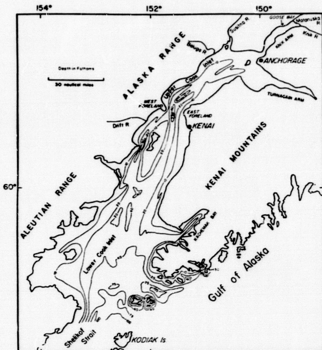
Figure 13. Generalized bathymetry of Cook Inlet (from Sharma and Burrell 1970).
