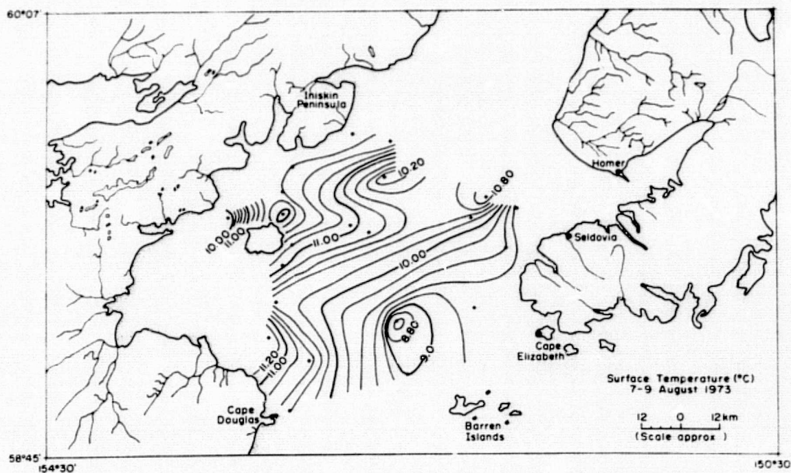
Figure 52. Surface temperature distribution, 7-9 August 1973.
