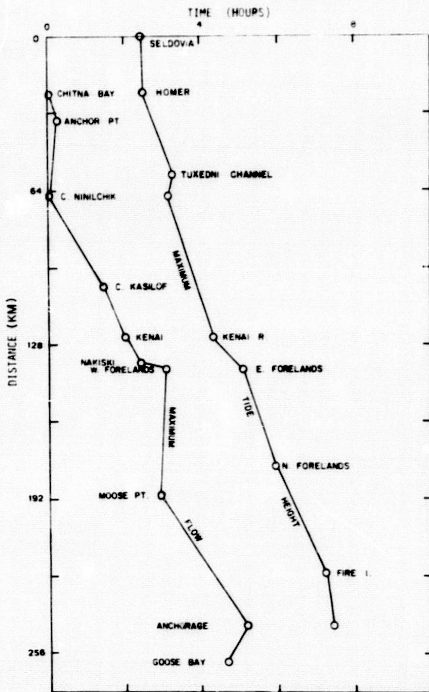
Figure 15. Difference between time of high tide and maximum flow (adapted from Carlson and Behlke 1972).
