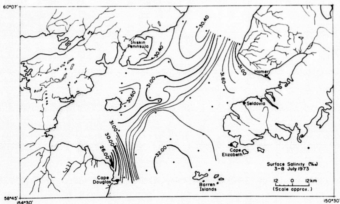
Figure 50. Surface salinity distribution, 3-8 July 1973.
