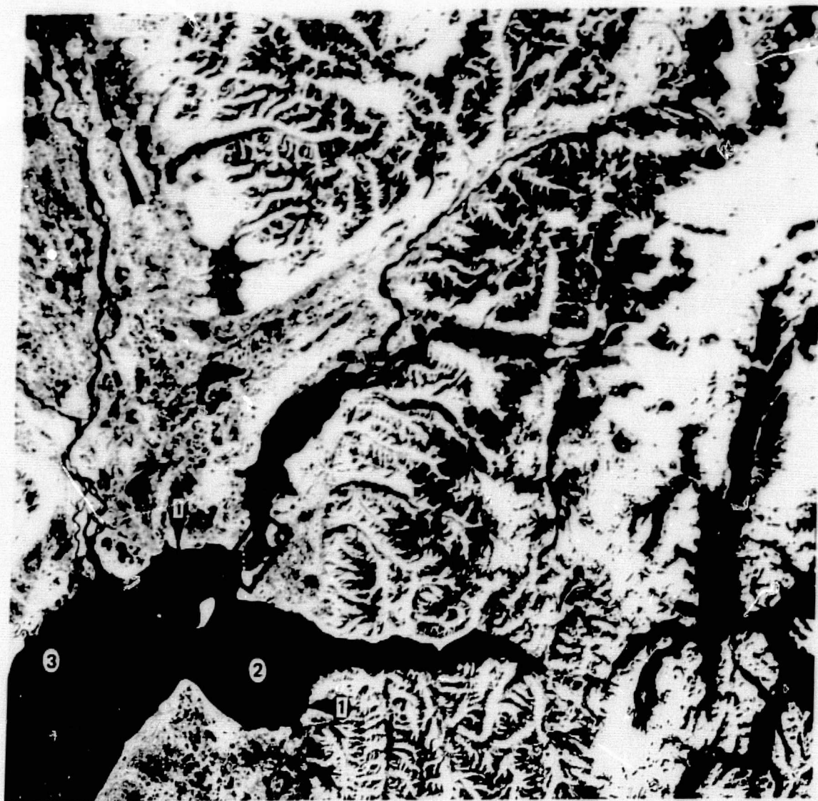
Figure 66. Northern Cook Inlet. LANDSAT MSS band 7 image 1390-20450, acquired 17 August 1973; ebb tide at Anchorage.
