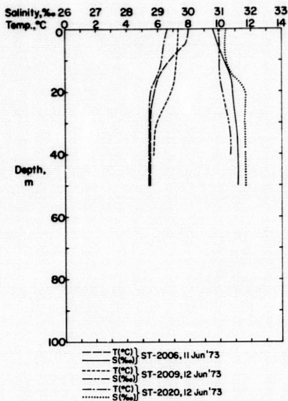
Figure 48. Temperature-salinity profiles, June 1973.
