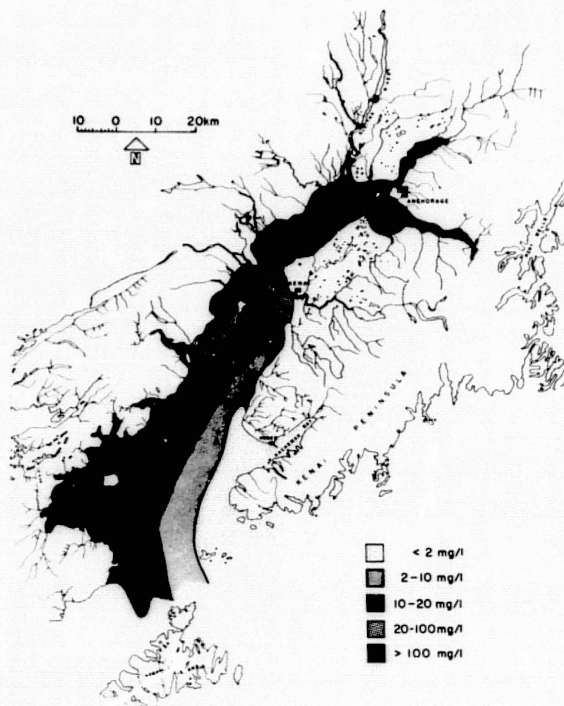
Figure 35 Generalized surface suspended sediment distribution (after Sharma et al. 1973).
