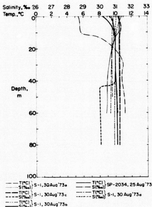
Figure 54. Temperature-salinity profiles, August 1973.
