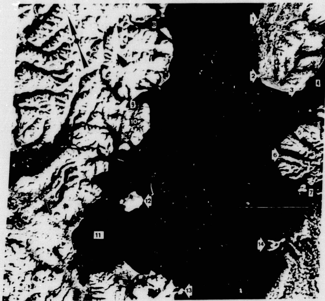
Figure 6. Southern portion of Cook Inlet. MSS band 6 image 1704-20574, acquired 4 November 1972.
