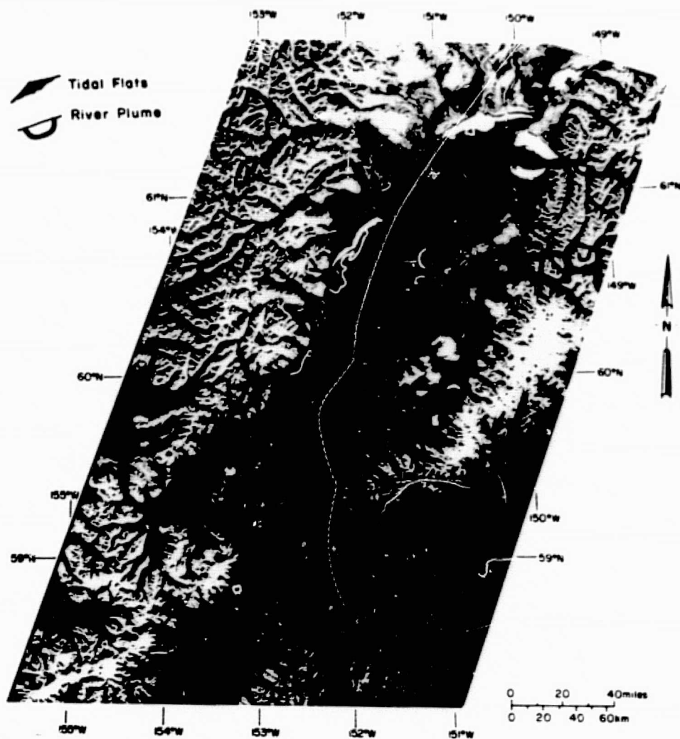
Figure 12. Tidal flat distribution and river plumes.
