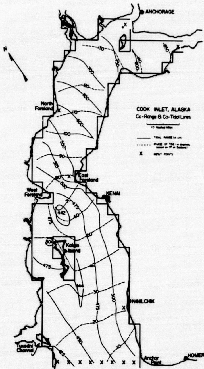
Figure 14. Co-tidal and co-range lines (from Mungall and Matthews 1970).
