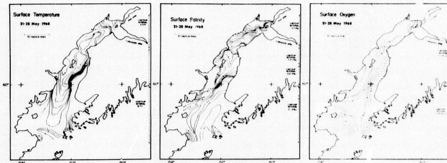
Figure 24. Surface temperature ( ^{\circ}\text{C} ), salinity (parts per thousand) and oxygen ( \text{mLO}_2/\text{l} ) in May 1968 (adapted from Kinney et al. 1970b).
