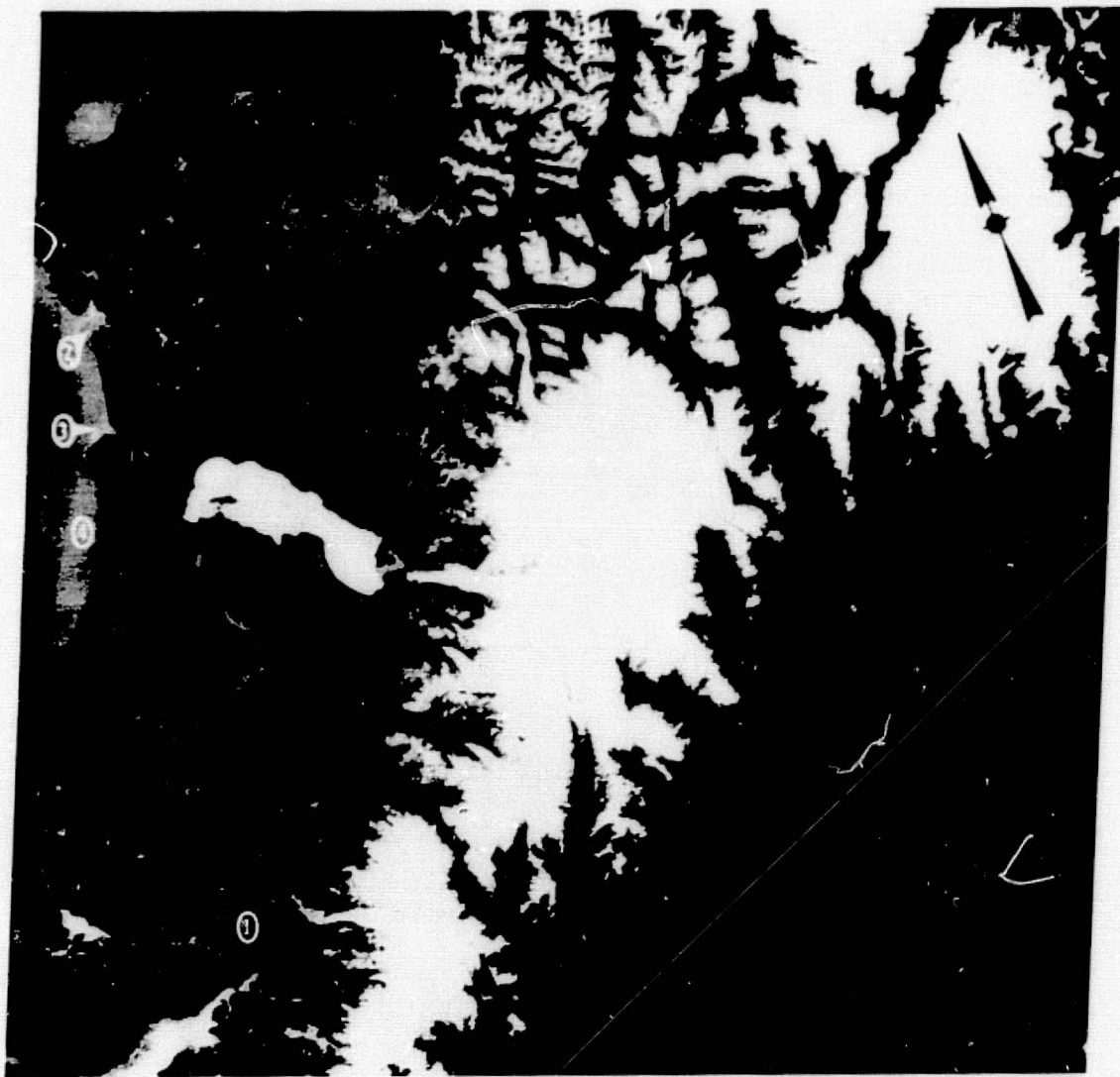
Figure 19. Southeastern Cook Inlet. MSS band 5 image 1390-20452, acquired 17 August 1973; early ebb at Anchorage, early flood at Seldovia.
