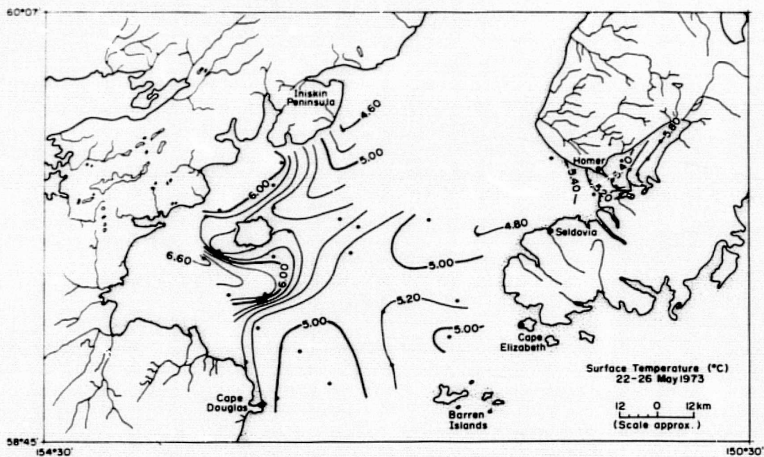
Figure 41. Surface temperature distribution, 22-26 May 1973.
