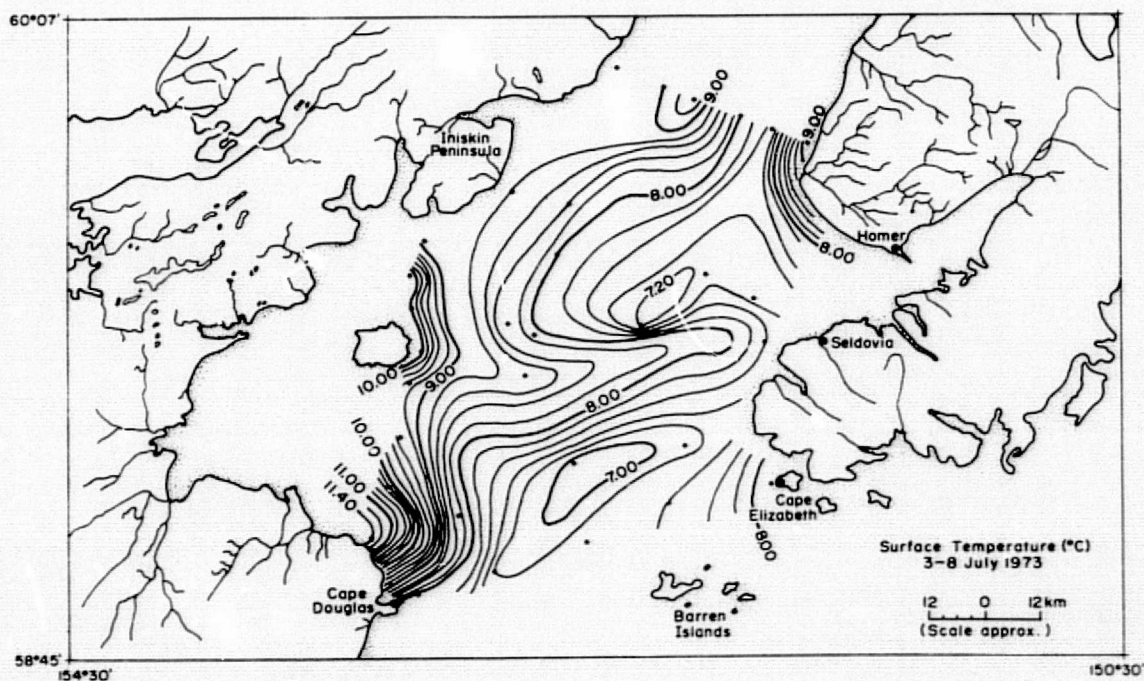
Figure 49. Surface temperature distribution, 3-8 July 1973.
