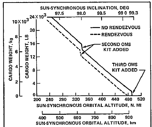
Cargo weights compared to altitudes in sun-synchronous orbits.
