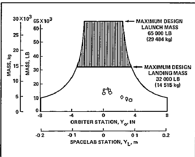
Basic Spacelab center-of-gravity locations along the Y-axis.
