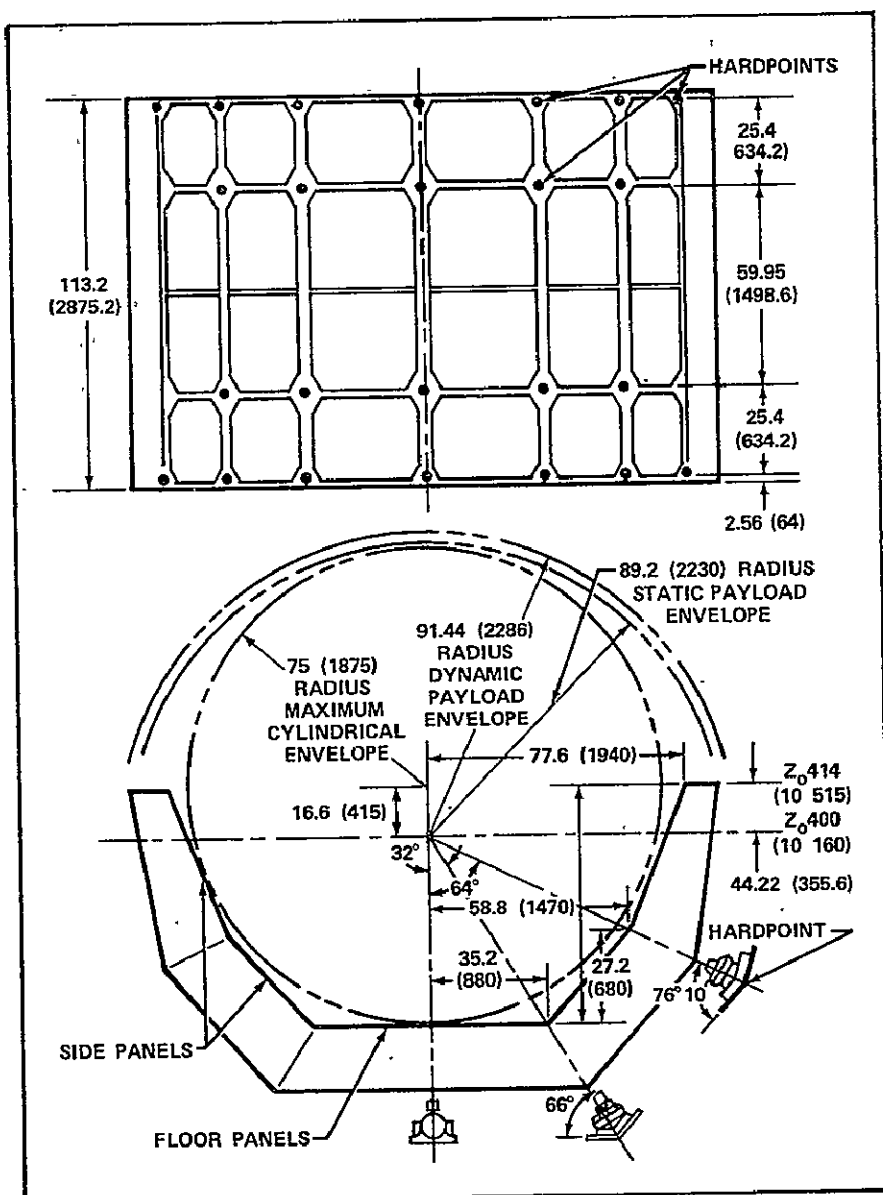
Hardpoints and envelope for pallet payloads.
