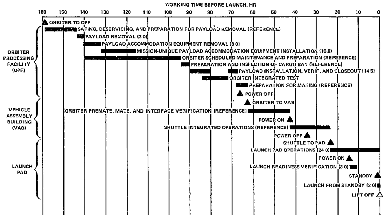
Typical processing schedule for payloads installed at the Orbiter Processing Facility. Allocated times shown are approximate only. The lines marked as reference indicate STS processing that does not involve the payload; they are shown to acquaint users with the overall ground flow.
