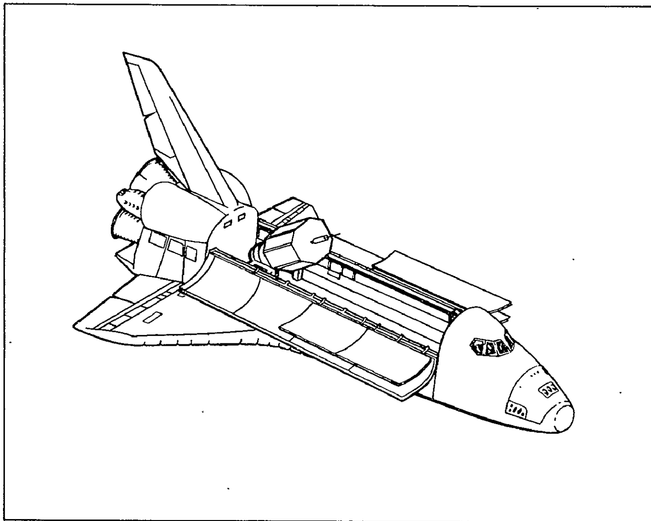
SSUS tilt/spin table mounted in the Orbiter cargo bay.
