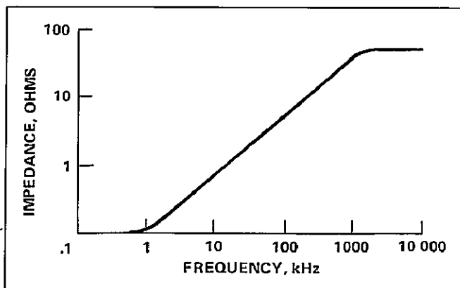
Orbiter dc power source impedance.
