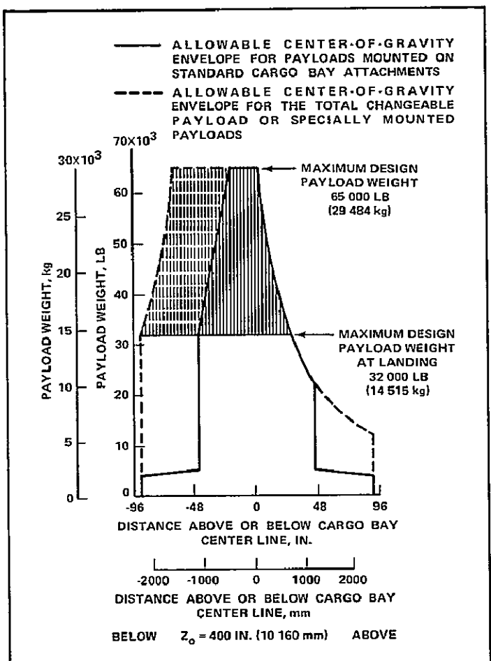
Center-of-gravity limits of cargo along the Z-axis (Z O ) of the Orbiter.
