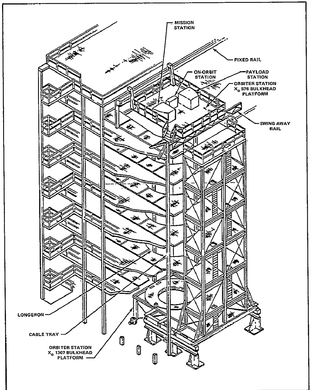
Vertical cargoes can undergo interface verification in this CITE configuration.
