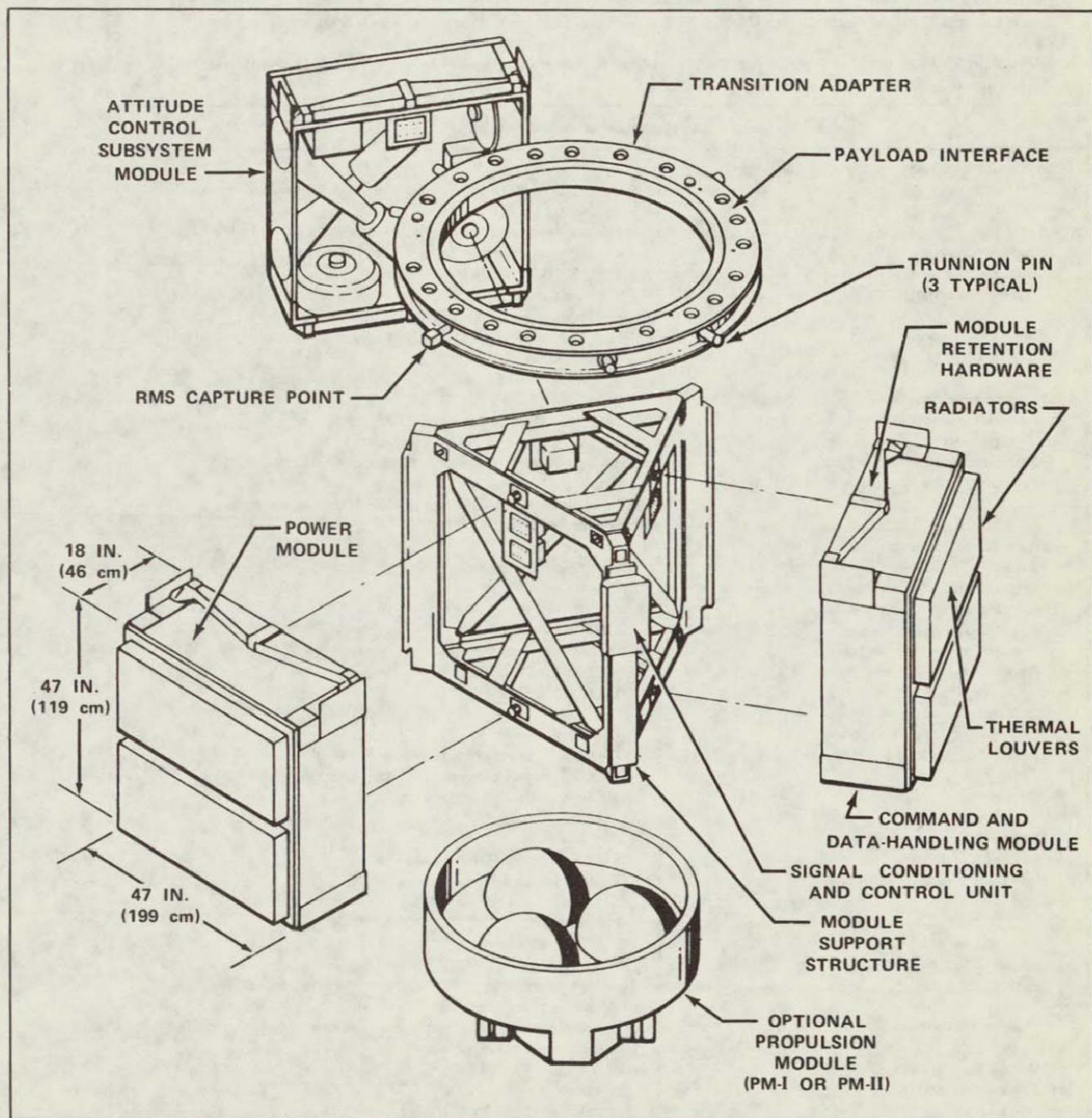
Modular mechanical subsystem components of the MMS.
