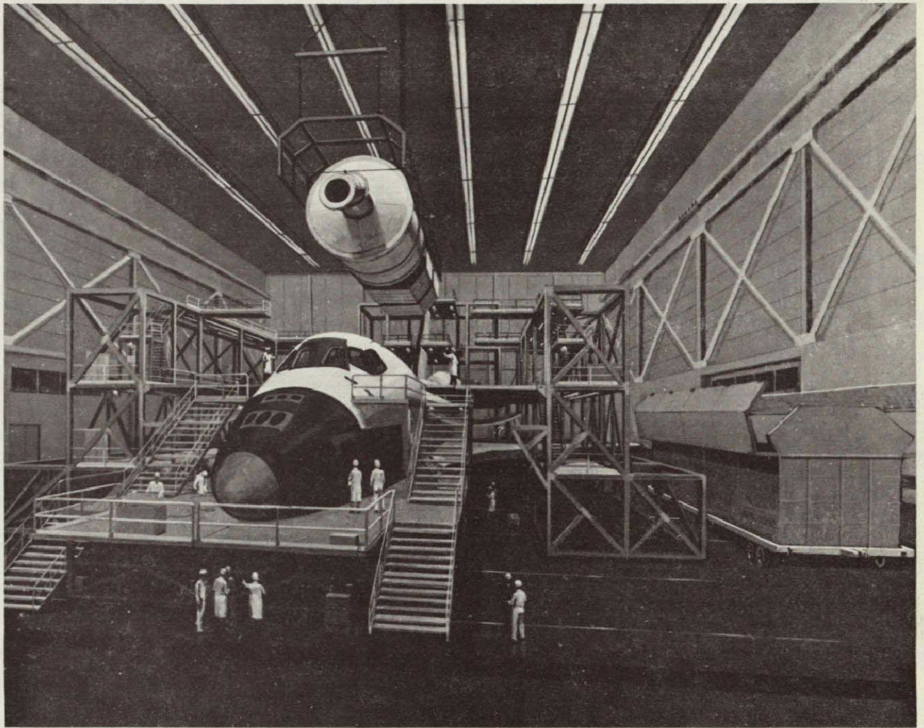
Strongback in use for horizontal installation of Spacelab. The empty canister is also clearly visible.
