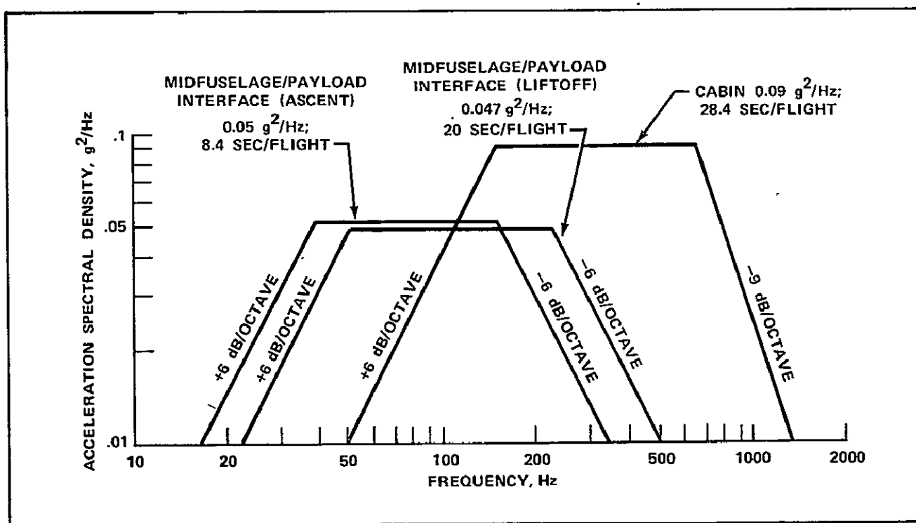
Random vibration at midfuselage main longeron payload attachment points interface and in the cabin. These levels are typical of liftoff, transonic flight, and flight at maximum aerodynamic pressure.
