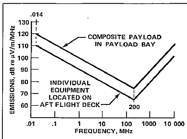
Payload allowable radiated broadband emissions.
