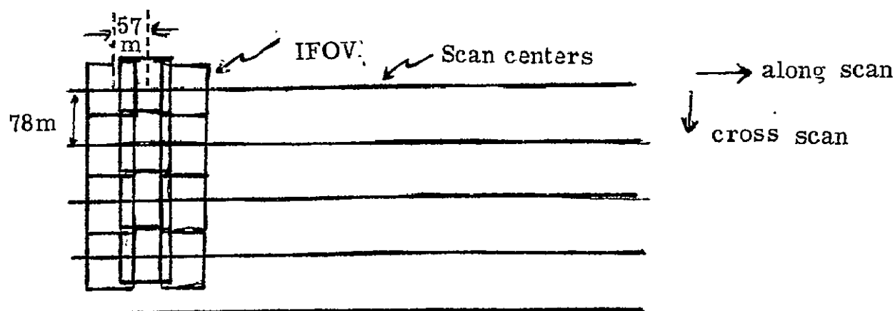
Fig 2.B-1 Sensor Sampling Convention
