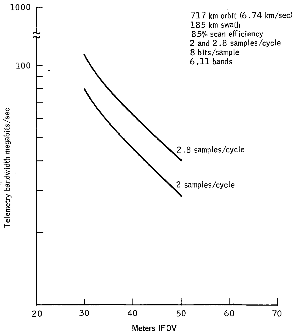
Figure A-1. - Telemetry bandwidth vs IFOV.
