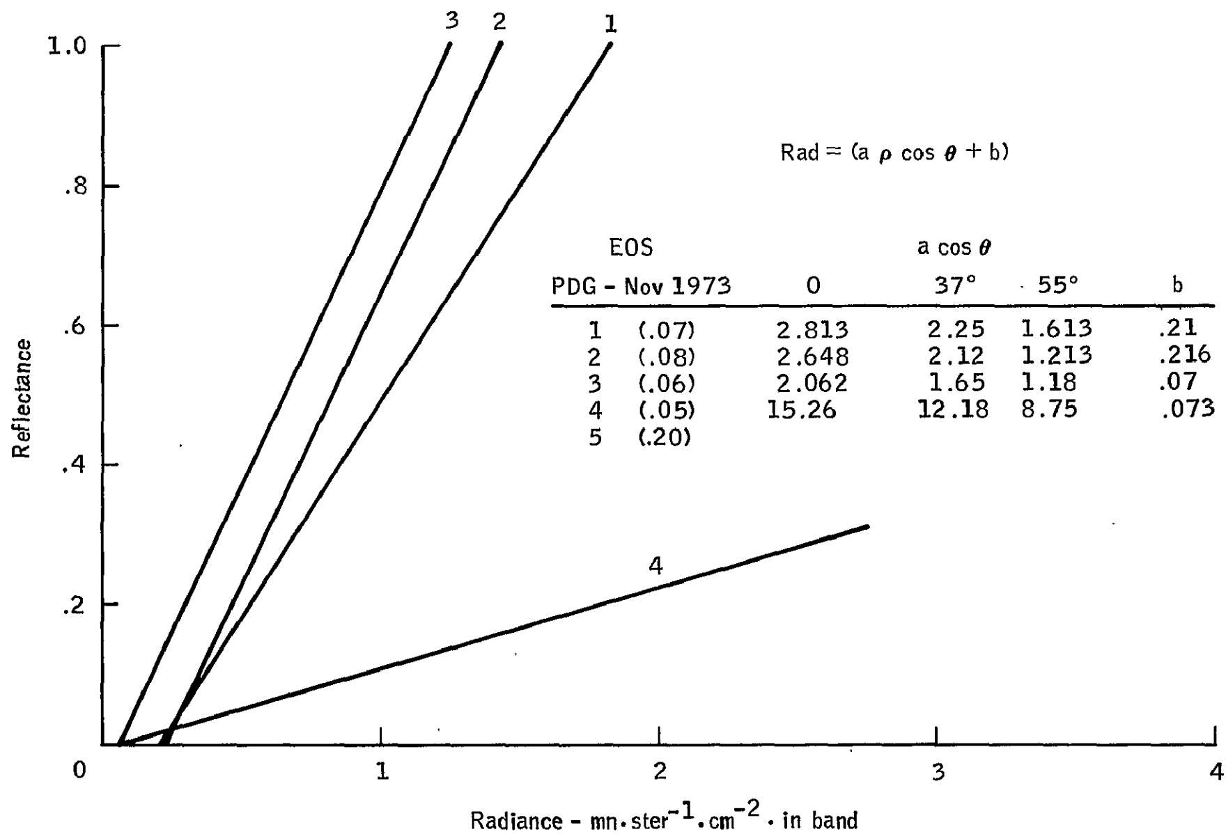
Figure B-1. - Reflectance vs radiance in EOS-PDG bands (Rogers & Peacock) Z = 55^\circ .
