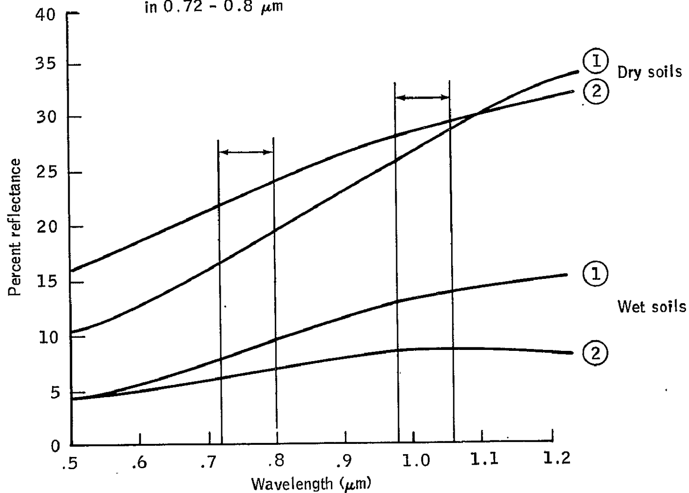
Figure 2. - Reflectance of wet and dry soils.
