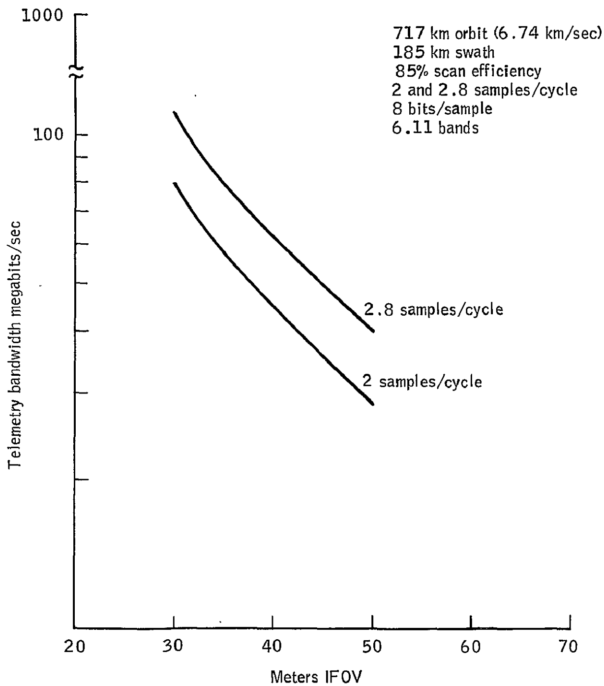
Figure 5. - Telemetry bandwidth vs IFOV.
