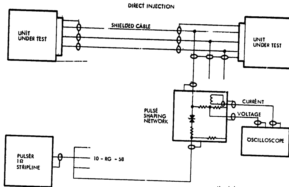
Figure 10. Direct Injection Coupling Technique
