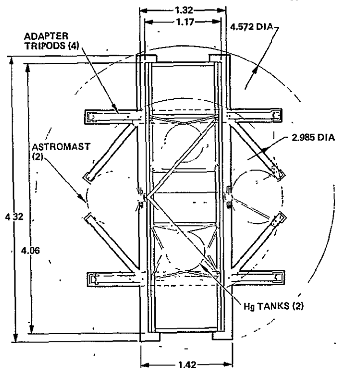
Figure 13. Thrust system layout.
