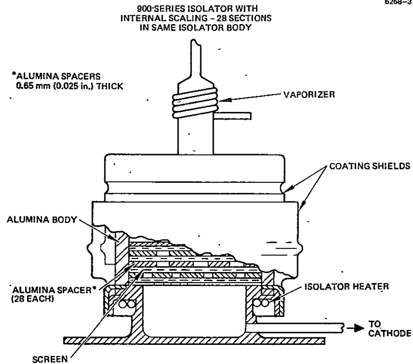
(a) High-voltage propellant electrical isolator using multisegment design concept.
