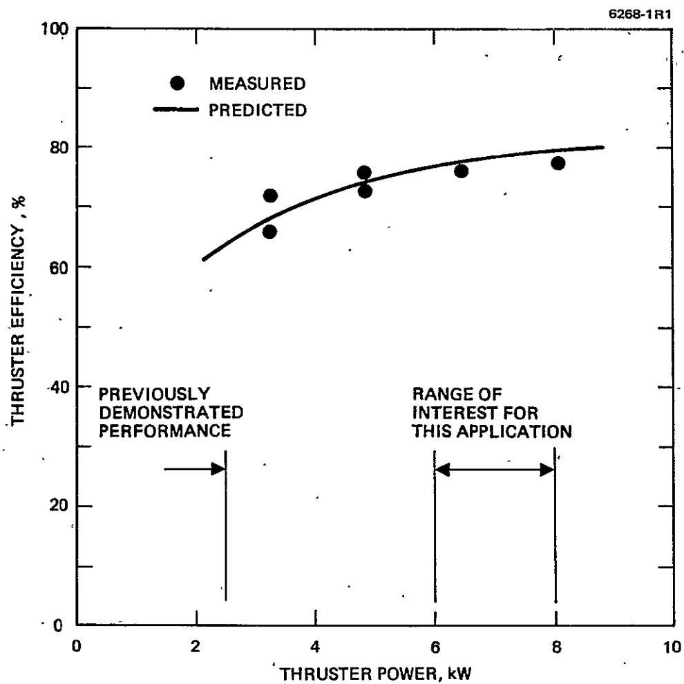
Figure 30. Comparison of measured and predicted thruster performance.
