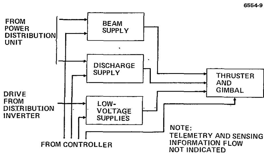
(b) Half of thrust module (one thruster).
