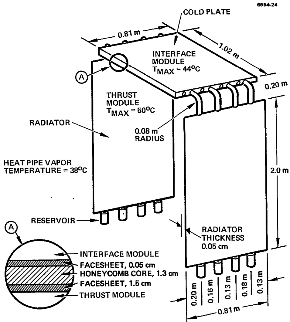
Figure 17. Radiator/ VCHP design description.
