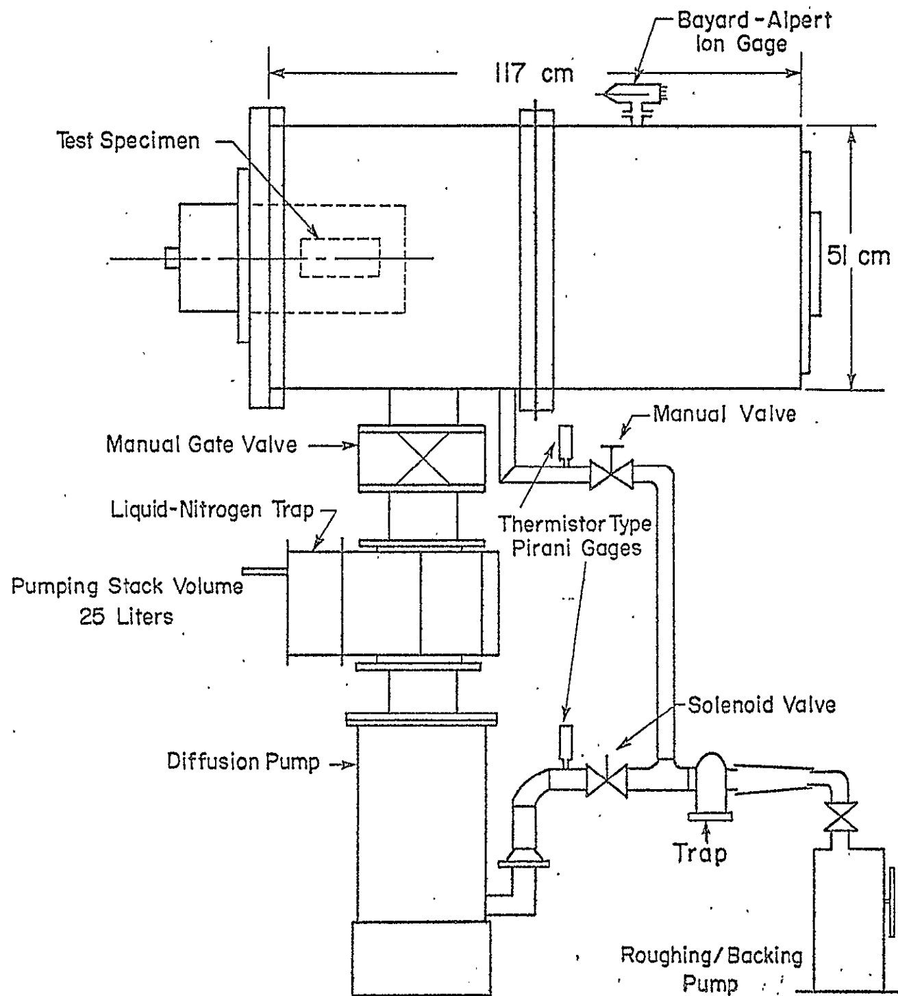
FIG.C2 SYSTEM SCHEMATIC
