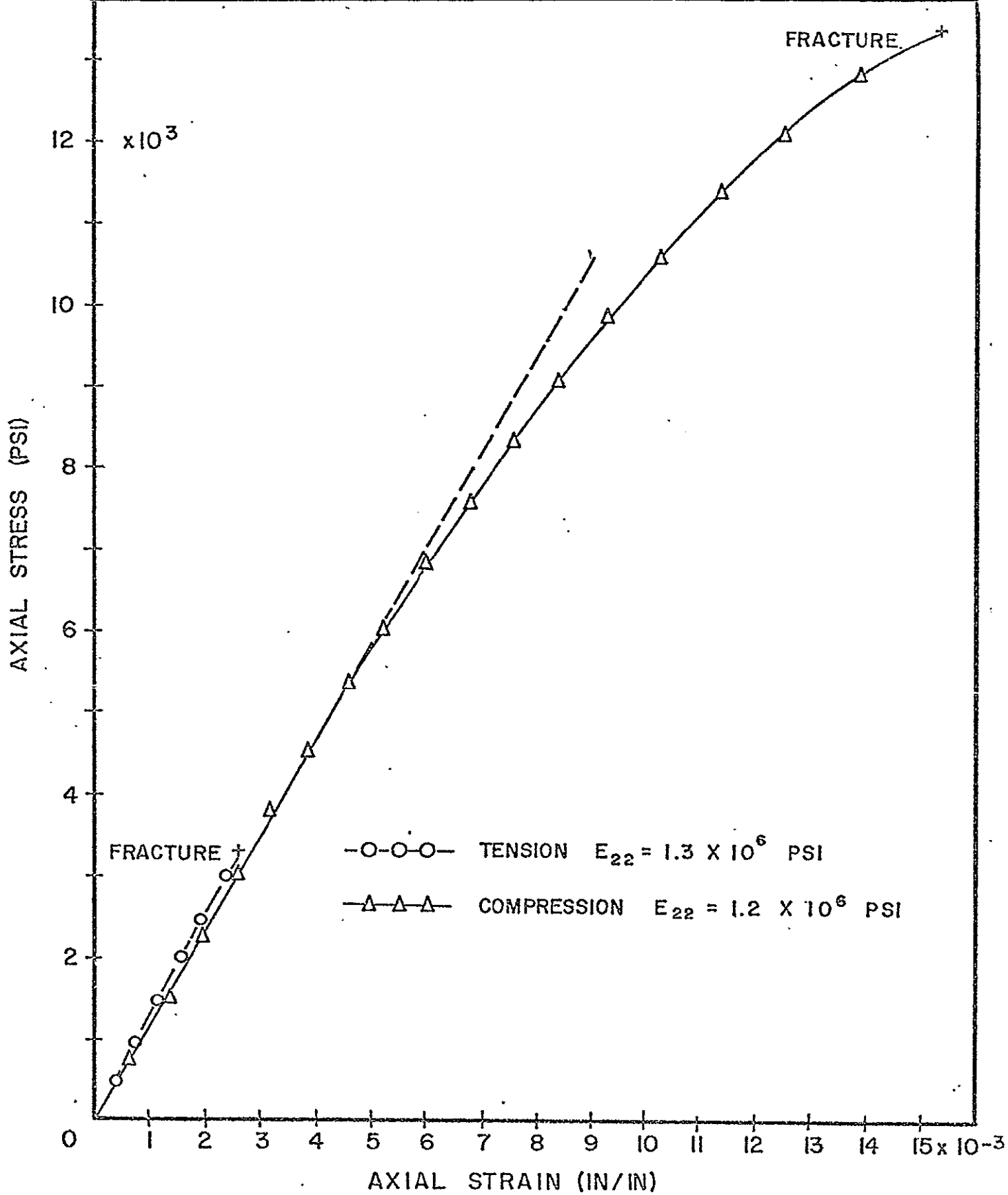
FIG. 6 STRESS-STRAIN CURVES FOR SCOTCHPLY (1002) LOADED PERPENDICULAR TO FIBER DIRECTION
