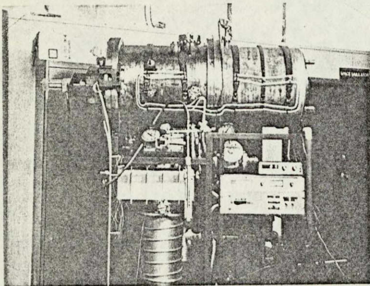
(a) Thermal Vacuum Test Facility.
