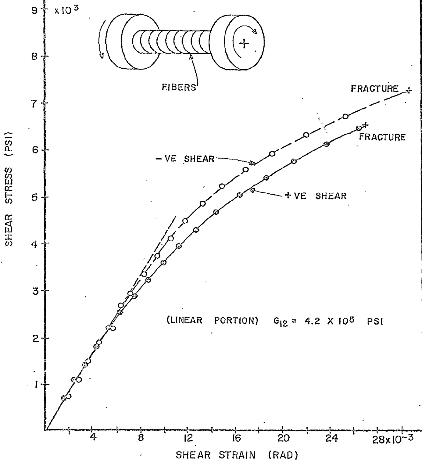
FIG. 7 STRESS-STRAIN CURVES FOR SCOTCHPLY (1002) IN PURE SHEAR
