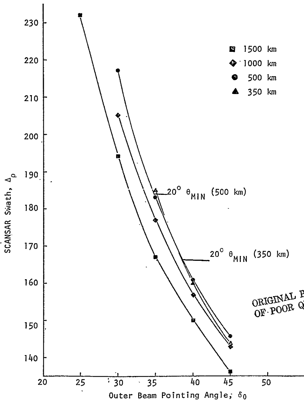
FIGURE 3a. Effect of Outer Beam Pointing Angle on SCANSAR Swath - 10 m Antenna, 5 Scan Cells, Safety Factor of 2 on Range and Azimuth.
