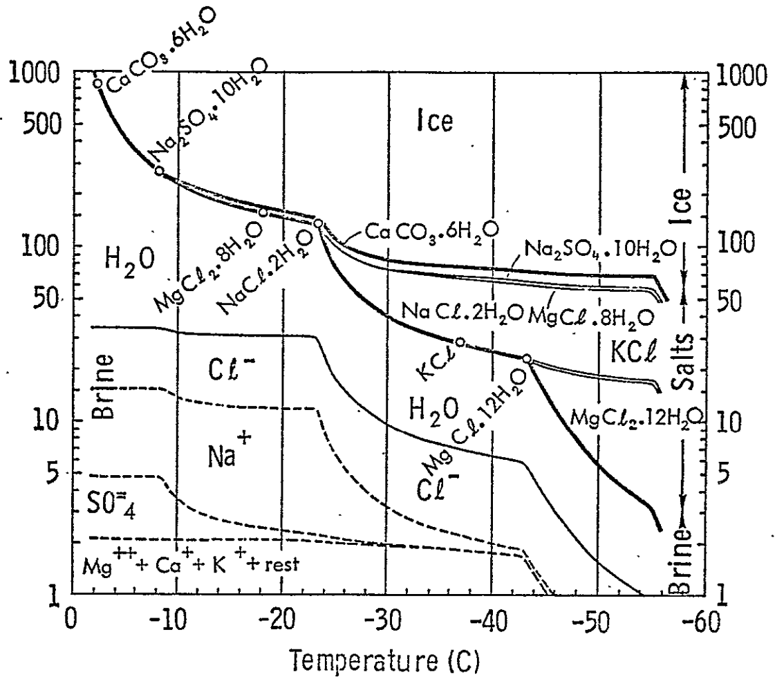
Figure 1. Phase relations for "standard" sea ice. Circles on the brine-salt line indicate temperatures at which solid salts precipitate (Assur, 1958 (31)).
