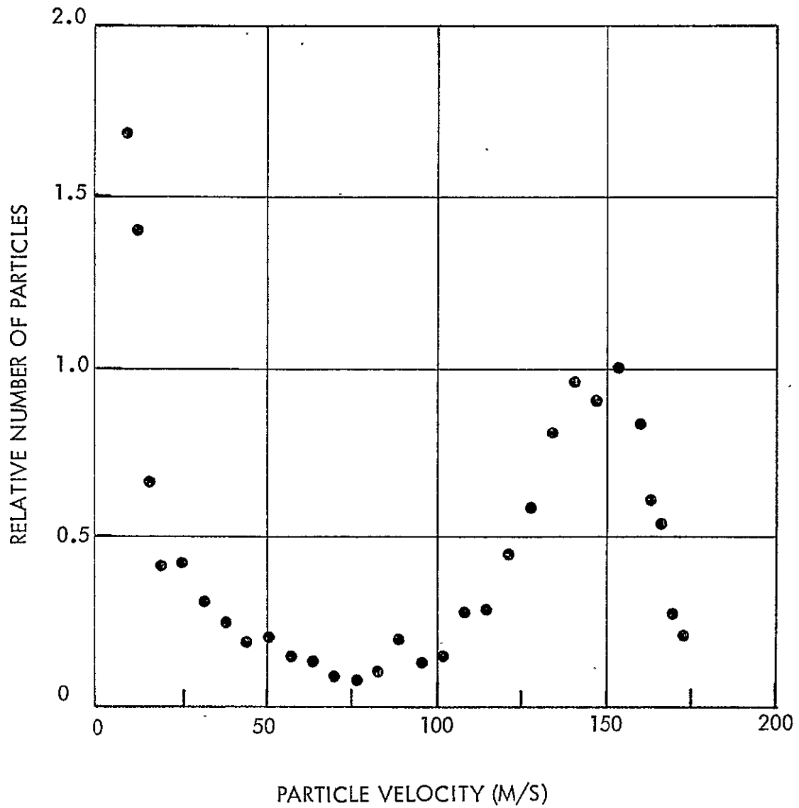
Fig. 5-5. 13 \mu\text{m} polystyrene spheres, 343 \mu\text{m} diameter orifice, 3.2 mm long
