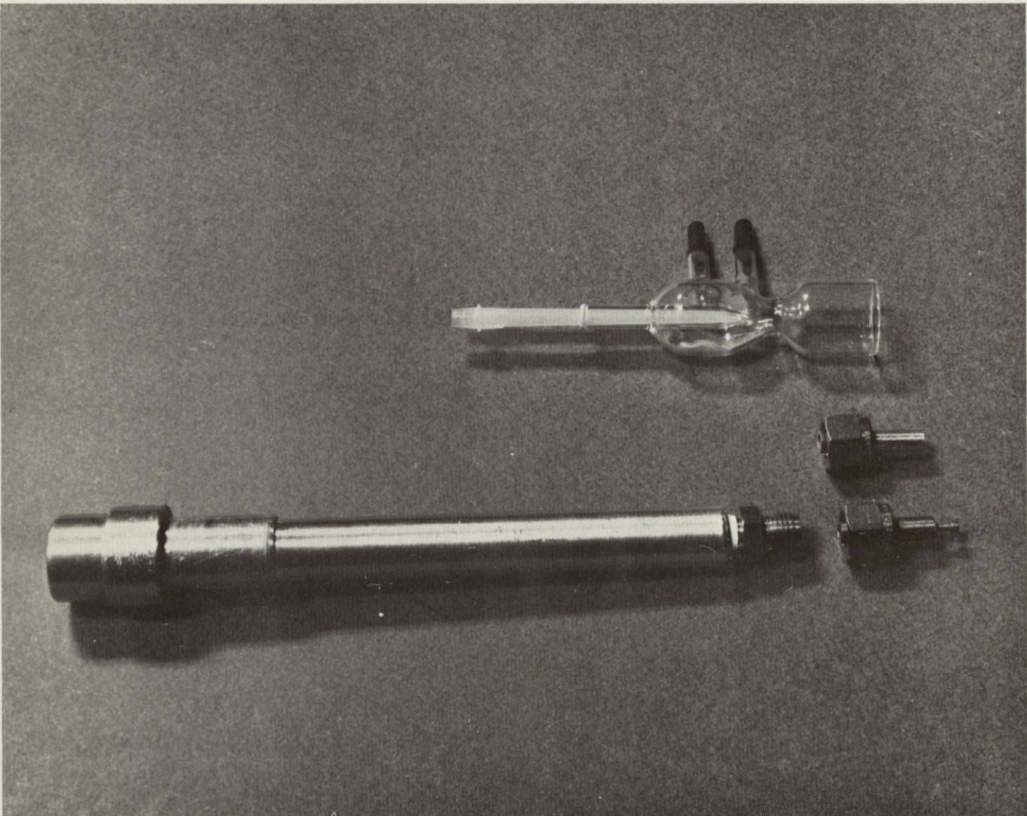
Fig. 3-4. Particle Generator
