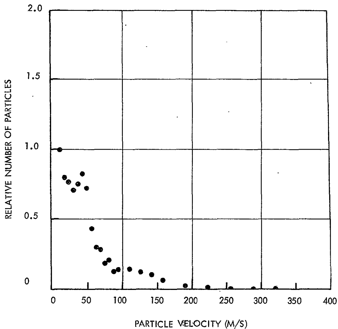
Fig. 5-8. 88 - 125 \mu\text{m} glass spheres, 343 \mu\text{m} diameter orifice, 125 \mu\text{m} long
