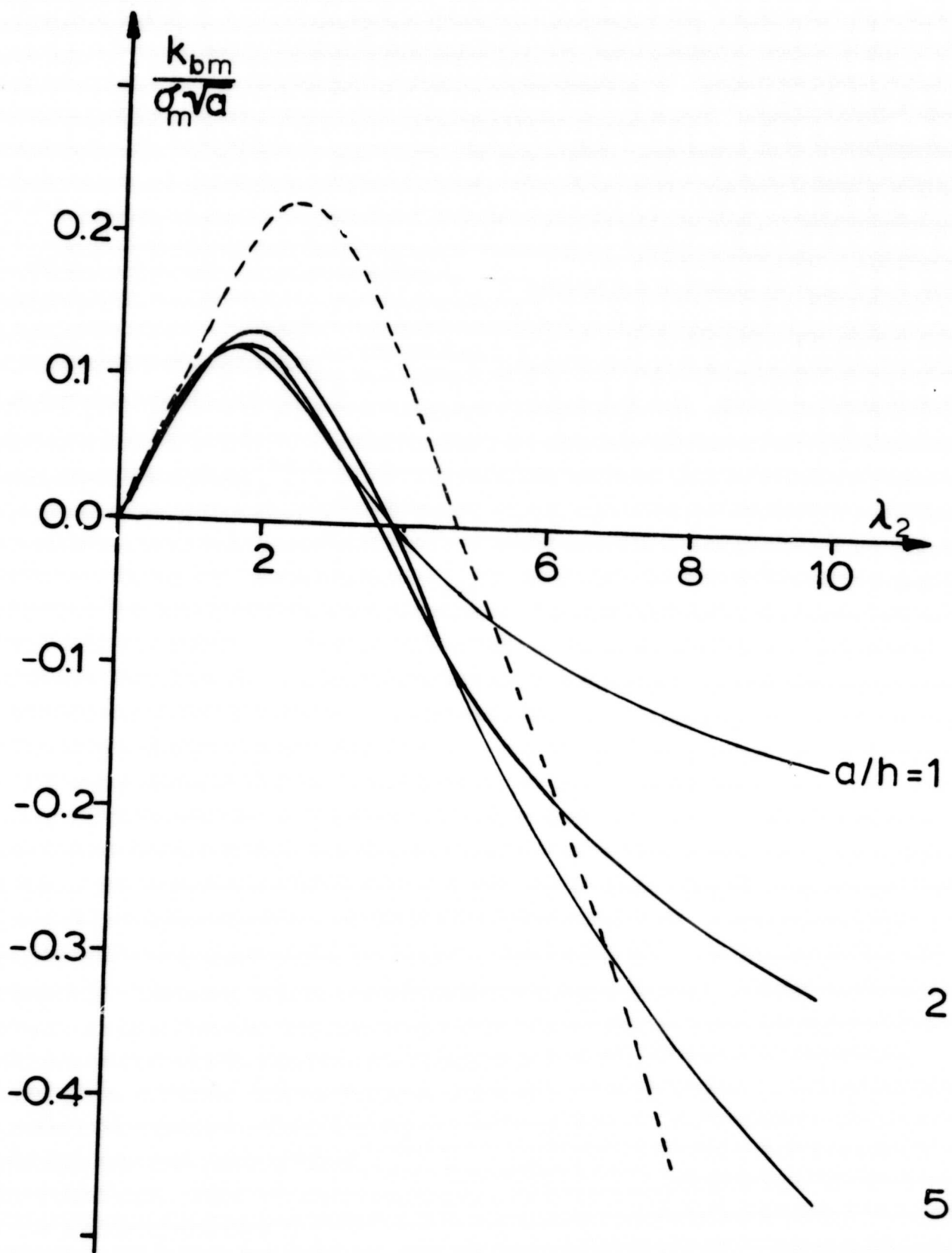
Figure 4 Bending component of the stress intensity factor ratio k_{bm} , N_{xx} \neq 0 , M_{xx} = 0
