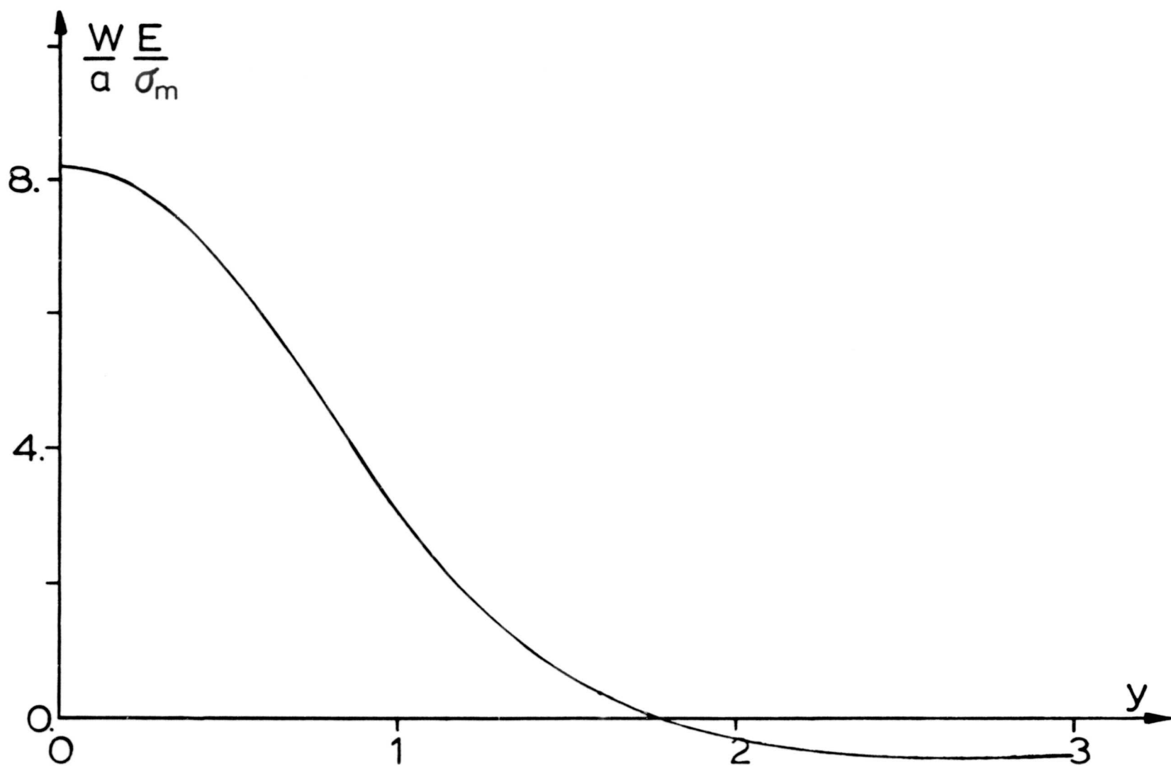
Figure 7 Displacement component perpendicular to the shell surface, w(0,y) . N_{xx} \neq 0 , M_{xx} = 0 , a/h = 5 , \lambda_2 = 4
