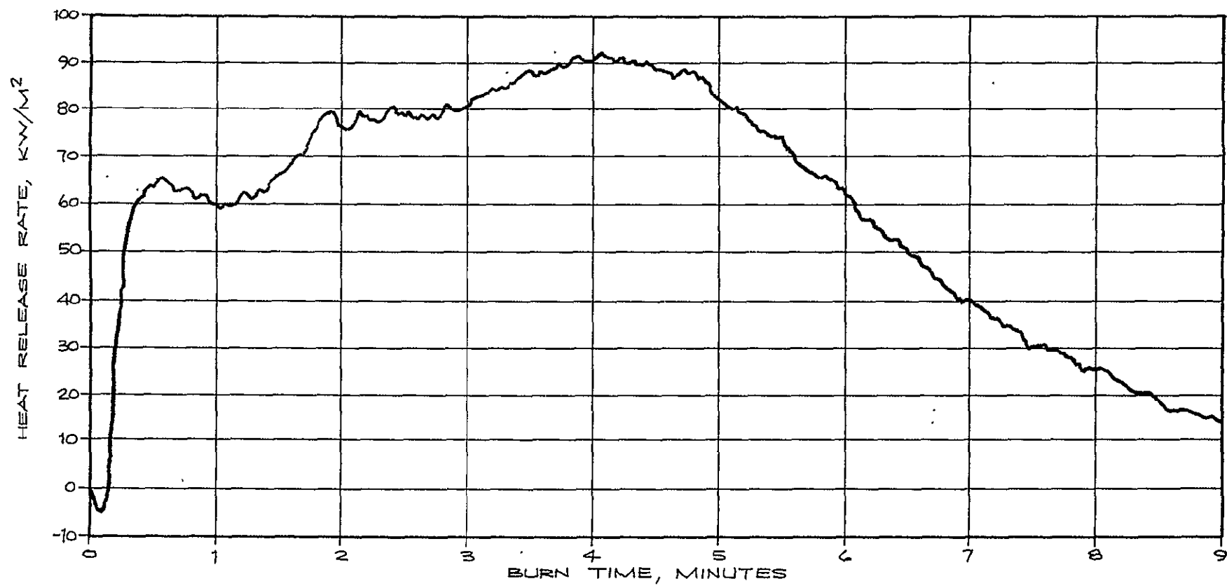
FIGURE 46. HEAT RELEASE RATE MATERIAL NO. 304
