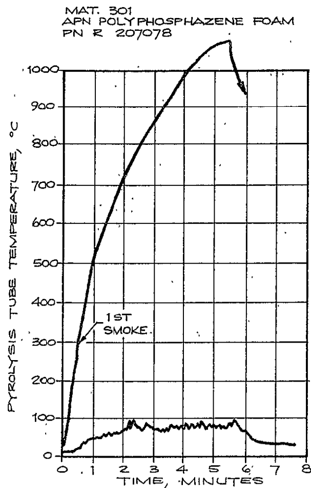
FIGURE 27. FLASH FIRE TC TRACE - (301)
