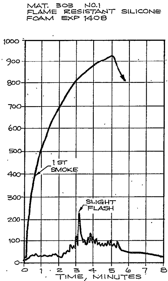
FIGURE 28. FLASH FIRE TC TRACE - (303) NO. 1
