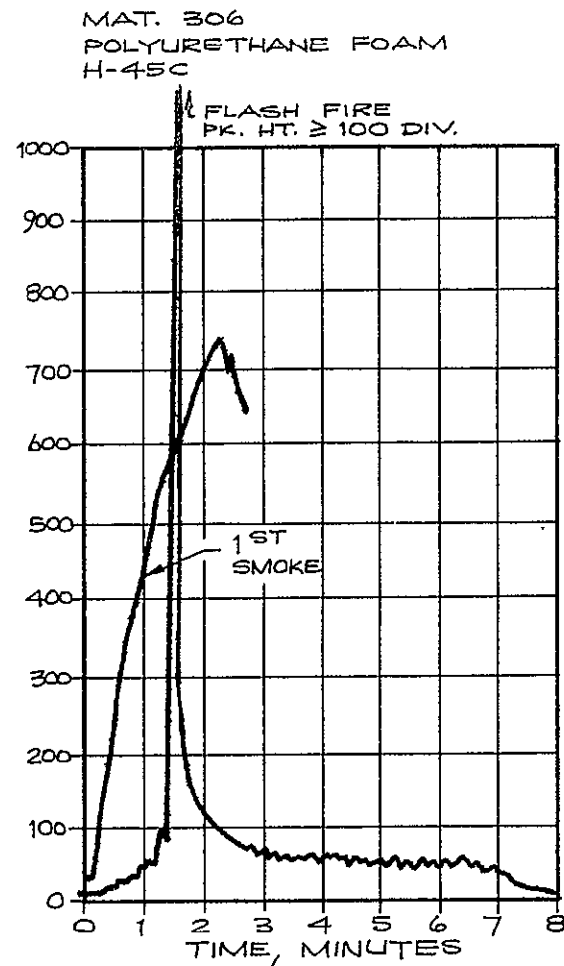
FIGURE 32. FLASH FIRE TC TRACE - (306)
