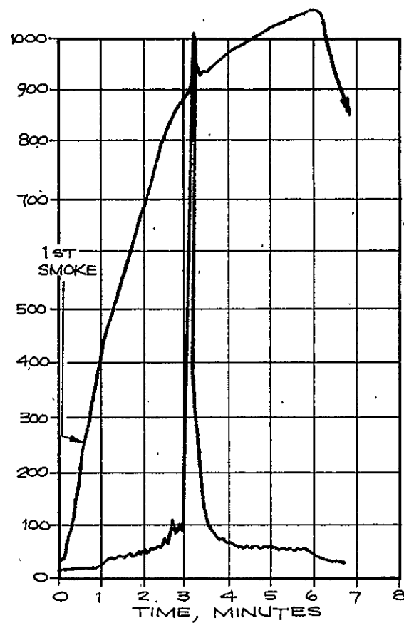
FIGURE 23. FLASH FIRE TC TRACE - (215)
