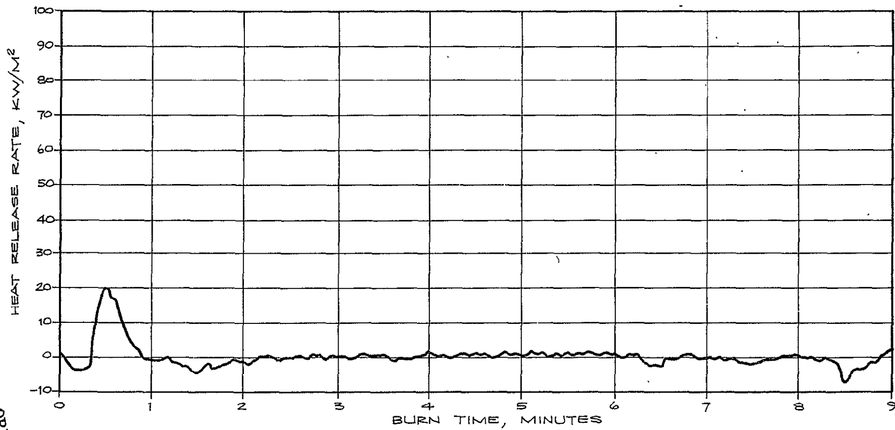
FIGURE 45. HEAT RELEASE RATE MATERIAL NO. 208
