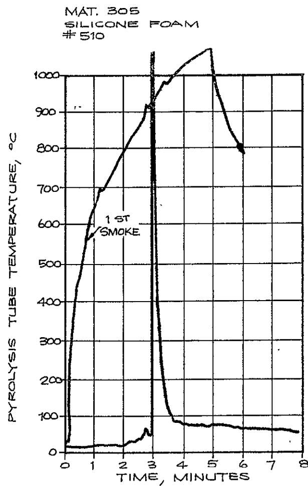
FIGURE 31. FLASH FIRE TC TRACE - (305)
