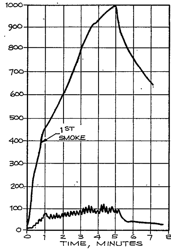
FIGURE 34. FLASH FIRE TC TRACE -(308)
