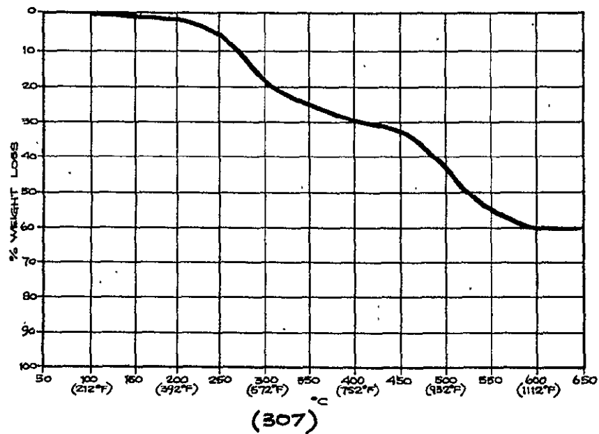
FIGURE 4. TGA RESULTS - CUSHIONING LAYERS (CONT'D)
