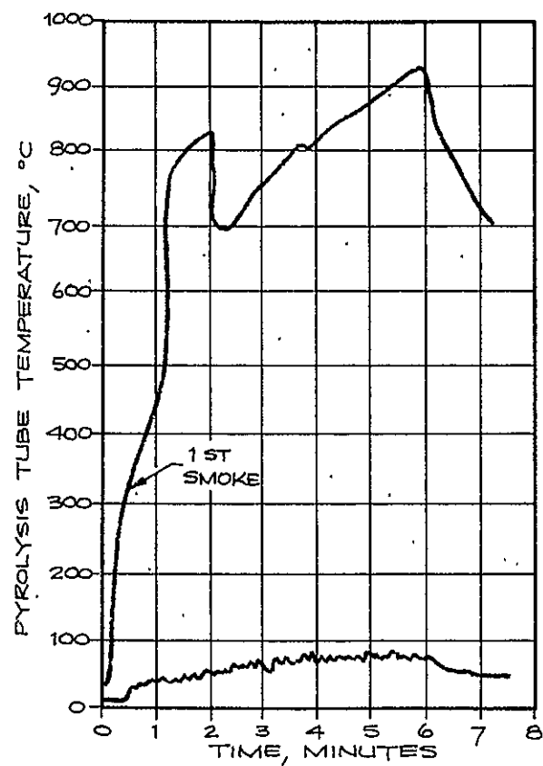
FIGURE 22. FLASH FIRE TC TRACE - (214)
