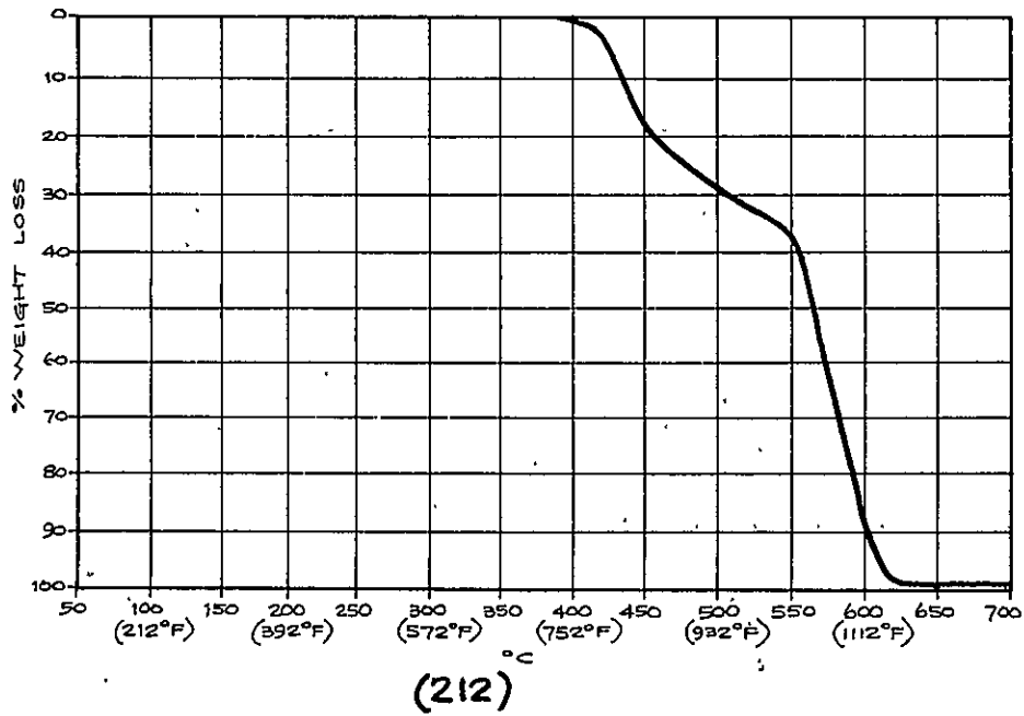
FIGURE 3. TGA RESULTS - FIRE BLOCKING LAYERS (CONT'D)
