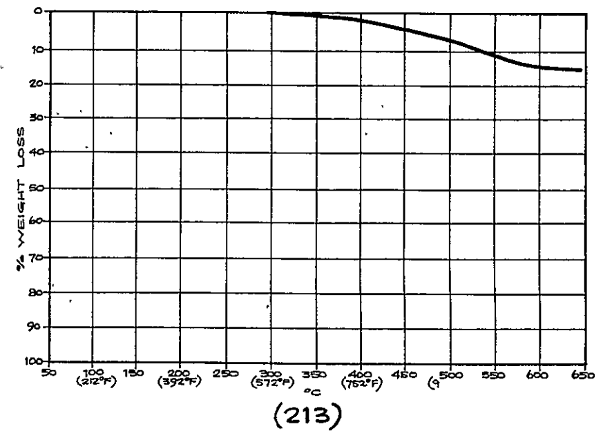
FIGURE 3. TGA RESULTS - FIRE BLOCKING LAYERS (CONT'D)
