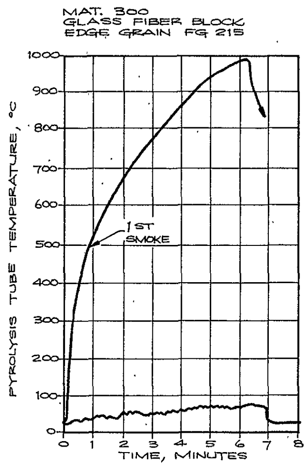
FIGURE 26. FLASH FIRE TC TRACE - (300)
