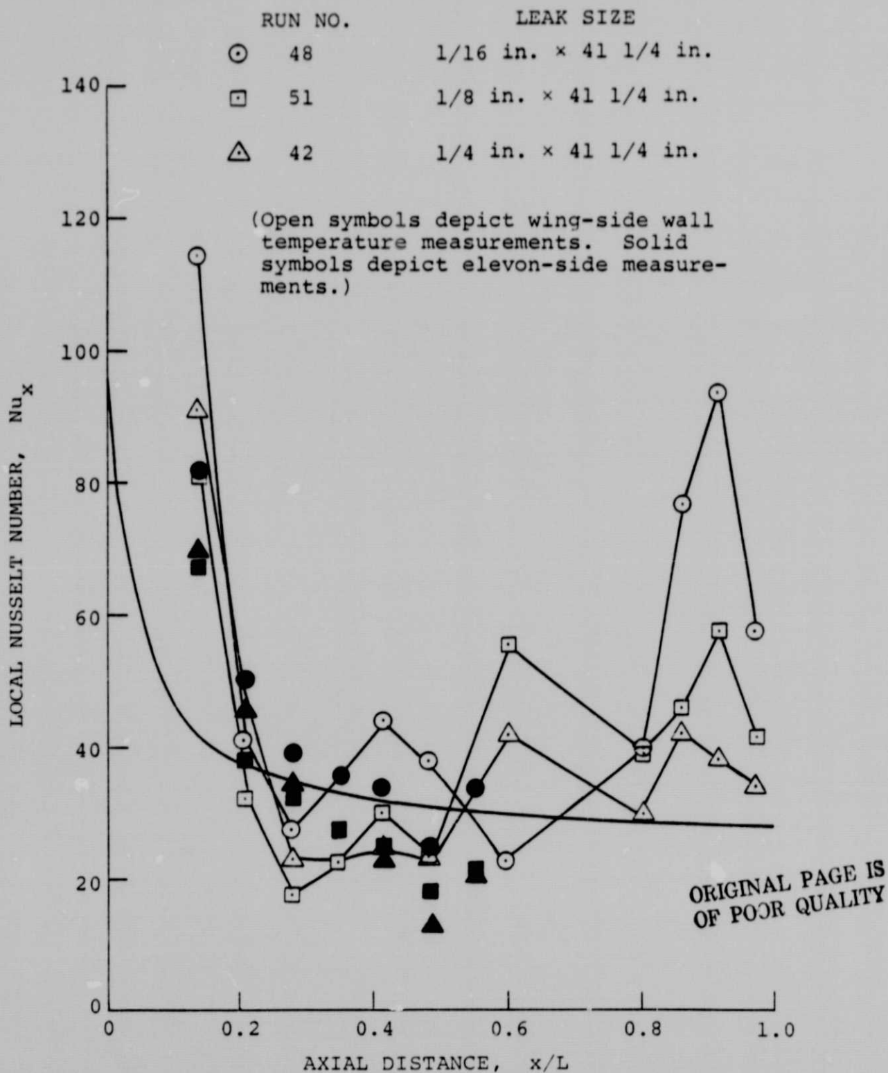
Figure 6. Local Nusselt numbers calculated from measured wall and gas temperatures in cove ("cold-wall" conditions) compared with computer model predictions based on laminar flow entrance conditions. T_{g,i} = 2.5 .
