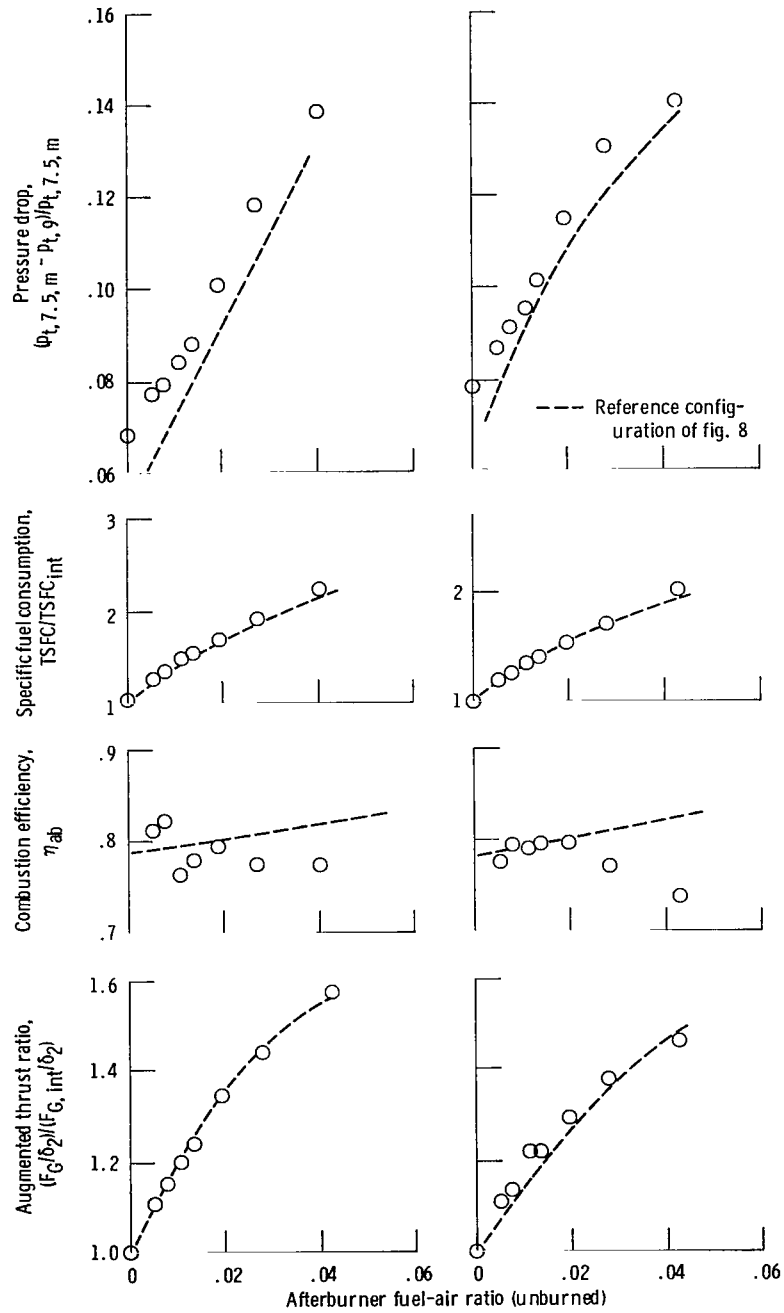
Figure 39. - Afterburner performance at two inlet temperatures. Configuration, carburetted flameholder II; Reynolds number index, 0.5; flameholder blockage, 37.9 percent.
