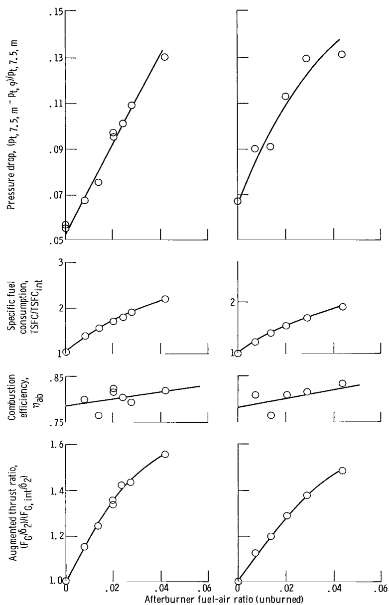
Figure 8. - Afterburner performance at two inlet temperatures. Configuration, reference TF30-P-3 afterburner; Reynolds index number, 0.5; flameholder blockage, 38.3 percent.
