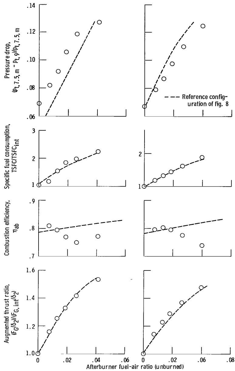
Figure 34. - Afterburner performance at two inlet temperatures. Configuration, carburetted flameholder I; Reynolds number index, 0.5; flameholder blockage, 35.1 percent.
