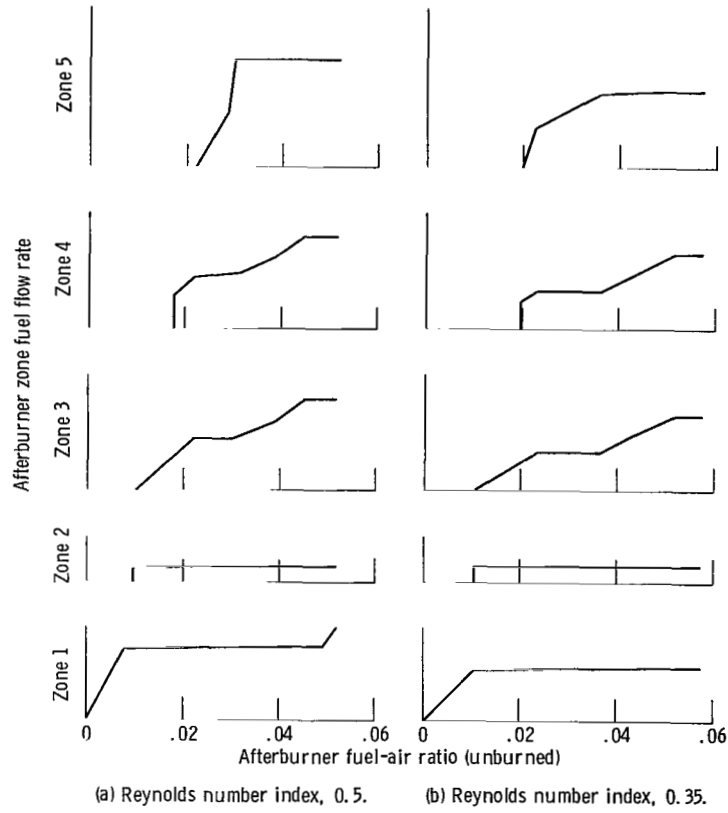
Figure 30. - Afterburner zone fuel flow distribution. Configuration, triple ring flameholder with swirl cans.
