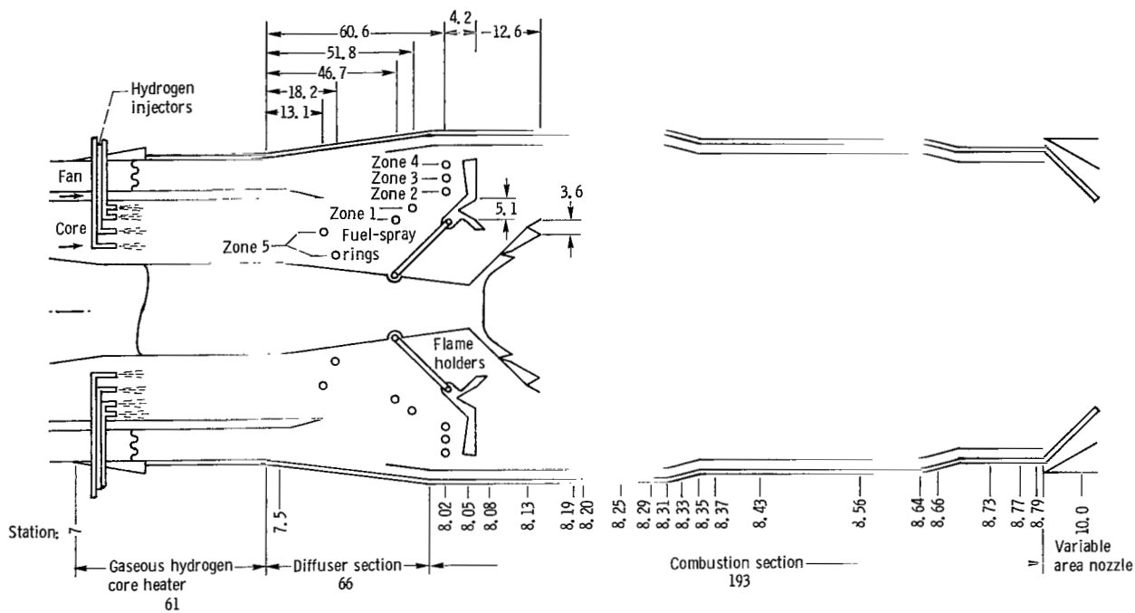
Figure 2. - Cross-sectional schematic of TF30-P-3 reference afterburner with instrumentation stations. All dimensions in centimeters.
