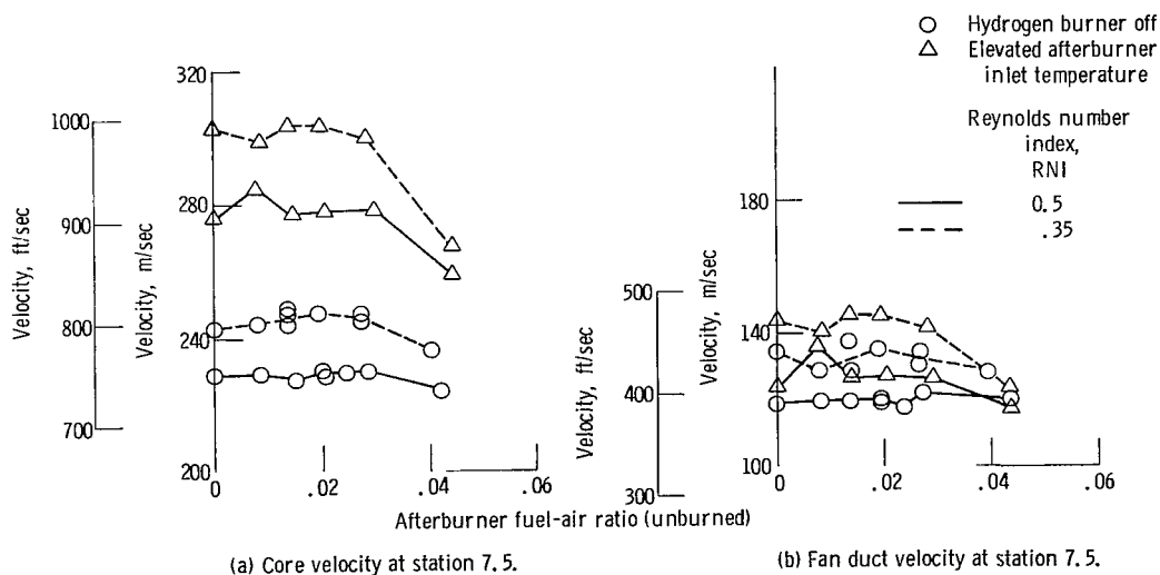
Figure 5. - Core and fan velocities at inlet to afterburner section. Configuration, reference TF30-P-3 afterburner.
