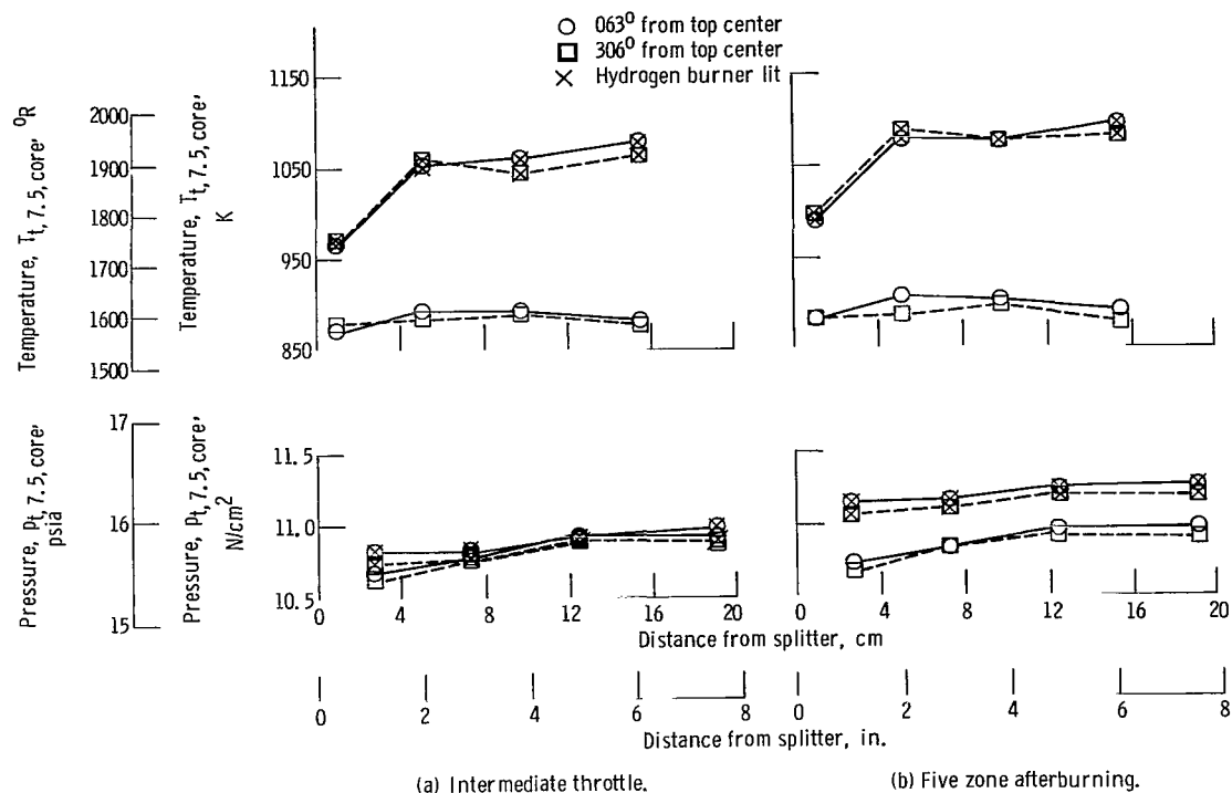
Figure 4. - Pressure and temperature profiles leaving hydrogen heater. Reynolds number index, RNI, 0.5.
