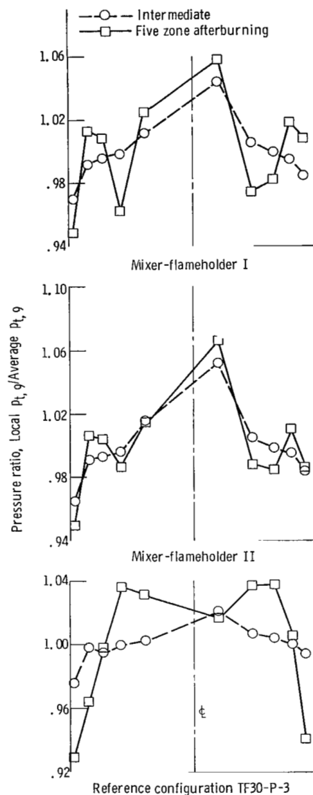
Figure 19. - Total pressure profile across duct at station 9. Reynolds number index, 0.5.
