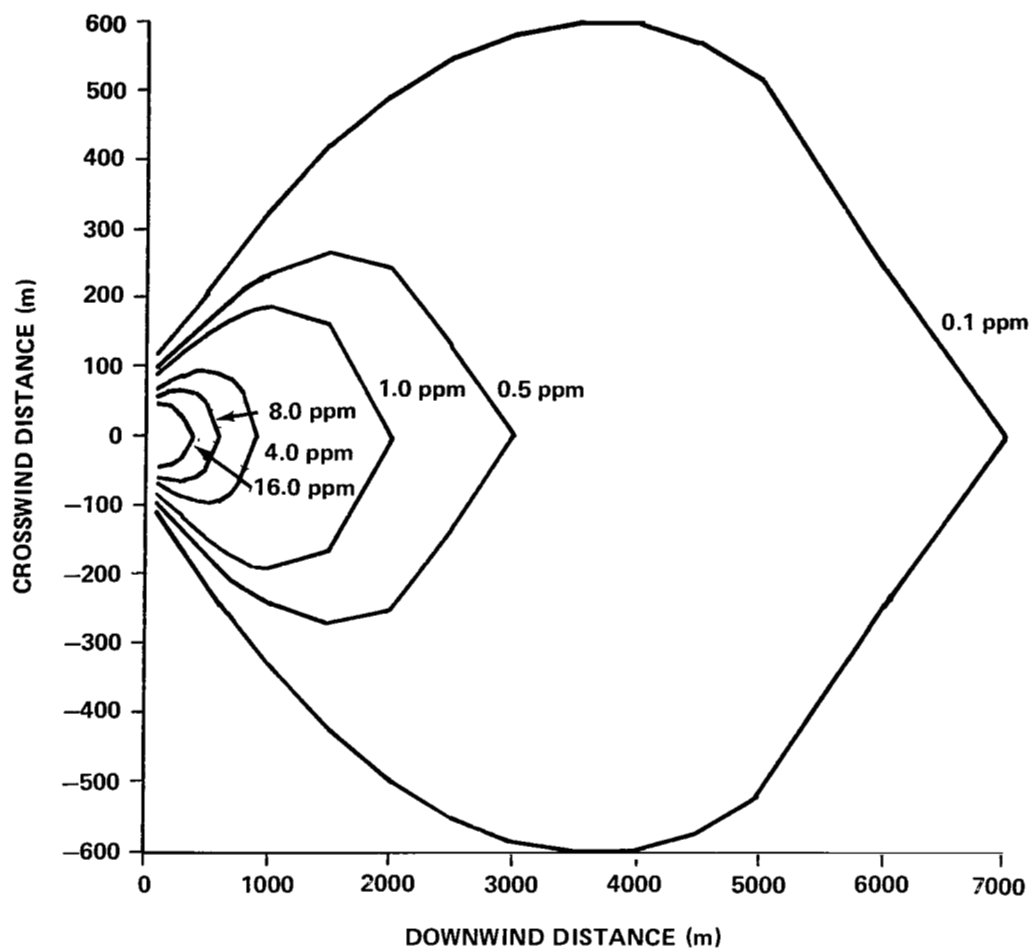
Figure 34. Computed HCl concentration isopleths by NASA/MSFC Multilayer Diffusion Model: Static Test No. 14 (height 2.0 m, azimuth bearing 354.3^\circ ).
