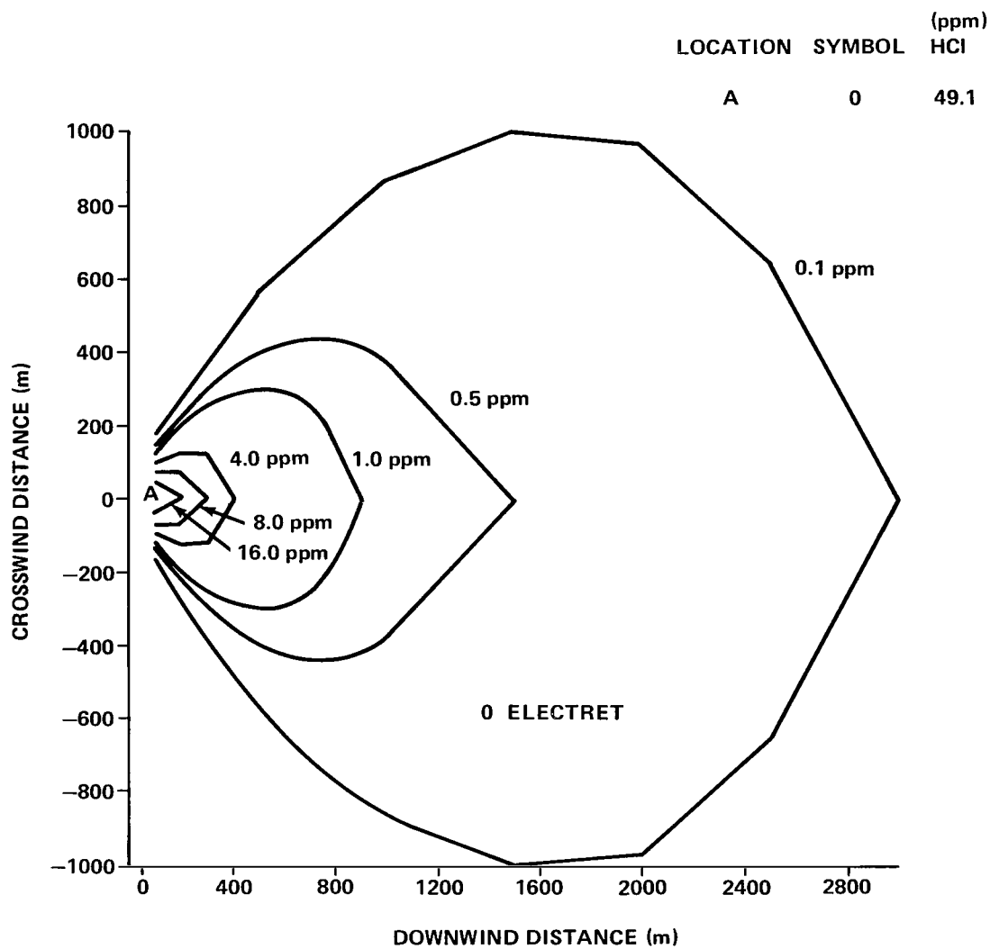
Figure 12. Comparison of HCl concentration isopleths computed by NASA/MSFC Multilayer Diffusion Model with measured values: Static Test No. 3 using Model 4 (height 2.0 m, azimuth bearing 333.6^\circ ).
