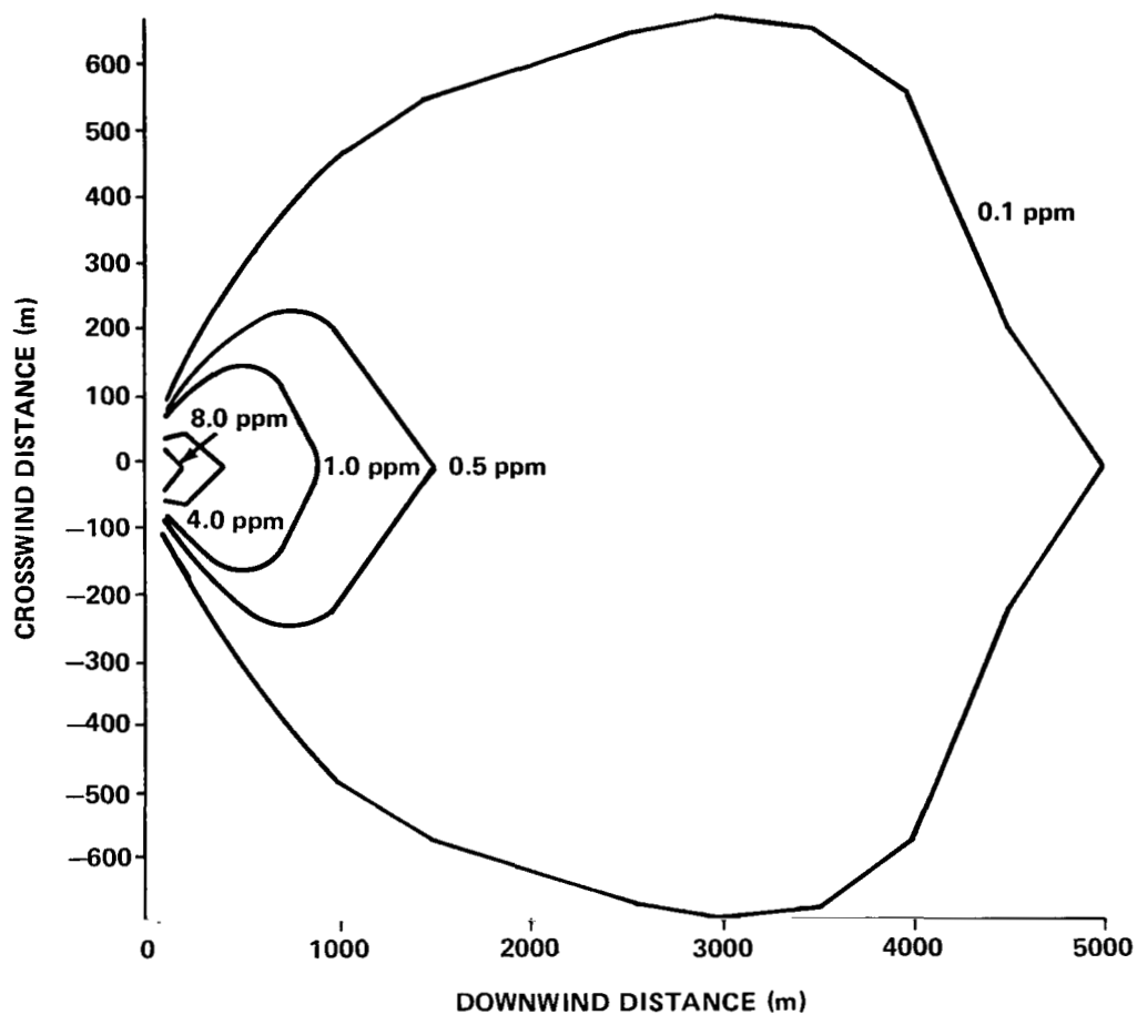
Figure 30. Computed HCl concentration isopleths by NASA/MSFC Multilayer Diffusion Model: Static Test No. 12 using Model 4 (height 2.0 m, azimuth bearing 328.6^\circ ).
