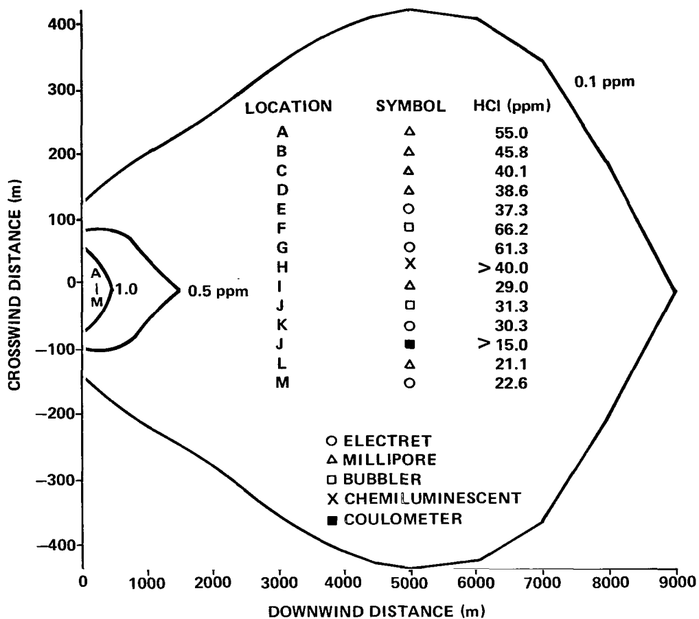
Figure 42. Comparison of HCl concentration isopleths computed by NASA/MSFC Multilayer Diffusion Model with measured values: Static Test No. 18 (height 2.0 m, azimuth bearing 122.7°).
