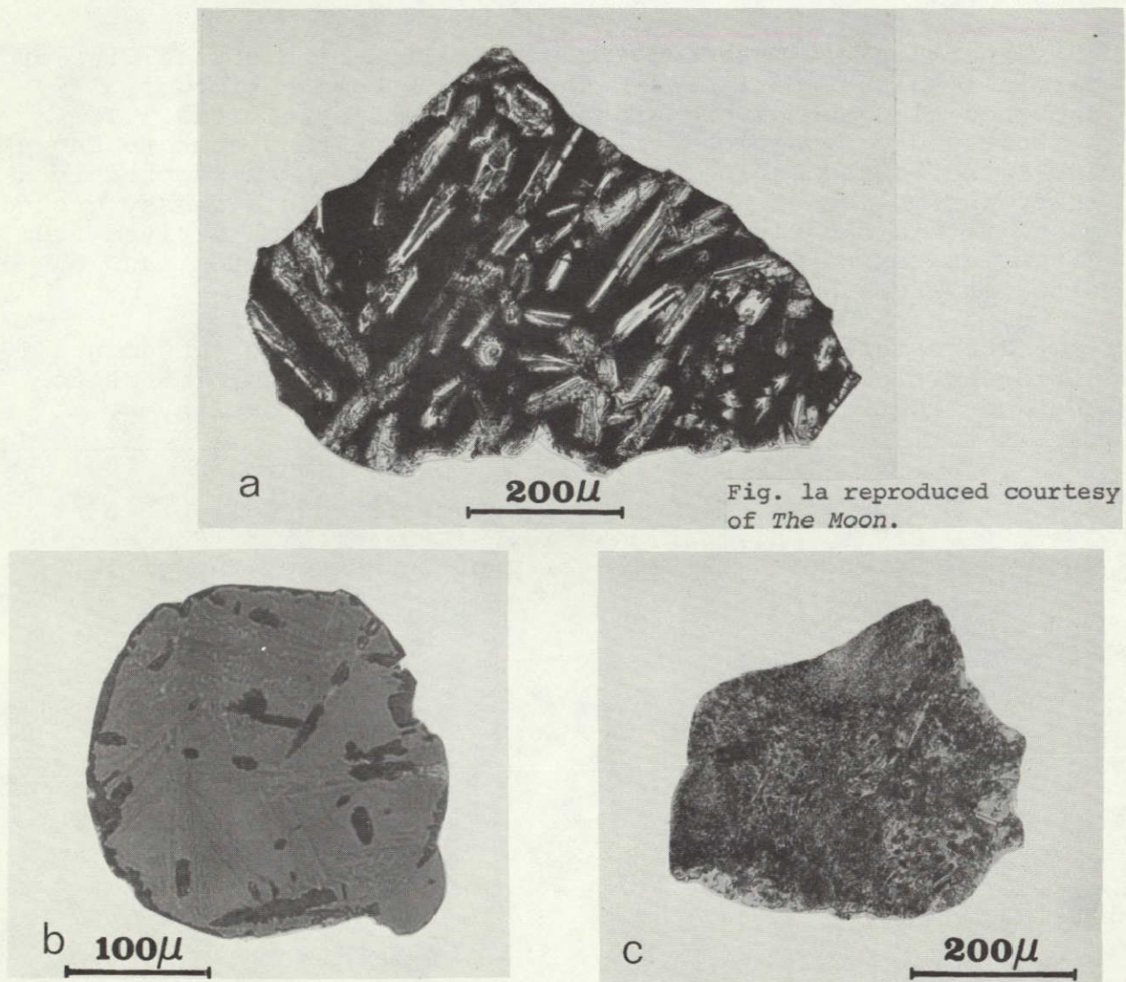
Figure 1. Three exotic particles from Luna 24 sample 24149. a. Olivine vitrophyre. (Transmitted light.) b. Devitrified Ti-rich glass spherule. (Reflected light.) c. Anorthositic gabbro: shock-melted and partially recrystallized. The larger dark specks are cavities, not opaque minerals. (Transmitted light.)
