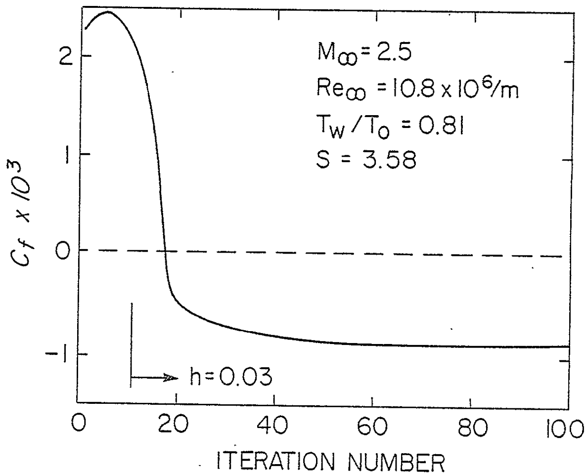
Figure 3A CONVERGENCE PROPERTY OF SKIN FRICTION
