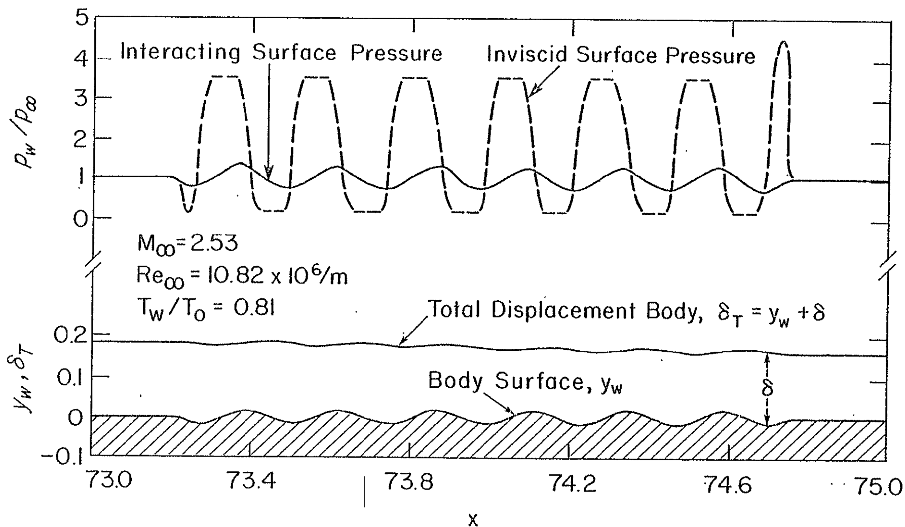
Figure 4 DISPLACEMENT BODY AND SURFACE PRESSURE - STANDARD CASE
