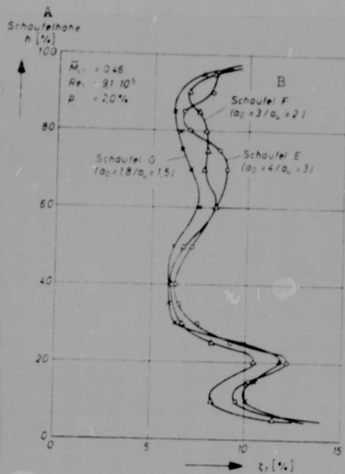
Figure 12 - Effect of the distance of the blow holes from the wall on the blade loss coefficient
