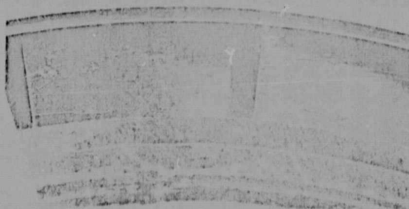
Figure 9 - View of the profile suction sides of turbine guide blades with visualized flow lines of the wall boundary layers with and without air blown onto the blades, M_{cl} = 0.45
