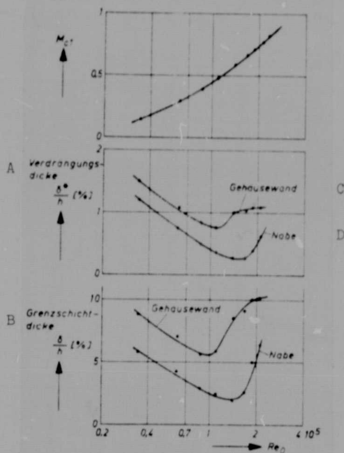
Figure 13 - Boundary layer formation in the oncoming flow as a function of the Reynolds number
