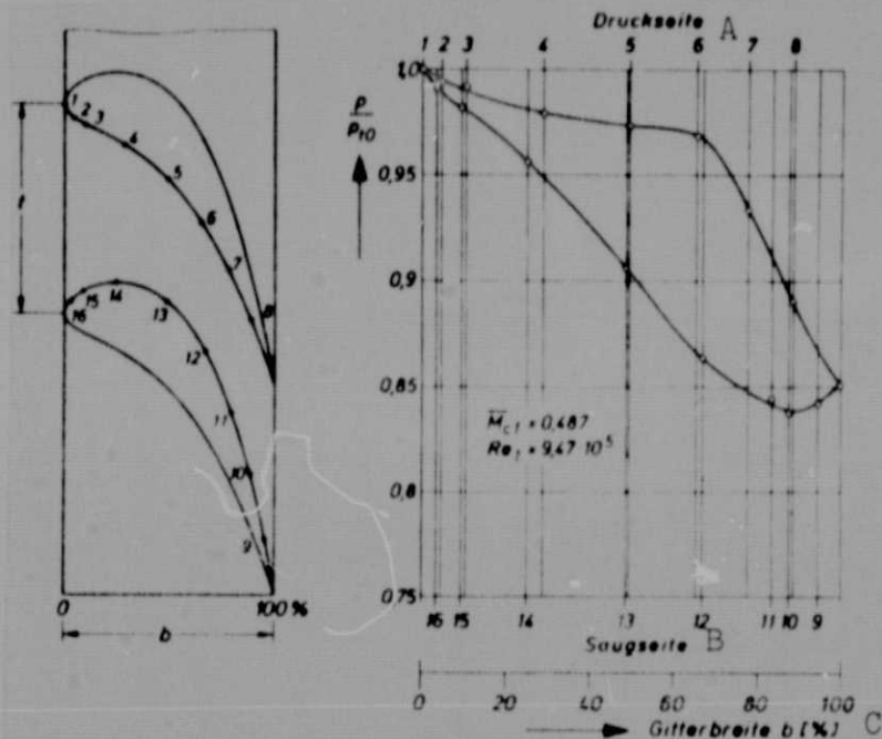
Figure 4 - Pressure distribution for the central section of the turbine guide blade channel at \bar{M}_{cl} = 0.487
