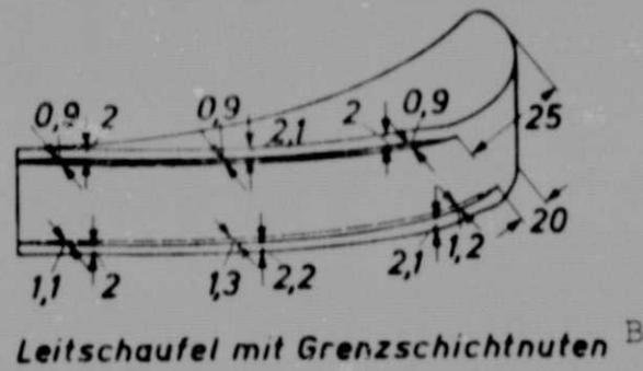
Figure 6 - Location of the blow holes and boundary layer groove dimensions according to [2]
