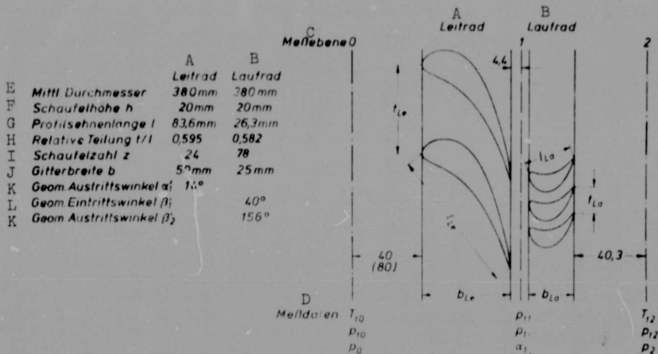
Figure 2 - Characteristic data for the turbine stage
