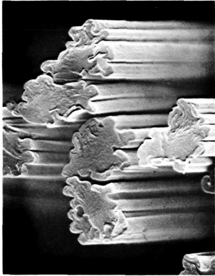
THORNEL 75 GRADE WYL 160
