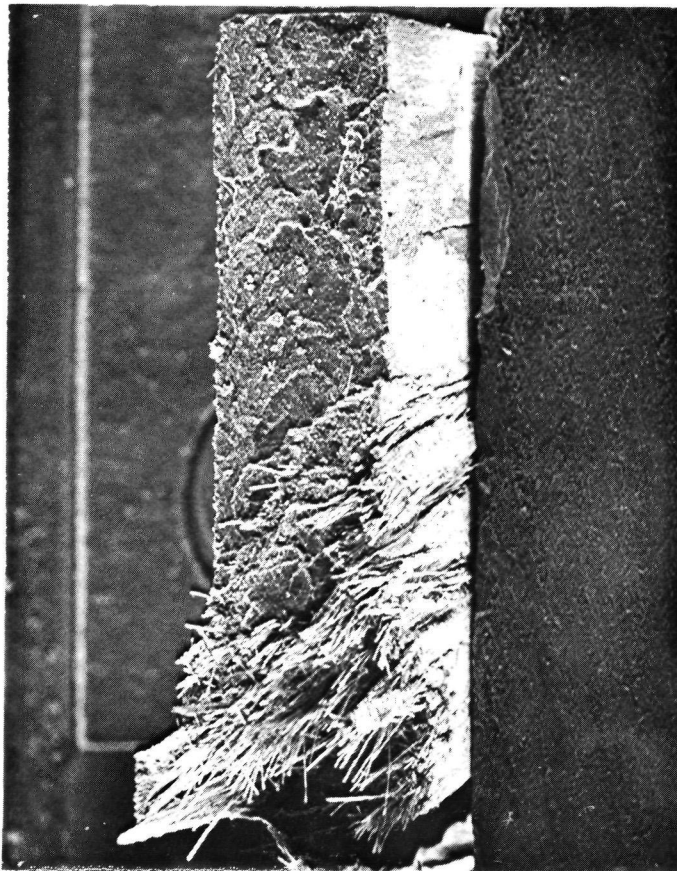
SCANNING ELECTRON MICROGRAPH OF FRACTURED SURFACE OF LB97-L2, 410 MPa (59.6 ksi) 1100°C PREPARATION
