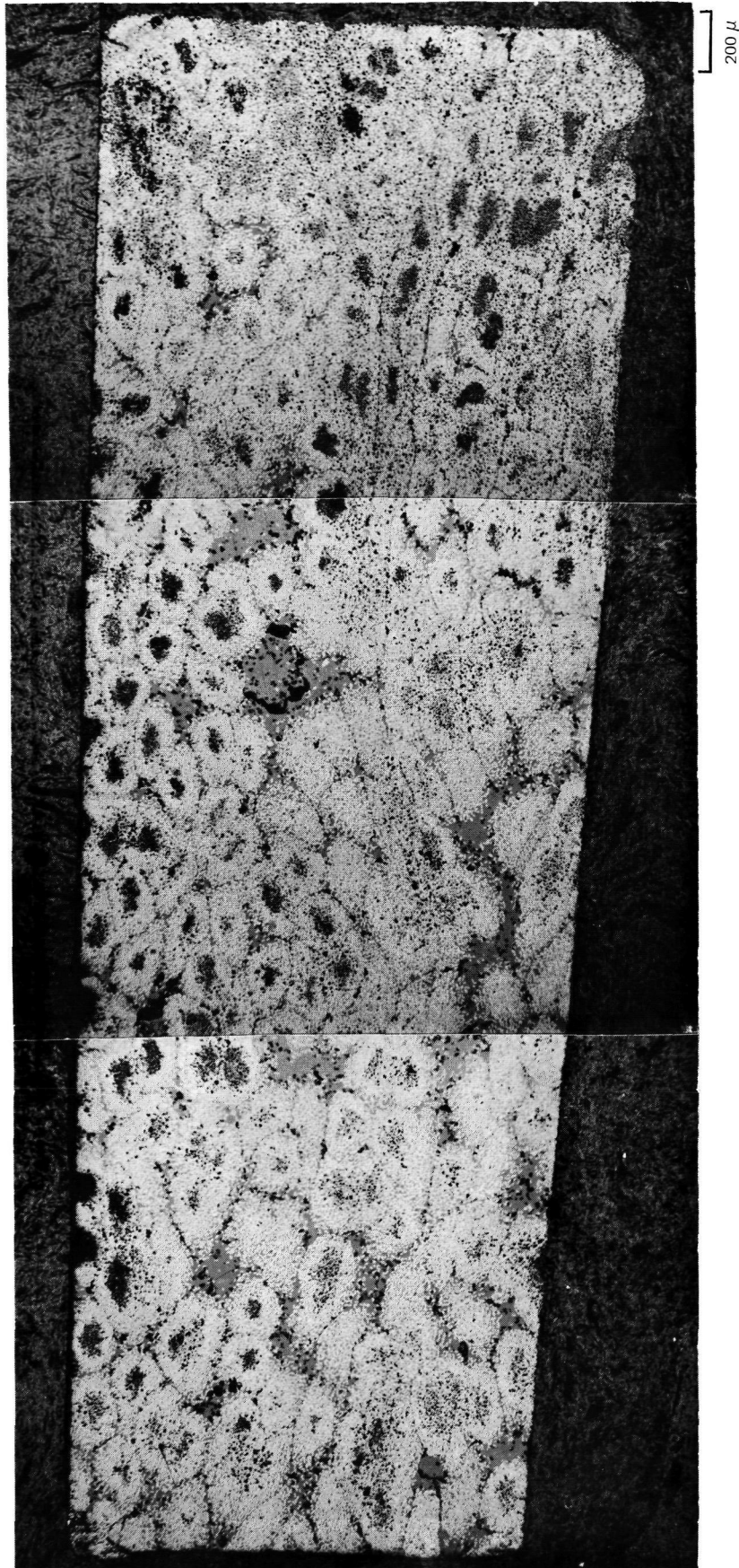
TAPE-MAP OF UNFRACTURED SAMPLE LB96 CELANESE DG-102 FIBER, 7740 GLASS MATRIX, HOT PRESSED AT 1075 °C
