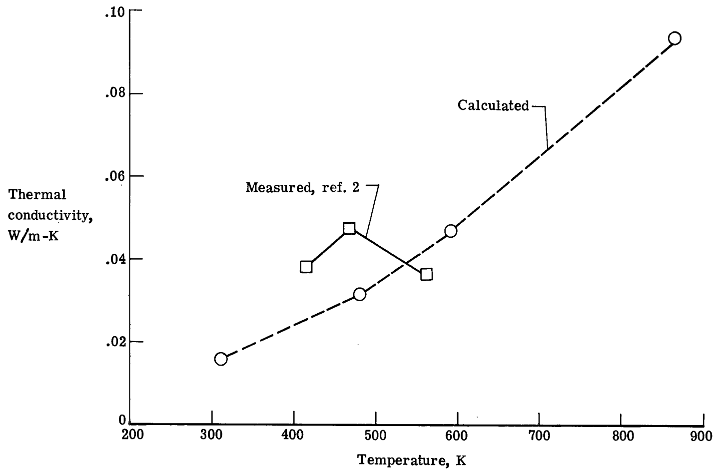
Figure 11.- Comparison of measured and calculated polyimide-foam thermal conductivity.
