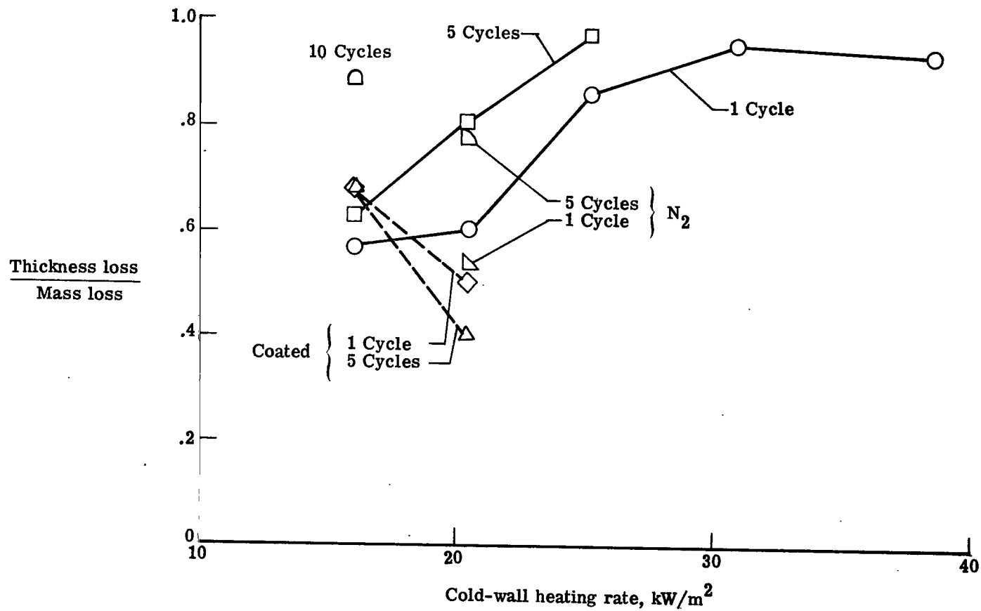
Figure 9.- Change in thickness-loss to mass-loss ratio as function of cold-wall heating rate and number of cycles.
