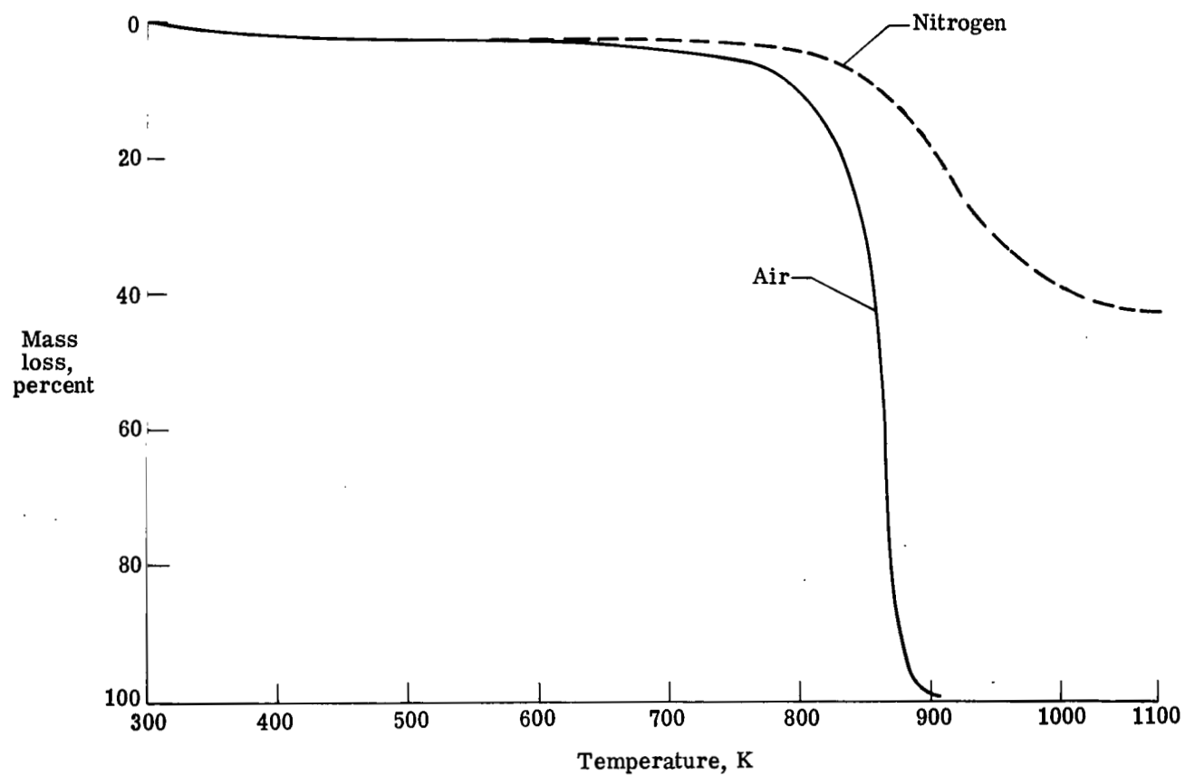
Figure 4.- TGA curve for polyimide foam. Temperature-rise rate = 2.5 K/min.
