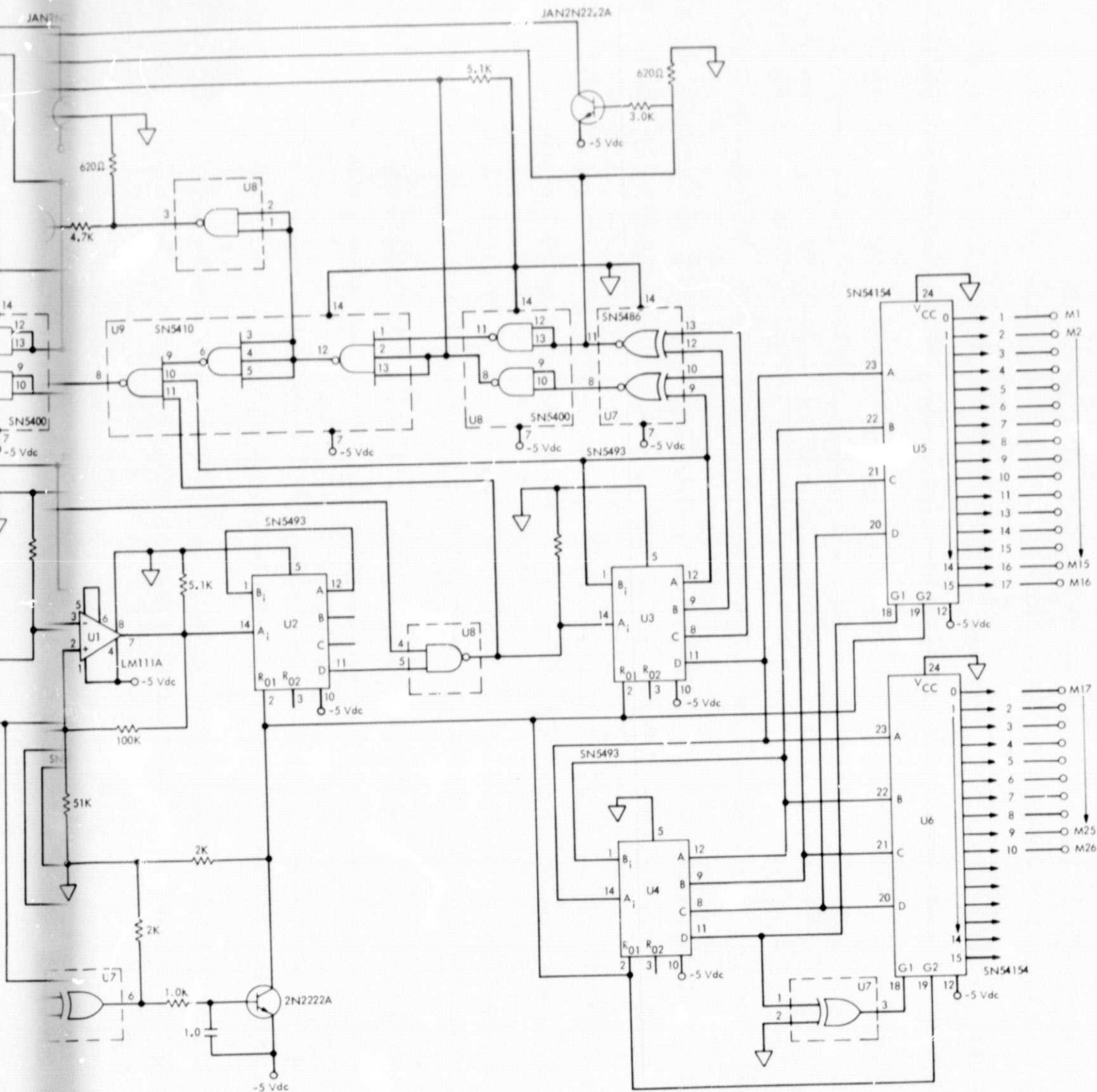
Figure 5-3. Multiplexer Schematic (MUX, B2)
