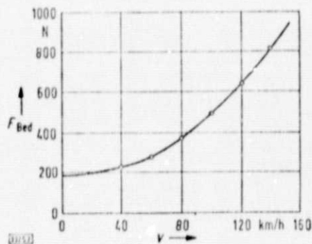
Fig. 2. Road resistance F_{Bed} = F_R + F_L of the sample vehicle (passenger car) as a function of the velocity v of the car on a level plane.
