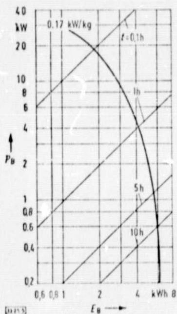
Fig. 5. Battery output as a function of energy removal with the discharge time t as the parameter for a specific output of 0.17 kW/kg.
