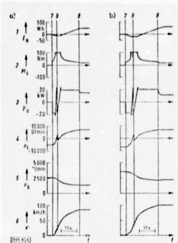
Fig. 8. Different events represented by an analog computer. a) from 0 to 80 km per hour with an initial speed of the i.c. engine n_O = 2500 rpm, b) from 0 to 100 km per hour with an initial speed of n_O = 3350 rpm.
