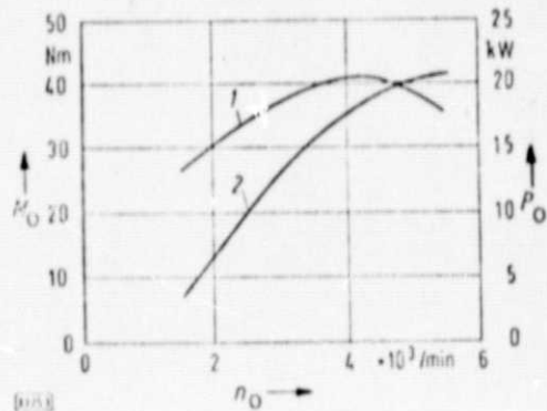
Fig. 3. Maximum torque and maximum power of the internal combustion engine as a function of rpm.
