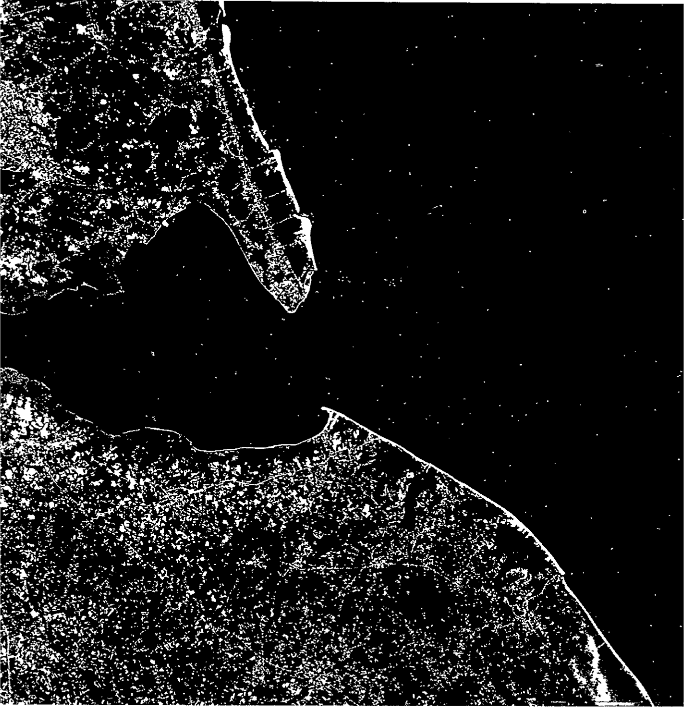
Figure 4.1 Skylab/EREP color photograph of the Delaware Bay region obtained with the S190A multispectral photographic facility on September 12, 1973
