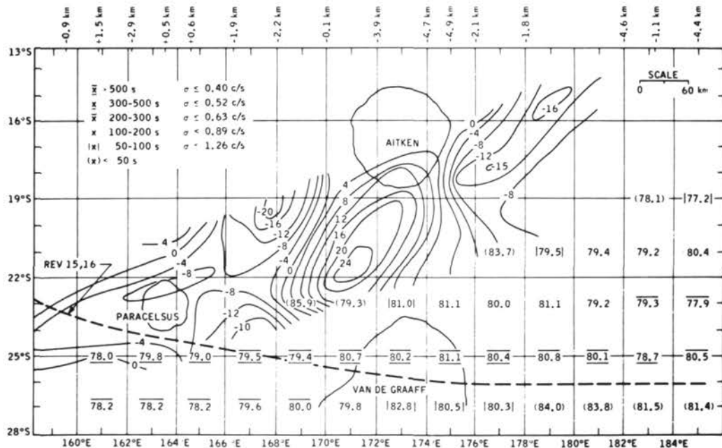
Figure 8.—The region around the crater Van de Graaff, showing the altitude-corrected, gamma-ray intensities between 0.55 MeV and 2.75 MeV in 2- by 2-degree areas, the location of the laser altimeter ground track with elevation given at the top, and a contour map of the lunar contribution to the solar-directed component of the magnetic field from an elevation of 67 km. The subsatellite magnetometer values are in tenths of gammas. The insert gives the coding which represents the observation time within the 2- by 2-degree area, and the maximum 1\sigma standard deviation corresponding to that period.
