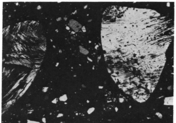
Figure 16.—Photomicrograph of glass-rich light-gray breccia 73215. (Width of field of view is 2.2 mm; crossed polarizers.) Two large rounded grains of partly recrystallized shock-deformed plagioclase are included within the dark aphanitic matrix.
