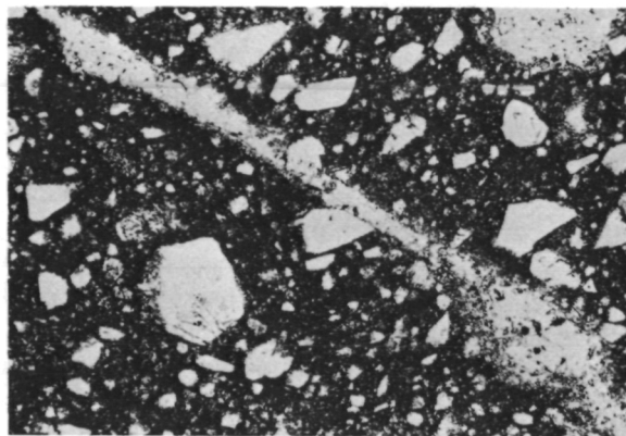
Figure 9.—Photomicrograph of dark material in thermally metamorphosed breccia 12013. (Width of field of view is 2.2 mm; plane-polarized light.) As in light-gray breccia 73255 (see fig. 5), most clasts are of single mineral grains, and fragments and groundmass have the appearance of being two distinct materials. Fragment sizes are similar to those in 73255, and the fragments show rough planar preferred orientation (NE. to SW.). This rock is unusually rich in material of the composition of lunar "granite" and a veinlet of such material cuts the field of view (NW. to SE.).
