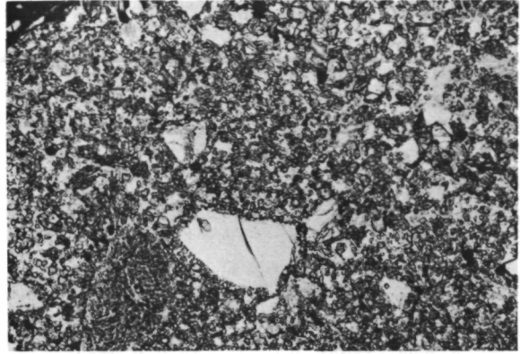
Figure 18.—Photomicrograph of hornfels clast in glass-rich light-gray breccia 73215. (Width of field of view is 2.2 mm; plane-polarized light.) The rock consists of a very fine grained recrystallized granoblastic matrix that contains xenocrysts (such as the angular one of plagioclase below center) and small xenoliths (such as the oval one to the left of the prominent plagioclase xenocryst).
