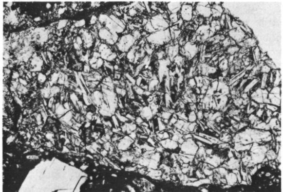
Figure 19.—Photomicrograph of clast of fine-grained basaltic-textured "troctolite" in glass-rich light-gray breccia 73215. (Width of field of view is 2.2 mm; plane-polarized light.) Plagioclase grains are lath-shaped, and olivine grains are roughly equant. A few partly resorbed phenocrysts of aluminous spinel are present (dark-gray skeletal grains near top left and bottom left of clast).
