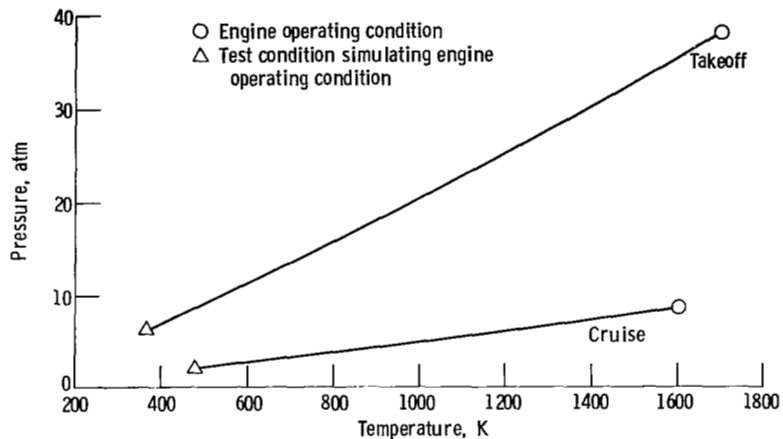
Figure 4. - Similarity curves for combustion-gas environments of advanced turbofan engine at takeoff and at cruise.
