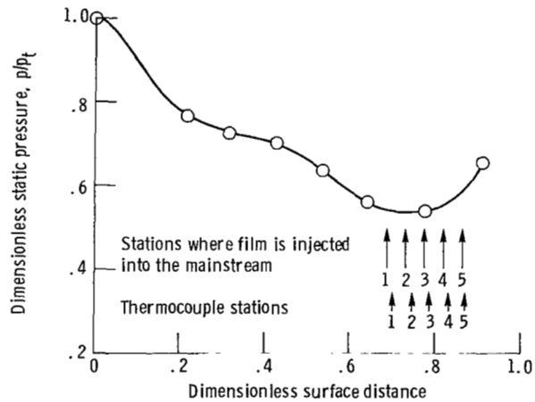
Figure 5. - Experimental midspan distribution of vane suction-surface pressure ratios obtained from cascade tests.
