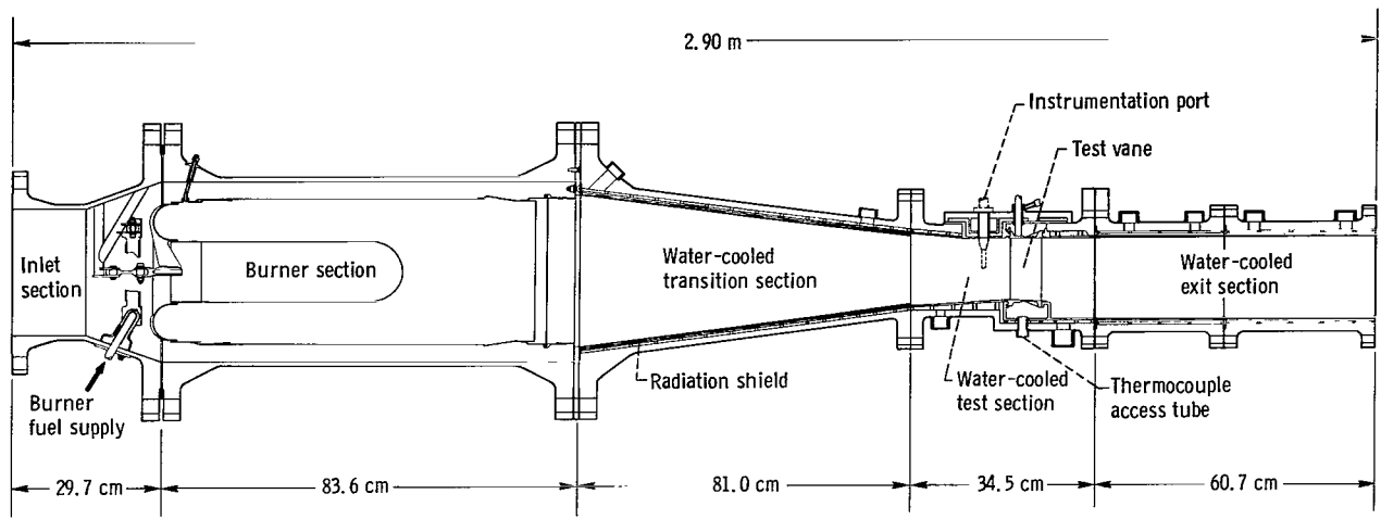
(a) Cascade facility.
