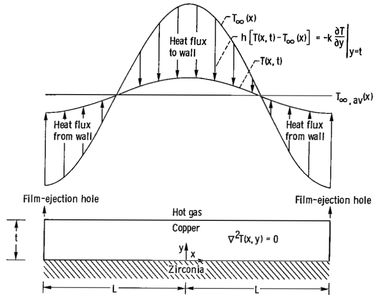
Figure 7. - Coordinate system and heat flux boundary condition for an insulated copper strip inserted into a film cooled wall.
