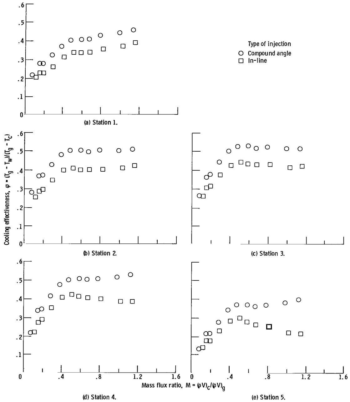
Figure 6. - Cooling effectiveness for film injection from in-line angle holes and compound-angle holes.
