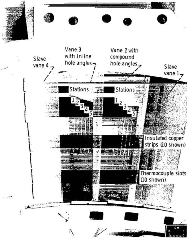
Figure 2. - Four-vane cascade with location of insulated copper strips on test vanes shown.
