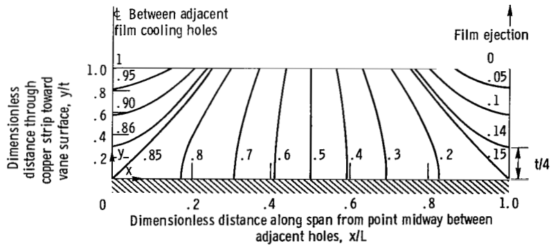
Figure 8. - Dimensionless isotherms within copper strip normalized by hottest and coldest surface temperatures.
