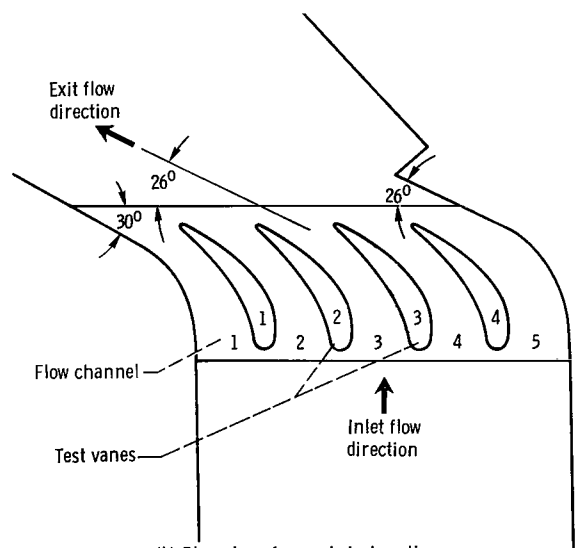
(b) Plan view of cascade test section.
