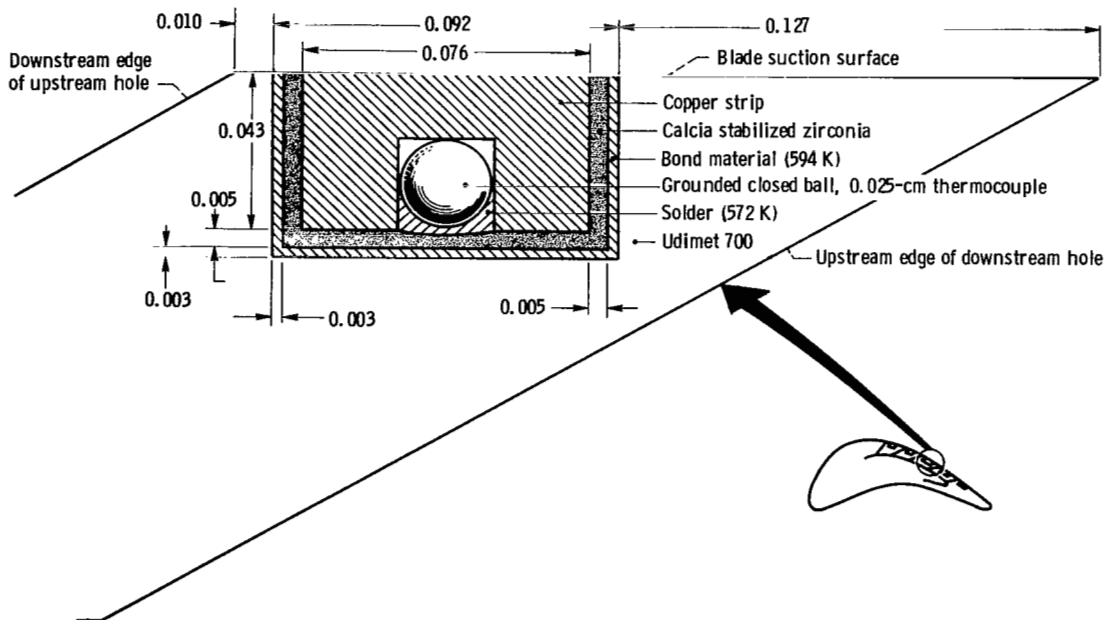
Figure 3. - Details of location and installation of thermocouple assembly. (All dimensions are in cm.)
