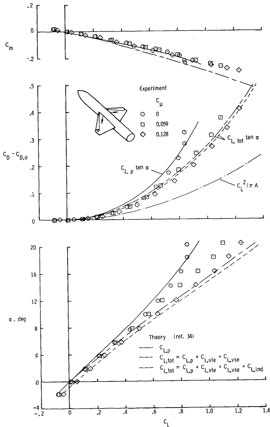
Figure 7.- Comparison of theoretical and experimental longitudinal aerodynamic characteristics of 44° swept trapezoidal wing configuration with \delta_{le} = \delta_{te} = 0^\circ ; M_\infty \approx 0.30 .
