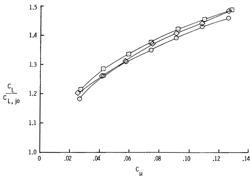
Figure 22.- Effect of C_\mu and \delta_{te} on lift augmentation ratio and lift effectiveness of blowing for 44° swept trapezoidal wing configuration; \delta_{le} = 0^\circ ; M_\infty = 0.30 ; \alpha \approx 21^\circ .
