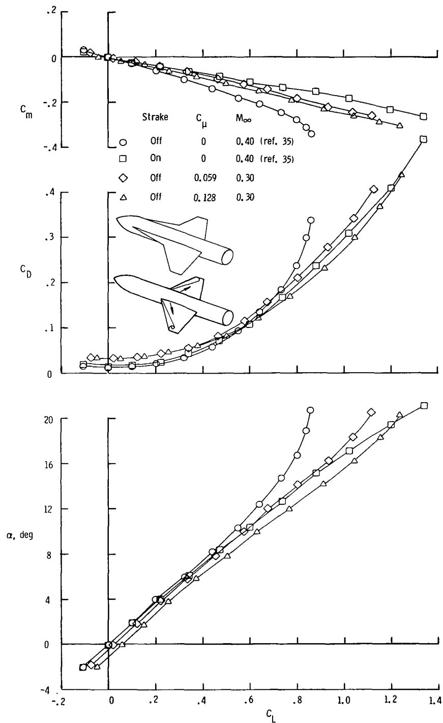
Figure 11.- Effect of wing strake and spanwise blowing on longitudinal aerodynamic characteristics of 44° swept trapezoidal wing configuration. \delta_{le} = 0^\circ .
