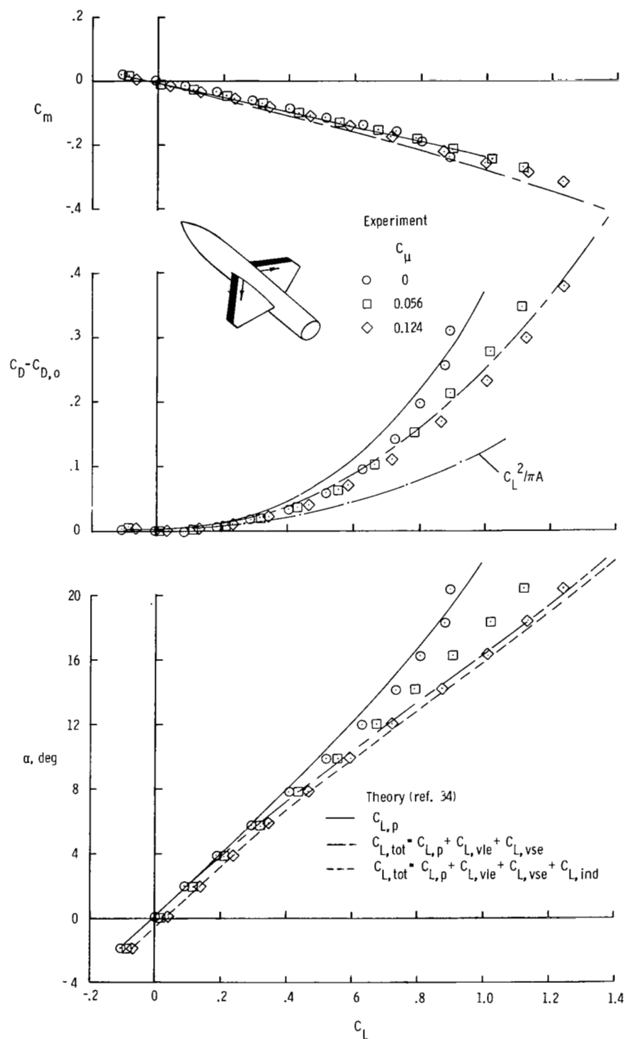
Figure 12.- Comparison of effect of spanwise blowing on theoretical and experimental longitudinal aerodynamic characteristics of 44° swept trapezoidal wing configuration with \delta_{le} = 4^\circ ; \delta_{te} = 0^\circ ; M_\infty = 0.30 .
