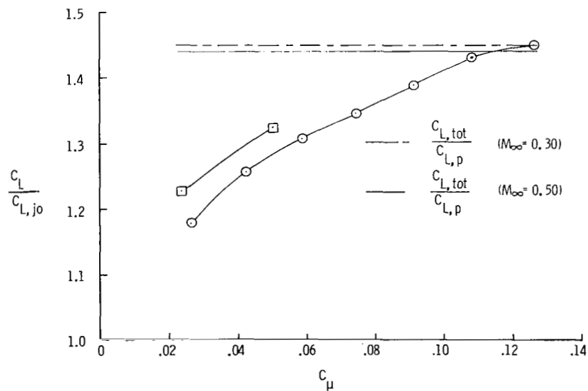
Figure 9.- Effect of C_{\mu} and M_\infty on lift augmentation ratio and lift effectiveness of blowing for 44° swept trapezoidal wing configuration for \alpha \approx 21^\circ .
