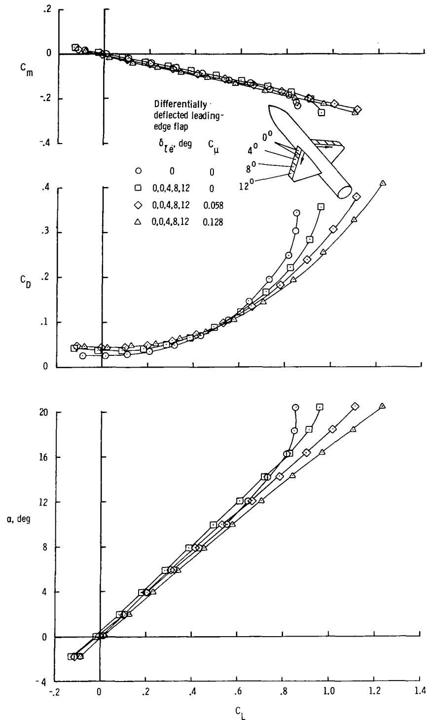
Figure 14.- Effect of spanwise blowing in conjunction with differentially deflected leading-edge flap on longitudinal aerodynamic characteristics of 44^\circ swept trapezoidal wing configuration; \delta_{te} = 0^\circ ; M_\infty = 0.30 .
