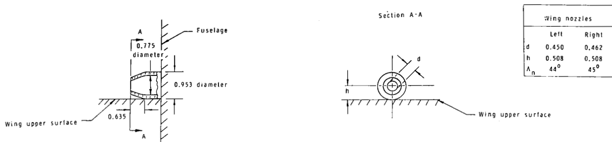
(a) Wing nozzle.
