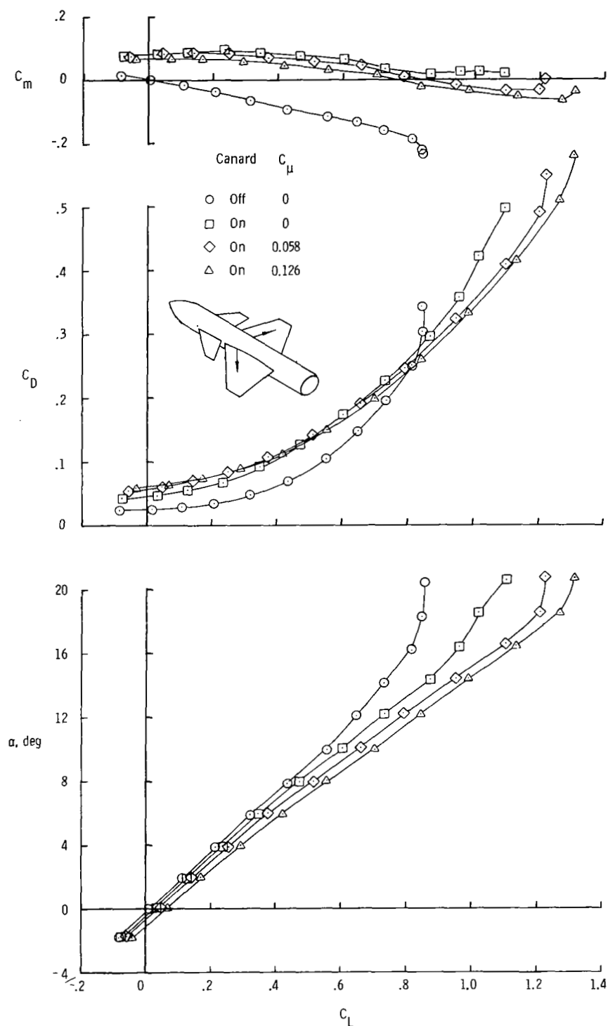
Figure 32.- Effect of spanwise blowing on 44^\circ swept trapezoidal wing on longitudinal aerodynamic characteristics of close-coupled canard wing configuration for i_C = 10^\circ ; M_\infty = 0.30 .
