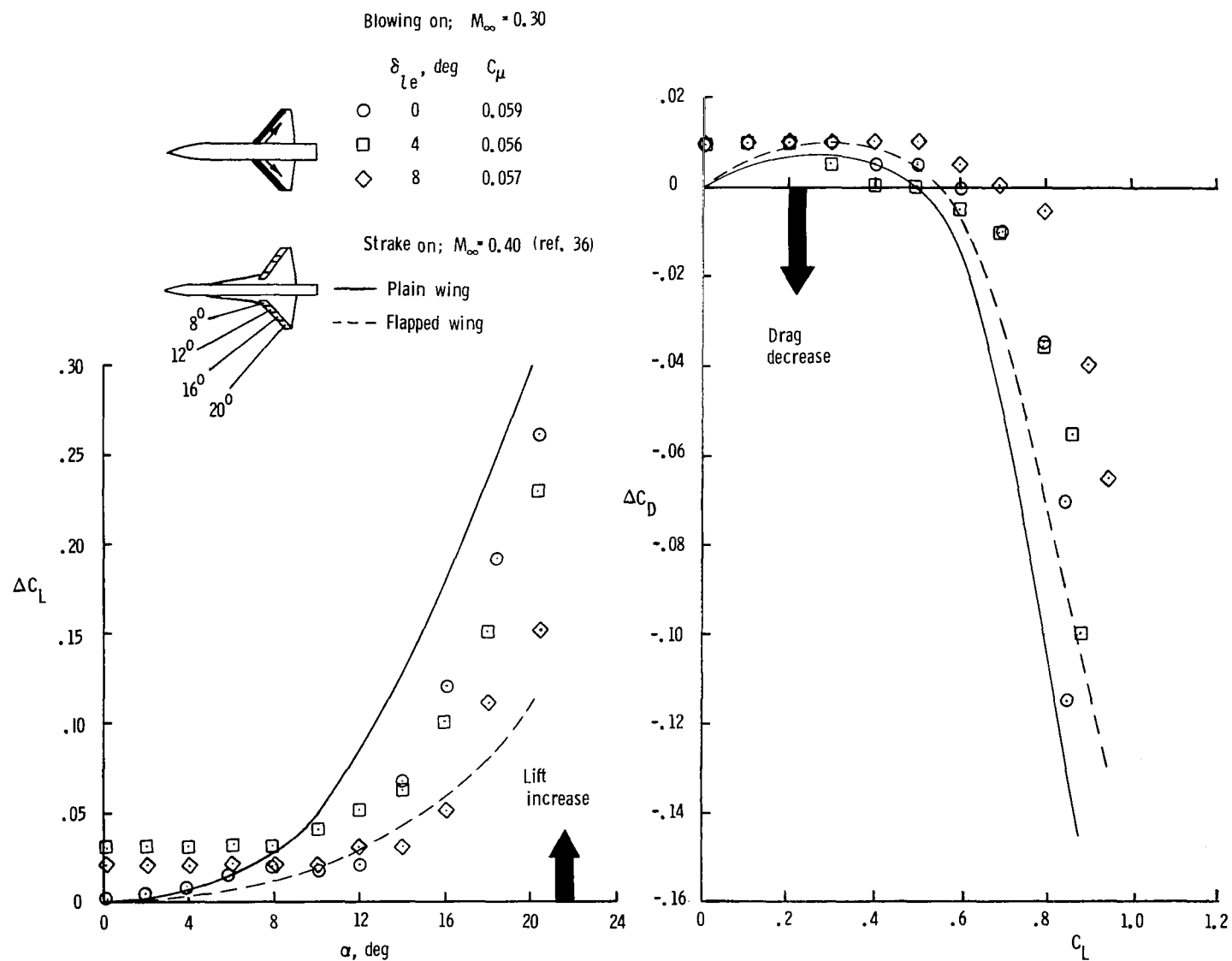
Figure 19.- Effect of leading-edge flap deflection on lift and drag increments due to wing stroke or spanwise blowing.
