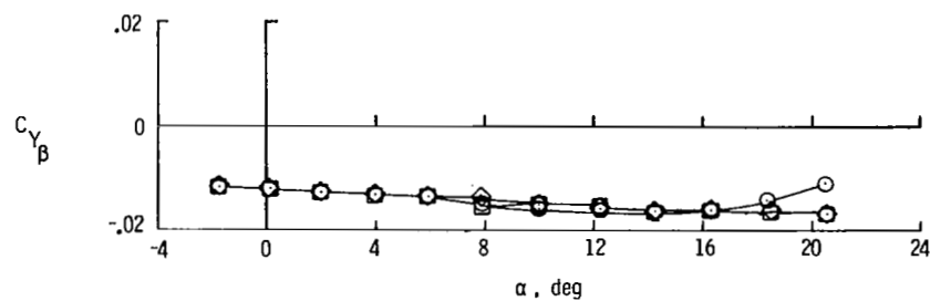
Figure 27.- Effect of spanwise blowing on lateral-directional stability derivatives of configuration with wing and vertical tail; M_\infty = 0.30 .
