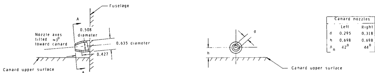
(b) Canard nozzle.
