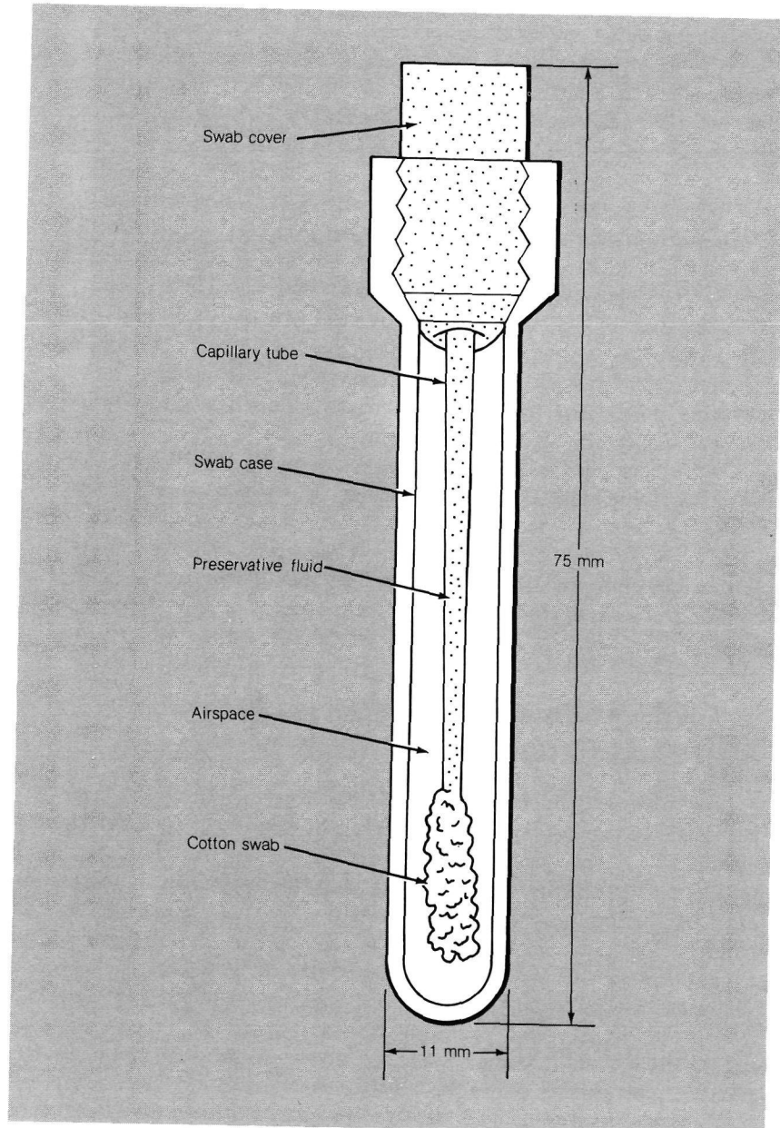
Figure 5.1 The AR-002 swab. Eighty of these swabs were carried on Apollo-Soyuz. Each swab was sealed in a plastic tube before and after use. Preservative fluid in the stem of the swab kept the microbes on the swab alive.
