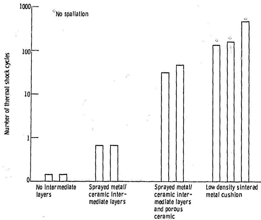
Figure 4. - Number of thermal shock cycles required to cause spallation of material for several turbine seal concepts evaluated.
