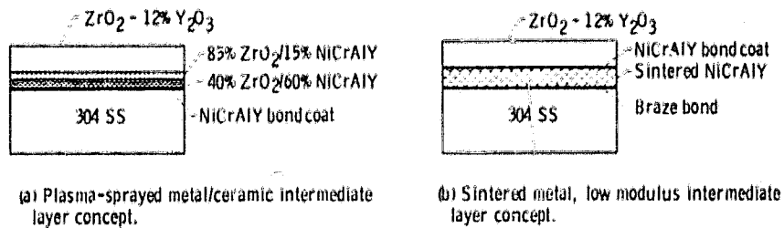
Figure 1. - Schematic representation of the two major turbine seal concepts evaluated.
