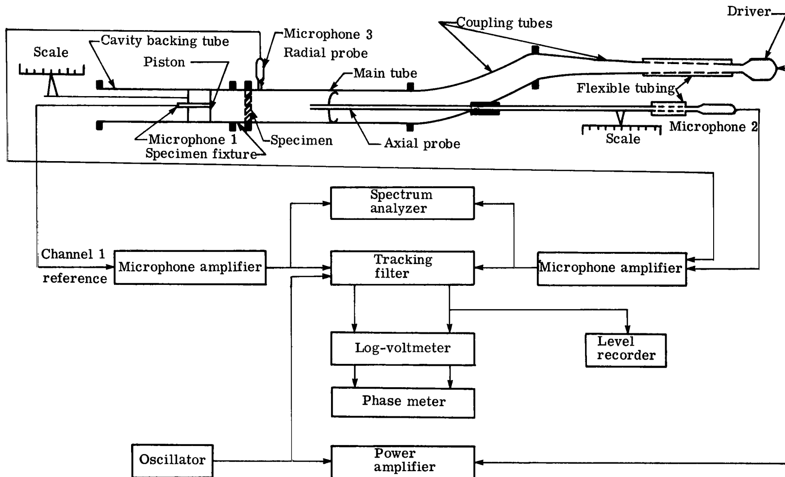
Figure 17.- Block diagram of experimental setup.
