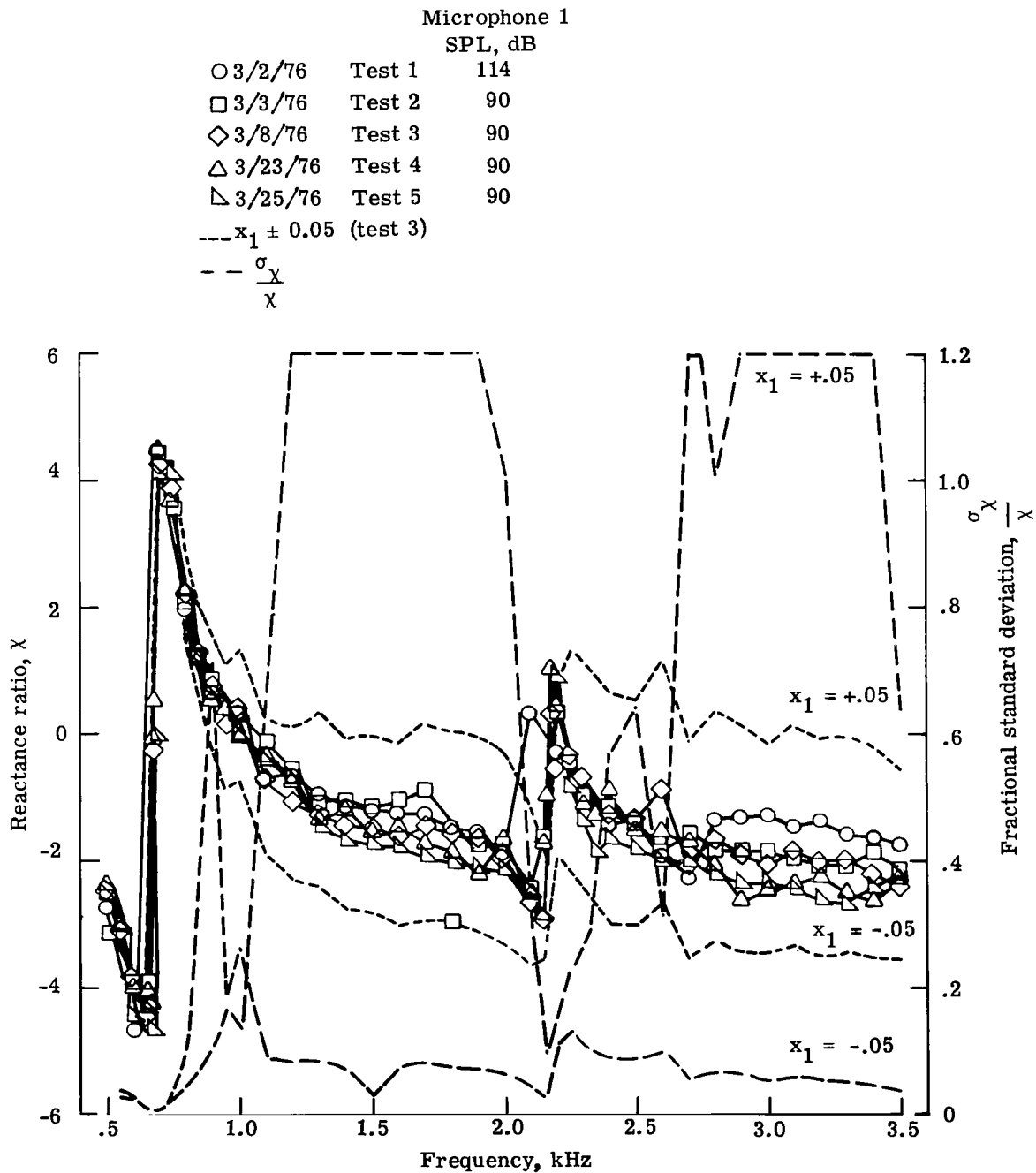
Figure 26.- Reactance ratio plotted against frequency for specimen C.
