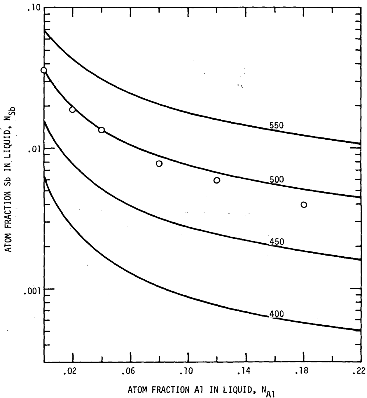
Fig. 3.3 AlGaSb liquidus isotherms
