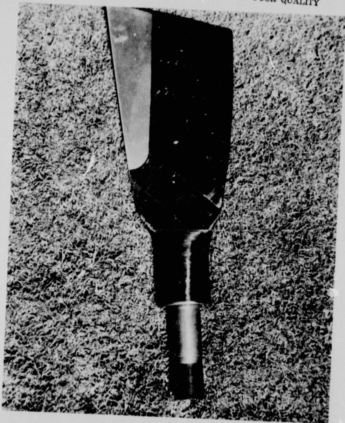
FIGURE 1. FILAMENT-WOUND SPAR SHELL FAN BLADE
