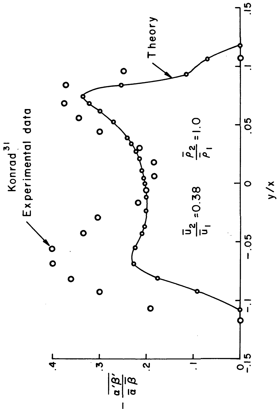
Figure 9. Profile of the unmixedness correlation \left(-\frac{\overline{\alpha'\beta'}}{\overline{\alpha}\overline{\beta}}\right) in a shear layer.
