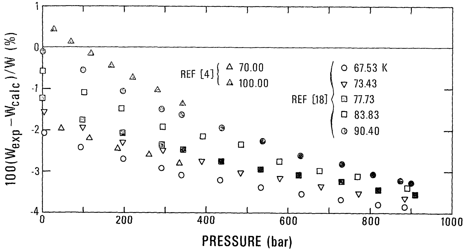
Figure 6. Comparison with experimental sound velocities in the compressed liquid.
