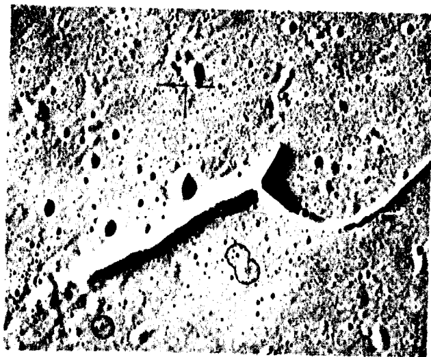
FIGURE 15-18. Comparison of "dot-shaped" vents on the Moon and Earth. Figure on left is part of a suspected vent and associated channel near the crater Delisle on the Moon (Apollo 15 frame AS15-2073); middle photograph is a view of the summit vent of Mauna Ulu in Hawaii; right photograph is an oblique aerial view of an elongate vent southeast of Big Southern Butte on the Snake River Plain. Lunar feature is about ten times larger than the terrestrial features.
