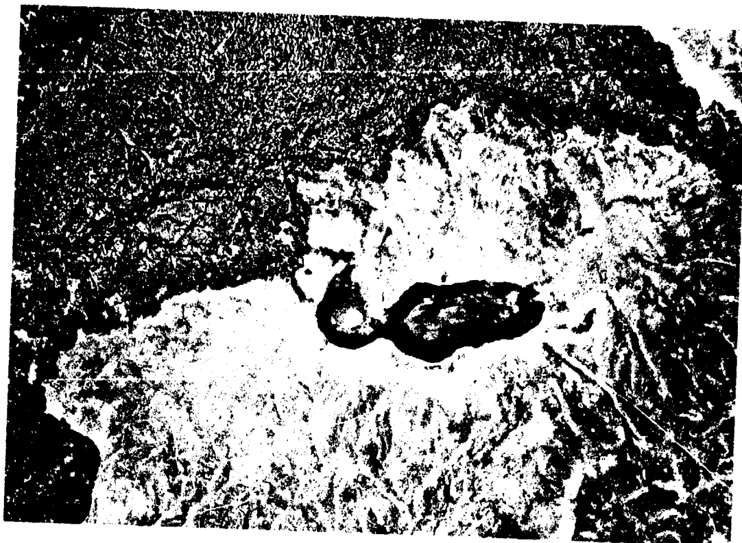
FIGURE 5-41. Aerial photograph of area 10 km SSE of Carey, showing variation in pahoehoe surface textures on the 1 to 5 m scale and circular collapse depressions. (North is to the right.) Area of photograph is 2.0 km by 1.3 km. (U. S. Geological Survey Photograph GS SWEZ 6-80, September, 1971.)
