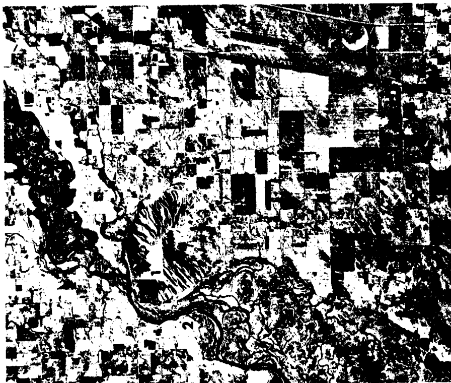
FIGURE 17-1. Landsat (ERTS) photograph of the eastern Snake River Plain. Hell's Half Acre flow (1), Snake River (2), American Falls reservoir (3), East and Middle Buttes (4), Big Southern Butte (5), Cerro Grande lava field (6), Wapi flow and King's Bowl Rift (7), Craters of the Moon lava field (8), Lost River Range (9). Arrows indicate trend of the Great Rift system. Area shown is 136 km by 142 km.
