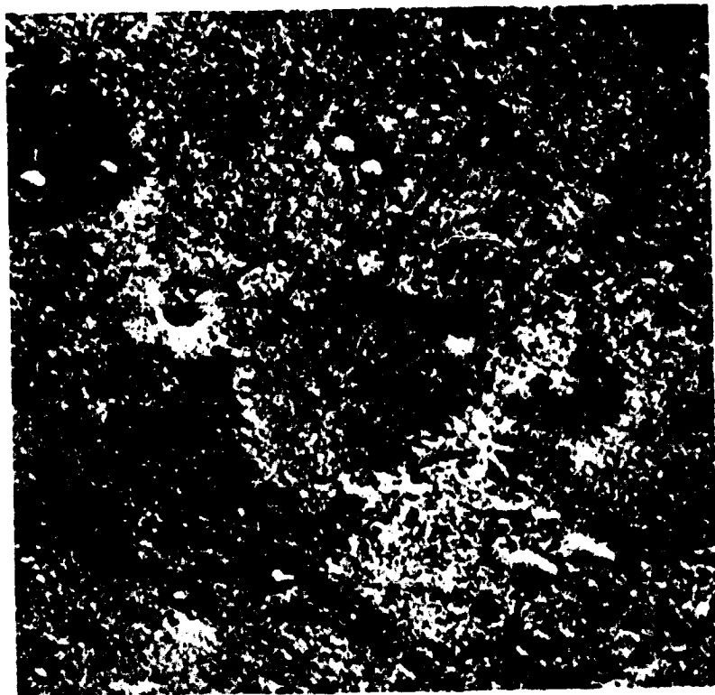
FIGURE 15-2. Low shield (arrow) about 4.2 km long in southeastern Chryse Planitia; a small "knob" several hundred km across occurs on the southern end of the low shield. (Viking Orbiter I frame 6A36.)
