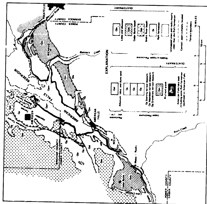
FIGURE 18-16. Geologic sketch map along the Snake River in the American Falls area. (After Trimble and Carr, 1961.)
