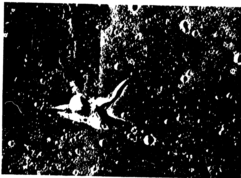
FIGURE 15-19. Comparison of Aratus CA in western Mare Serenitatis on the Moon (right photograph) with Bear Crater on the Snake River Plain. Area of lunar photograph is about 17 km by 25 km; terrestrial photograph is about 2.5 km by 3.3 km. Both features are vents for basaltic lavas (after Greeley, 1973).
