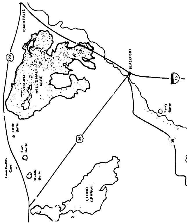
FIGURE 7-1. Index map to Hell's Half Acre lava field.
