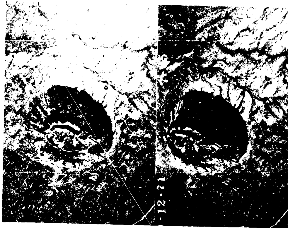
FIGURE 6-6b. Stereoscopic pair of aerial photographs (turn page 90° for viewing) of Middle Butte. (U. S. Geological Survey photograph GS-SWFZ 7-85, 86; October, 1971).
