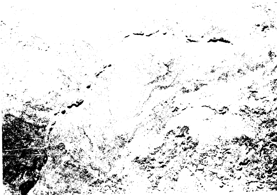
FIGURE 5-36. Vertical aerial photograph of the western end of Bear Trap lava tube; area of photograph 1.8 km by 2.7 km. (U. S. Geological Survey Photograph GS-SW12-8-19, October, 1971.)
