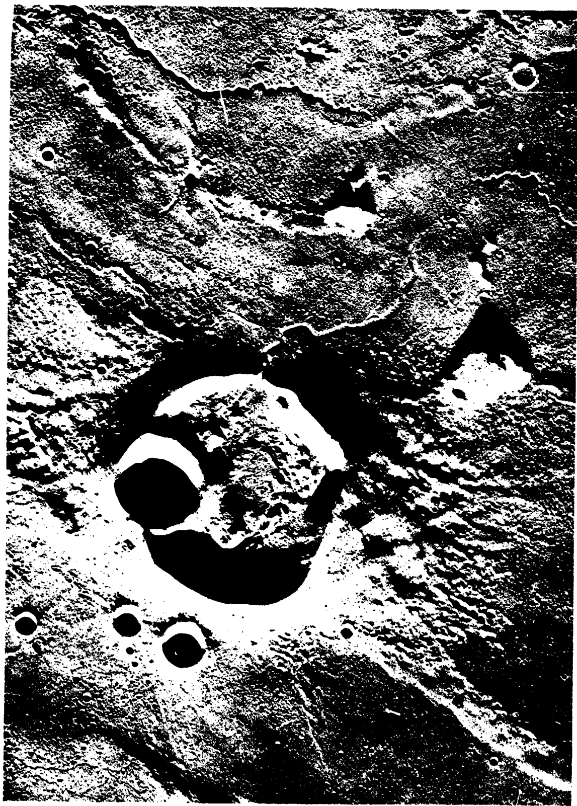
FIGURE 15-13. Apollo 15 photograph of the lunar crater Krieger showing a sinuous rille and probable associated flows that overlap an older sinuous rille on the right side of photograph. Lack of discernible flow margins suggest extremely thin flow units associated with the rille. Area of photograph is 40 km by 50 km; north is to the bottom. (Apollo 15 metric frame 2082.)
