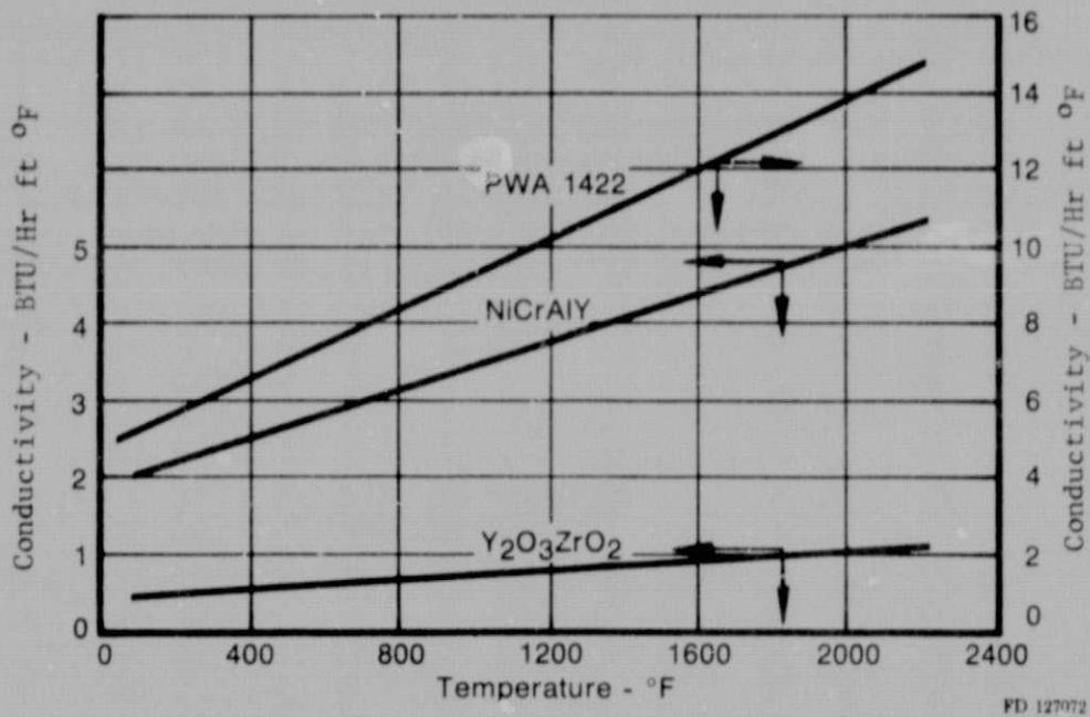
Figure A-1. Thermal Conductivity
