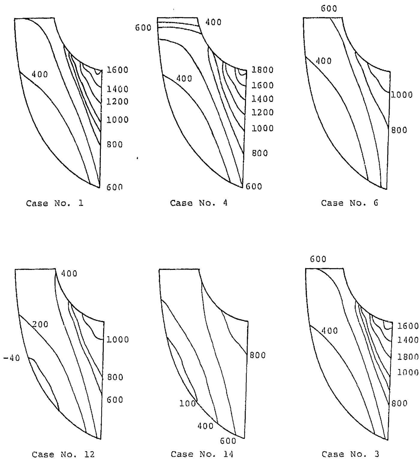
FIG. 5. MERIDIONAL VELOCITY DISTRIBUTION (FT/SEC)
