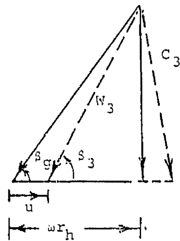
FIGURE 18B. EFFECT OF SWIRL VELOCITY NEAR HUB.
