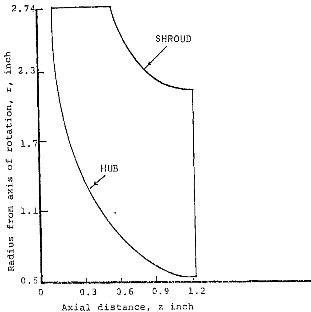
FIGURE 3A. MERIDIONAL VIEW OF THE ROTOP.
