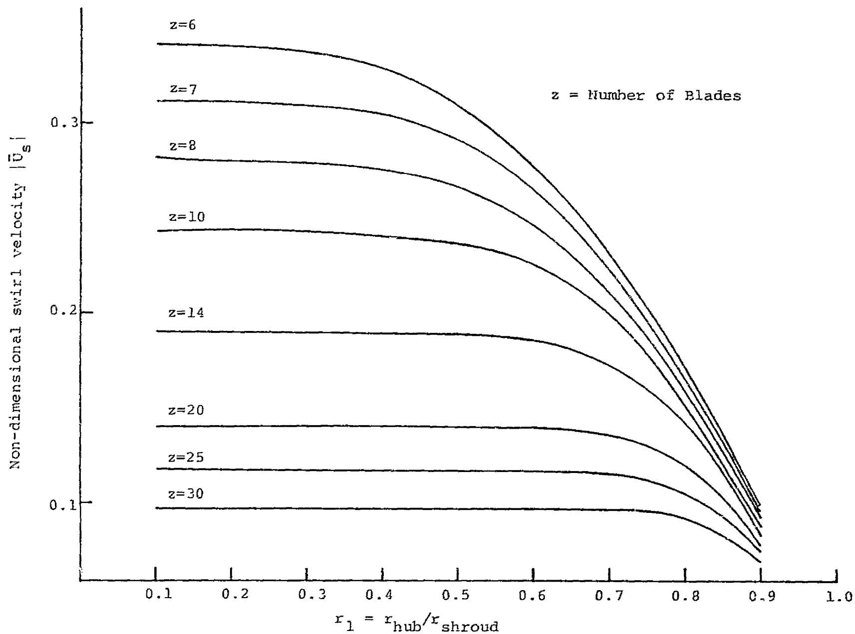
FIG. 20. EFFECT OF DESIGN VARIABLES UPON SWIRL VELOCITY NEAR SHOUD.
