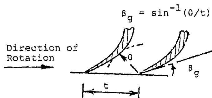
FIGURE 17A. GEOMETRIC BLADE EXIT ANGLE.
