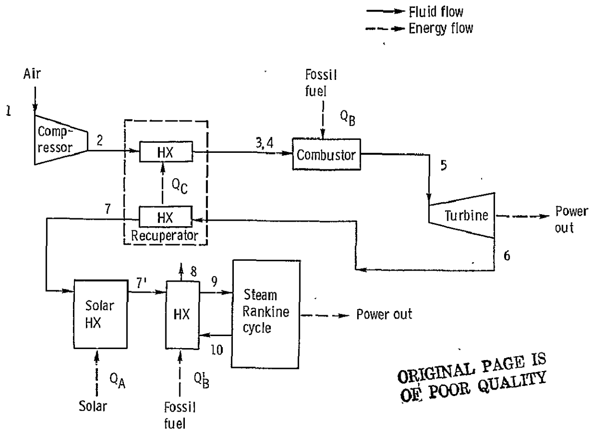
Figure 13. - Diagram of supplemental-fired combined cycle hybrid system.
