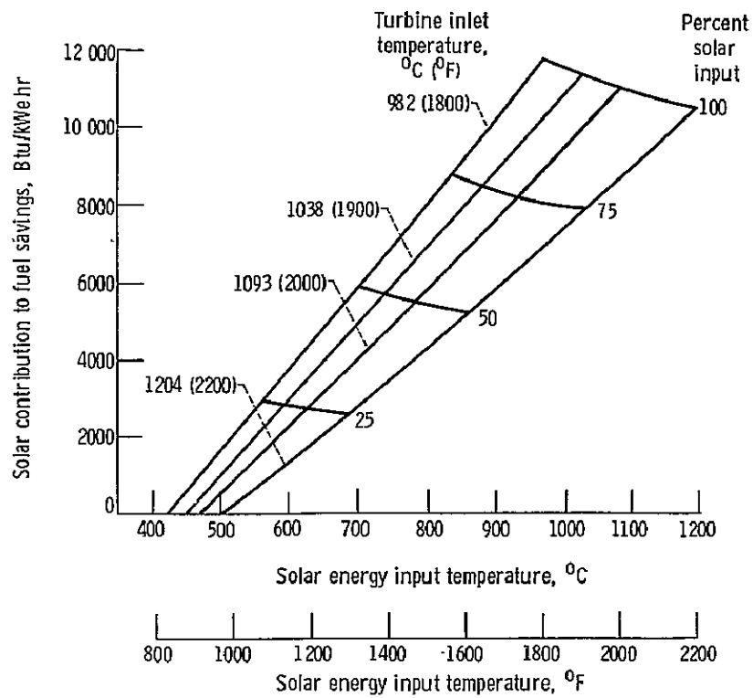
Figure 7. - Solar fuel savings for optimized simple gas turbine open cycle hybrids.
