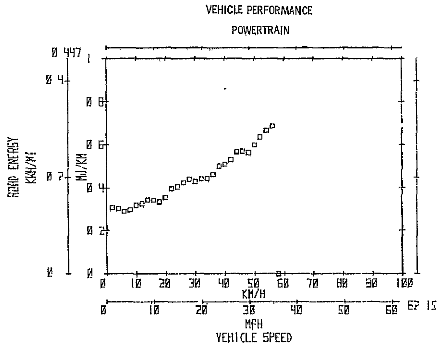
(a) With regenerative braking, July 20, 1977.
