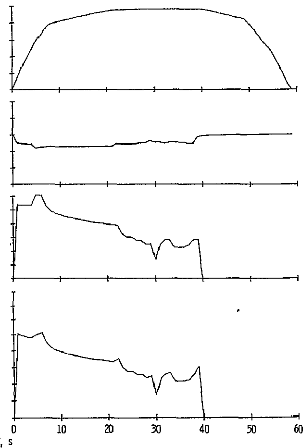
(h) Schedule C with regenerative braking, cycle 84, June 29, 1977.
