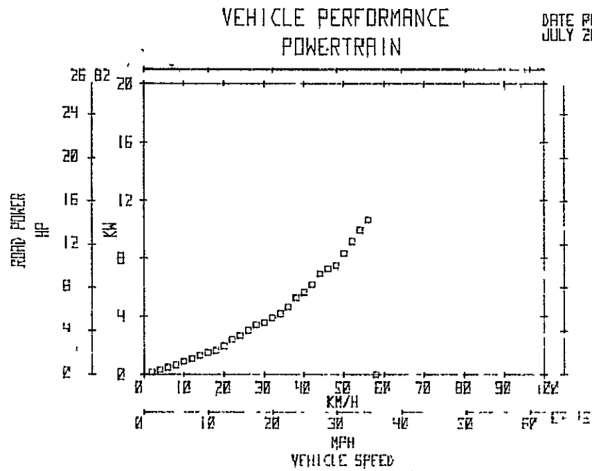
(a) With regenerative braking, July 20, 1977.
