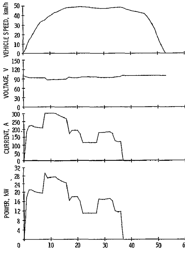
(g) Schedule C with regenerative braking, cycle 4, June 29, 1977
