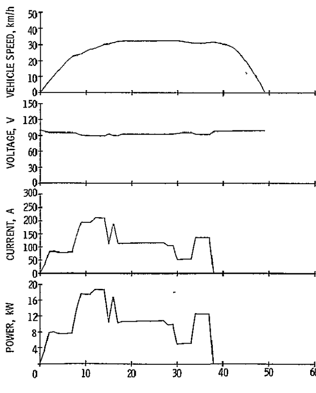
Figure 18 - Battery output as a function of time
