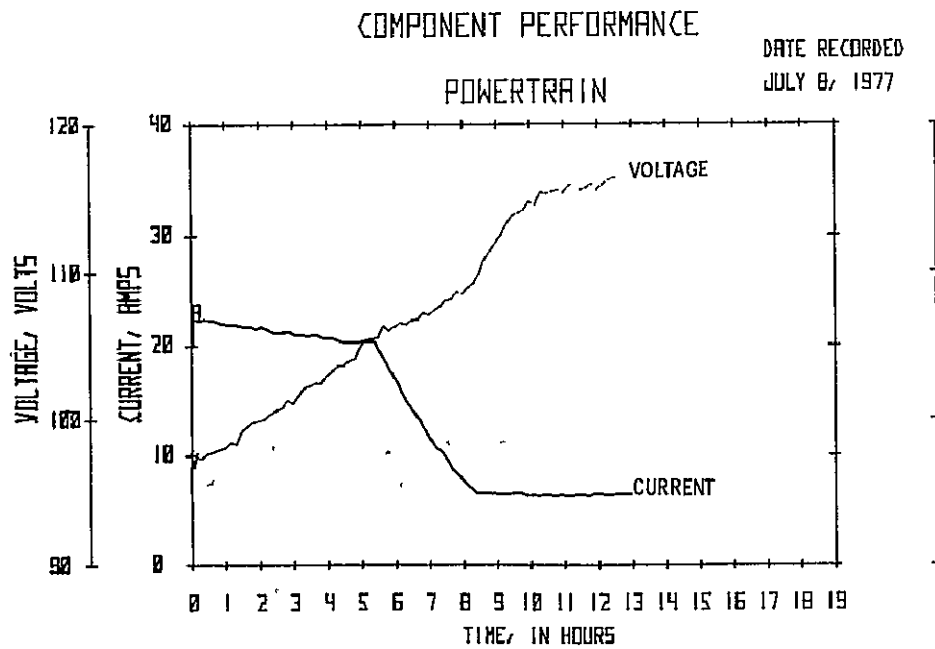
Figure 12 - Battery charger output voltage and current
