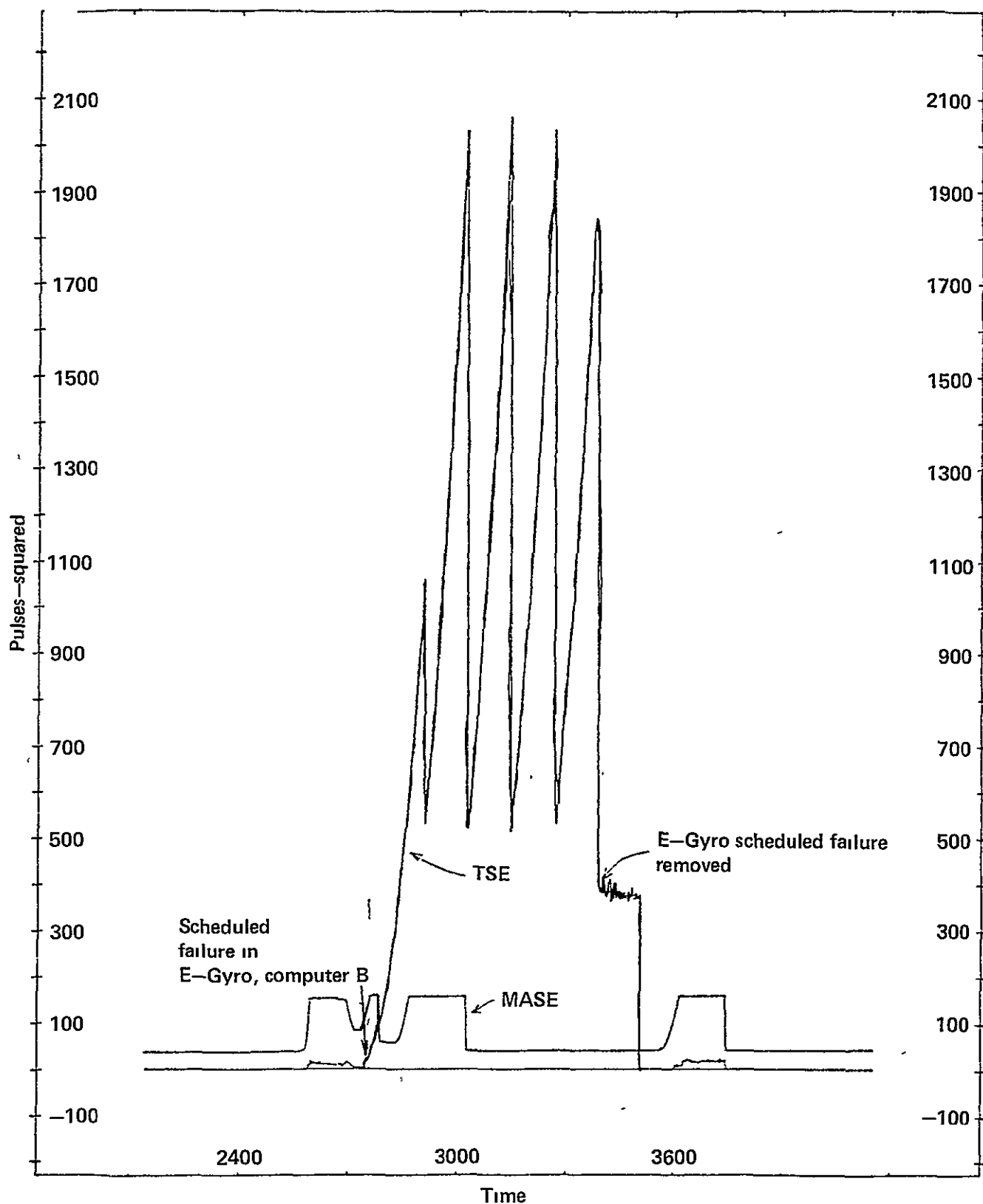
Figure 23.- Maximum allowable squared error (MASE) and total squared error (TSE) for gyros vs time, failure test computer (B), flight 9/05C.
