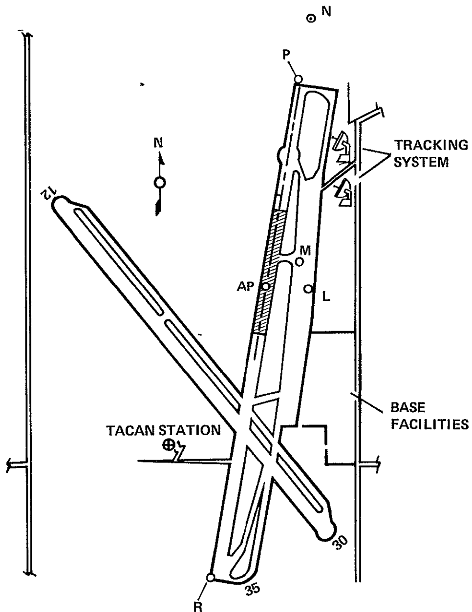
Figure 14.- Benchmark locations at Crows Landing.
