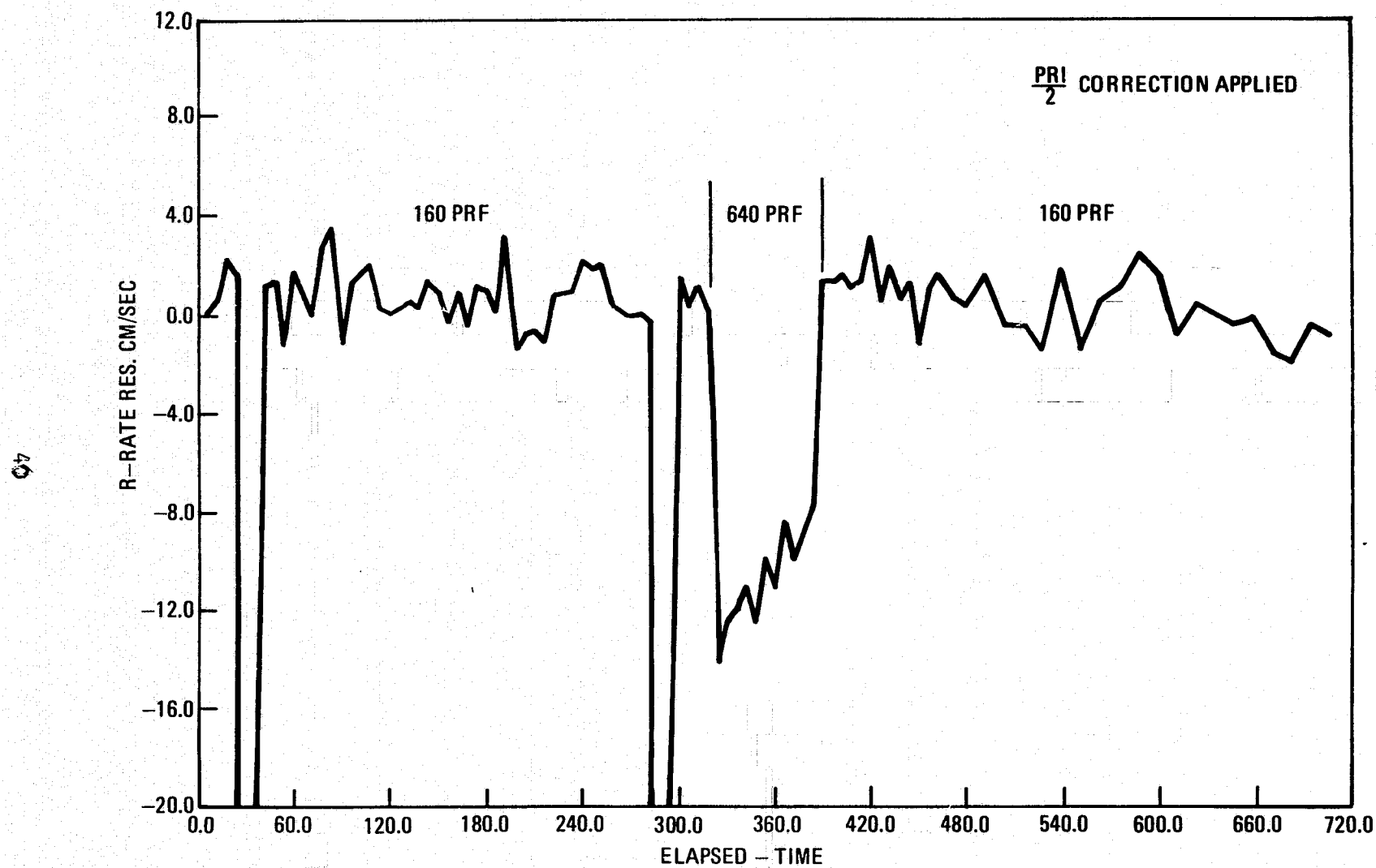
Figure 11. - Range rate residual error GEOS-3, Rev 498
