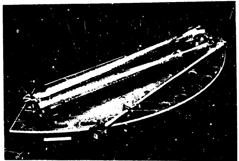
Figure 2. Magnetometer Deployment Mechanism with Thermal Control Finishes
