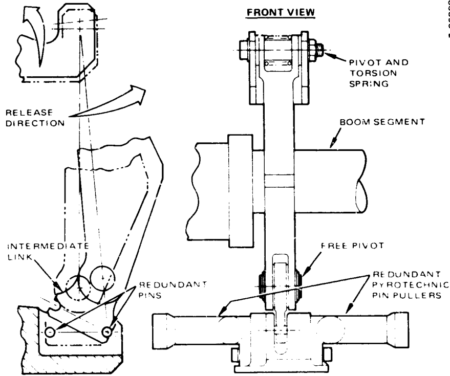
FIGURE 6. REDUNDANT PIN PULLERS
