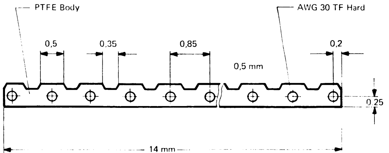
Fig. 3 Flexlead Cable Cross Section
